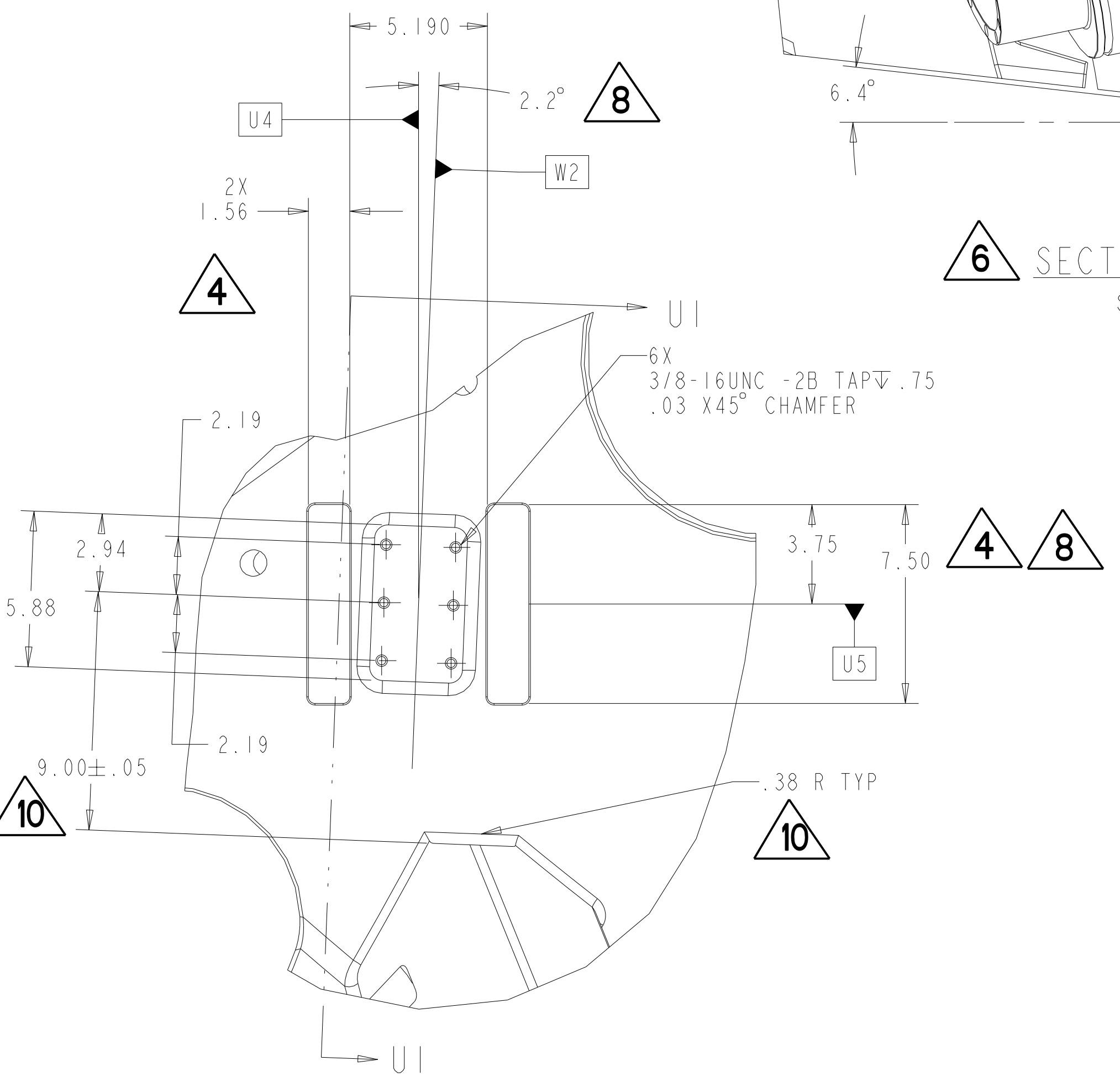
VIEW D4 - D4 SCALE 0.250
