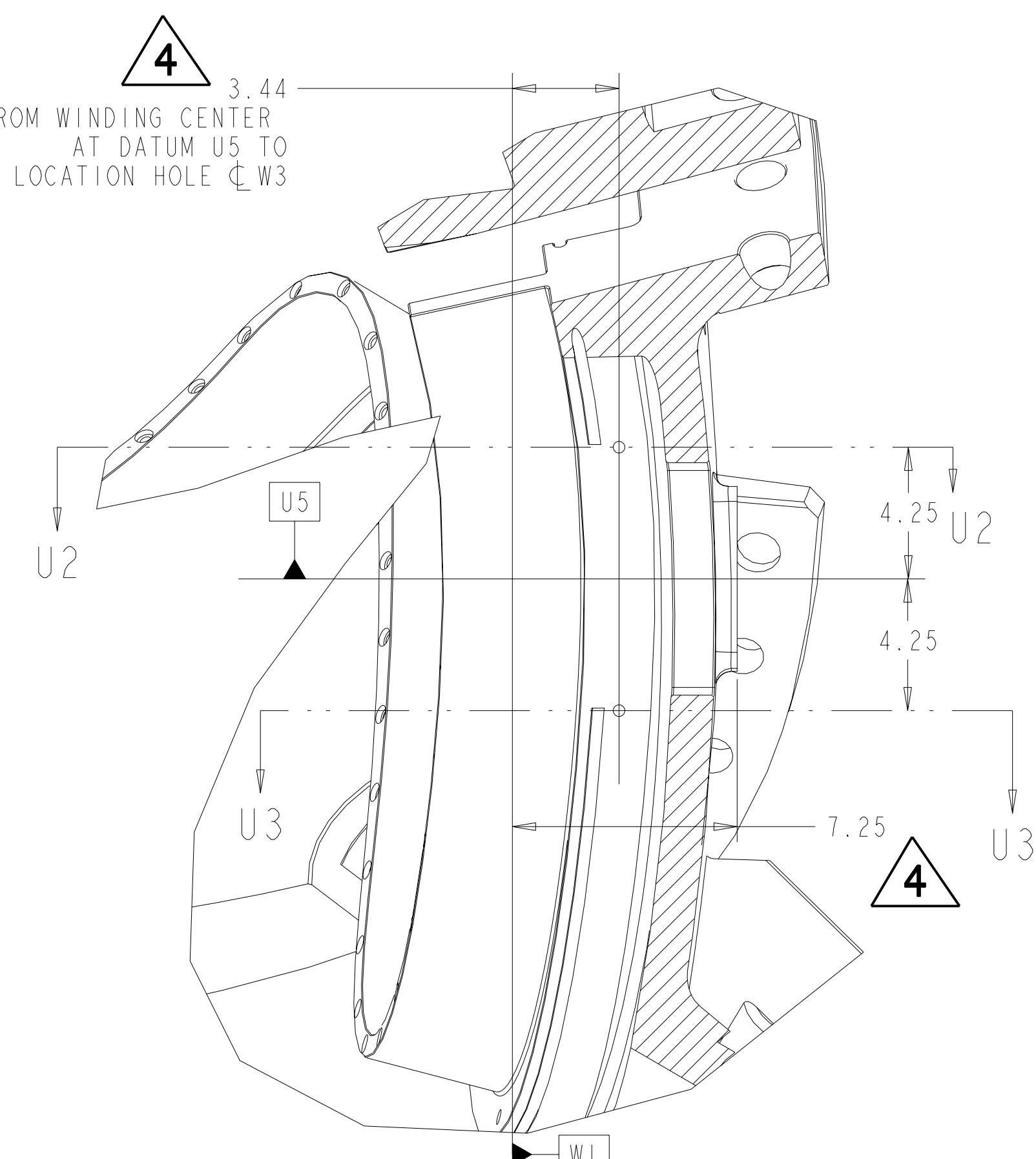
SECTION U1-U1 3 5 4
