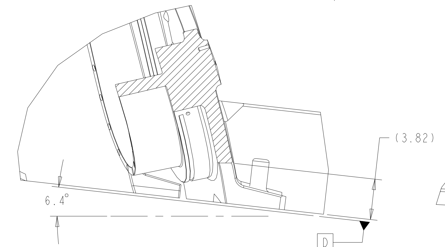
6 SECTION D3-D3 SCALE 0.19
