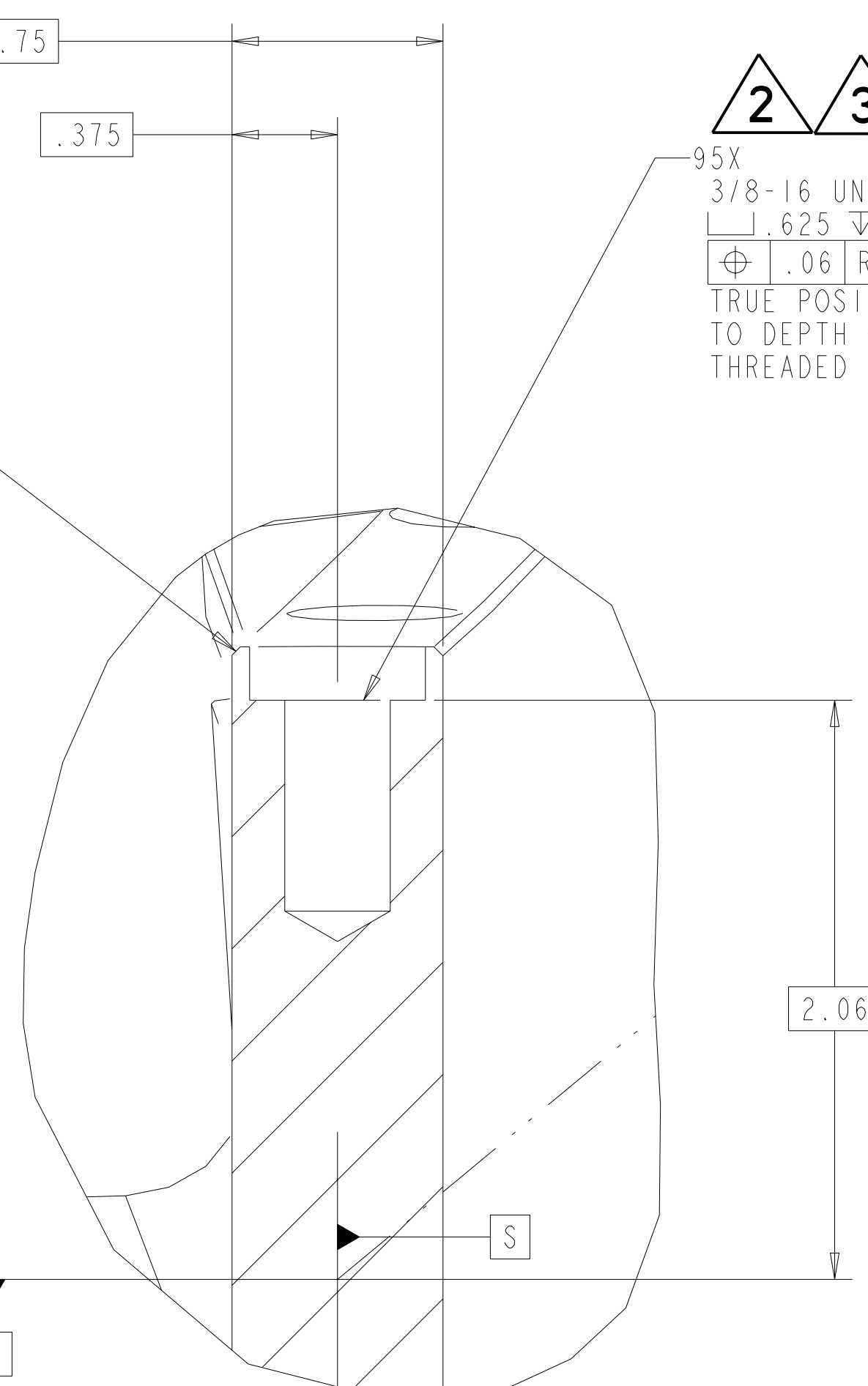
DETAIL C SCALE 2.00
