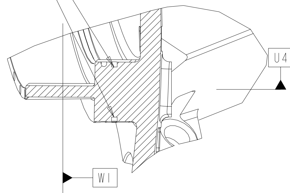
SECTION U2-U2 3 5
