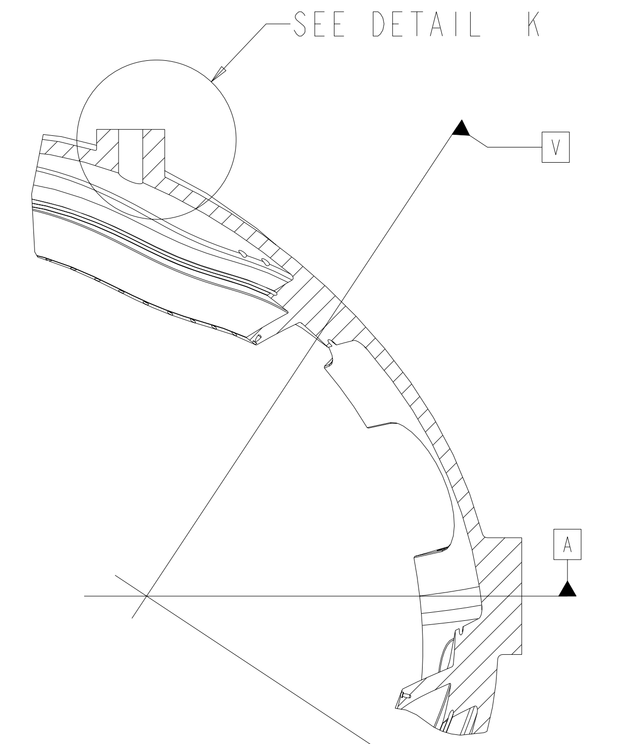
SECTION H-H VESSEL VERTICAL SUPPORT SCALE 0.10
