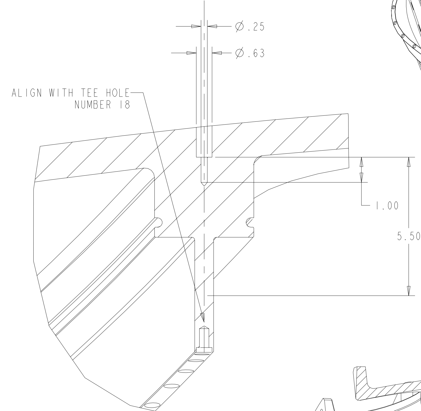
DETAIL D SCALE 0.50
