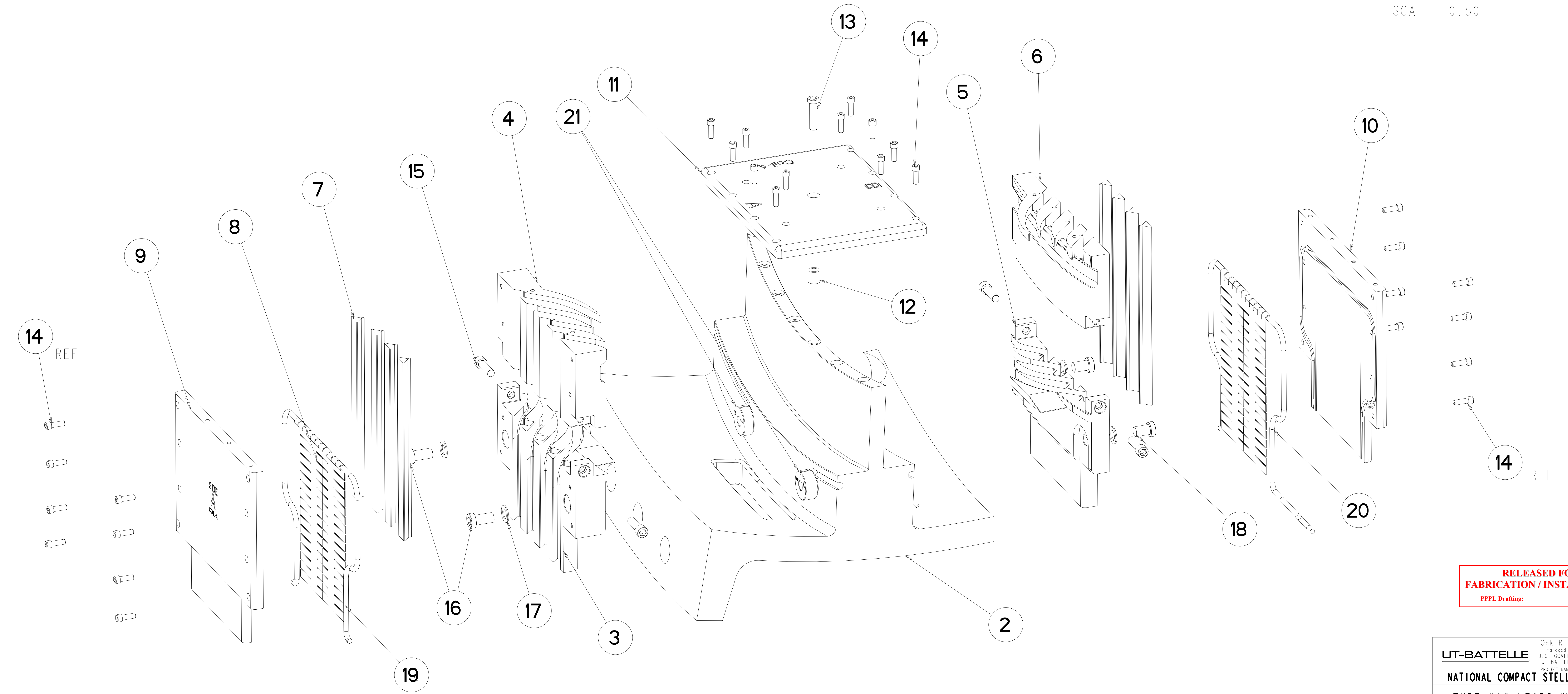
EXPLODED VIEW
