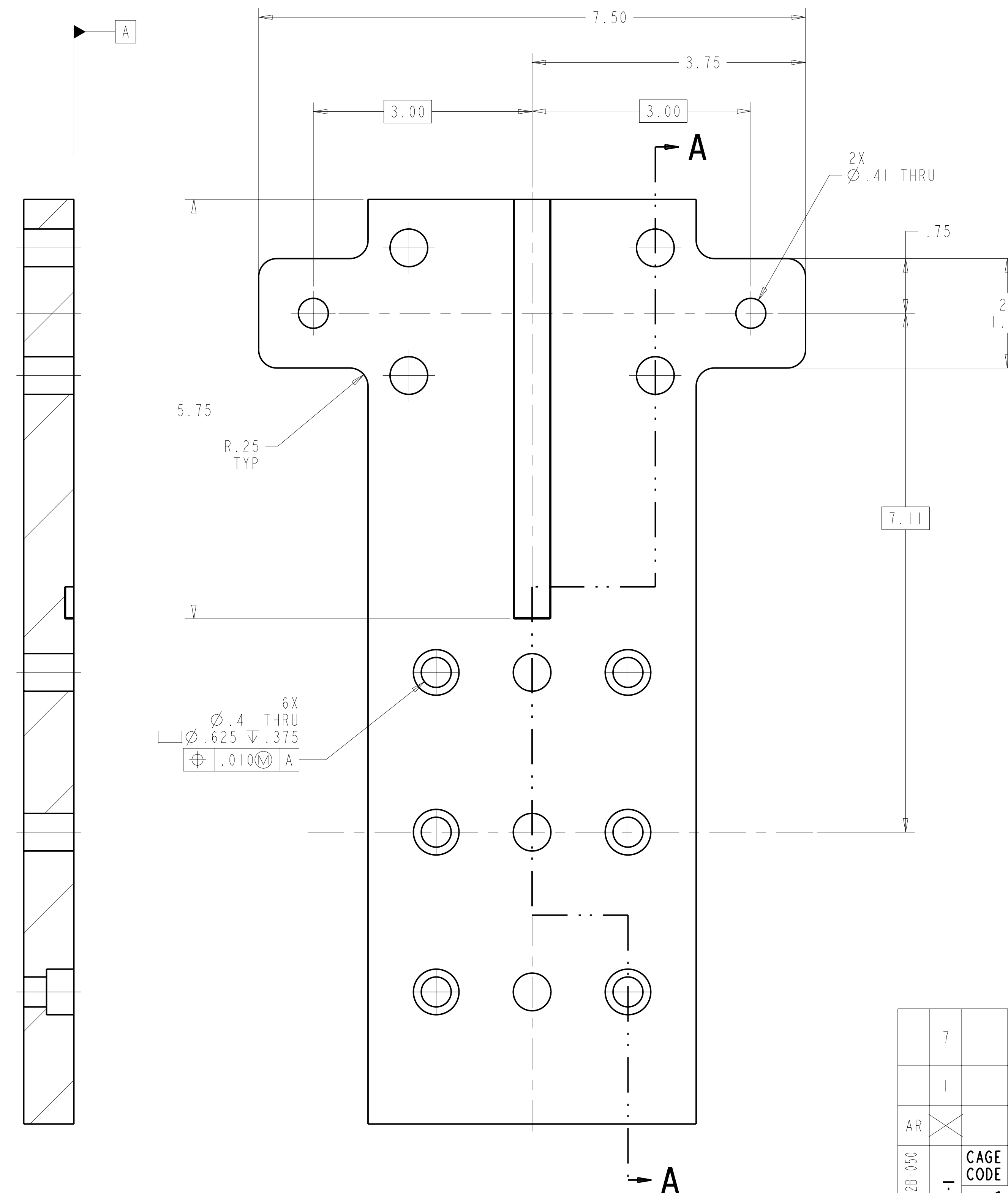
1 TOP VIEW
