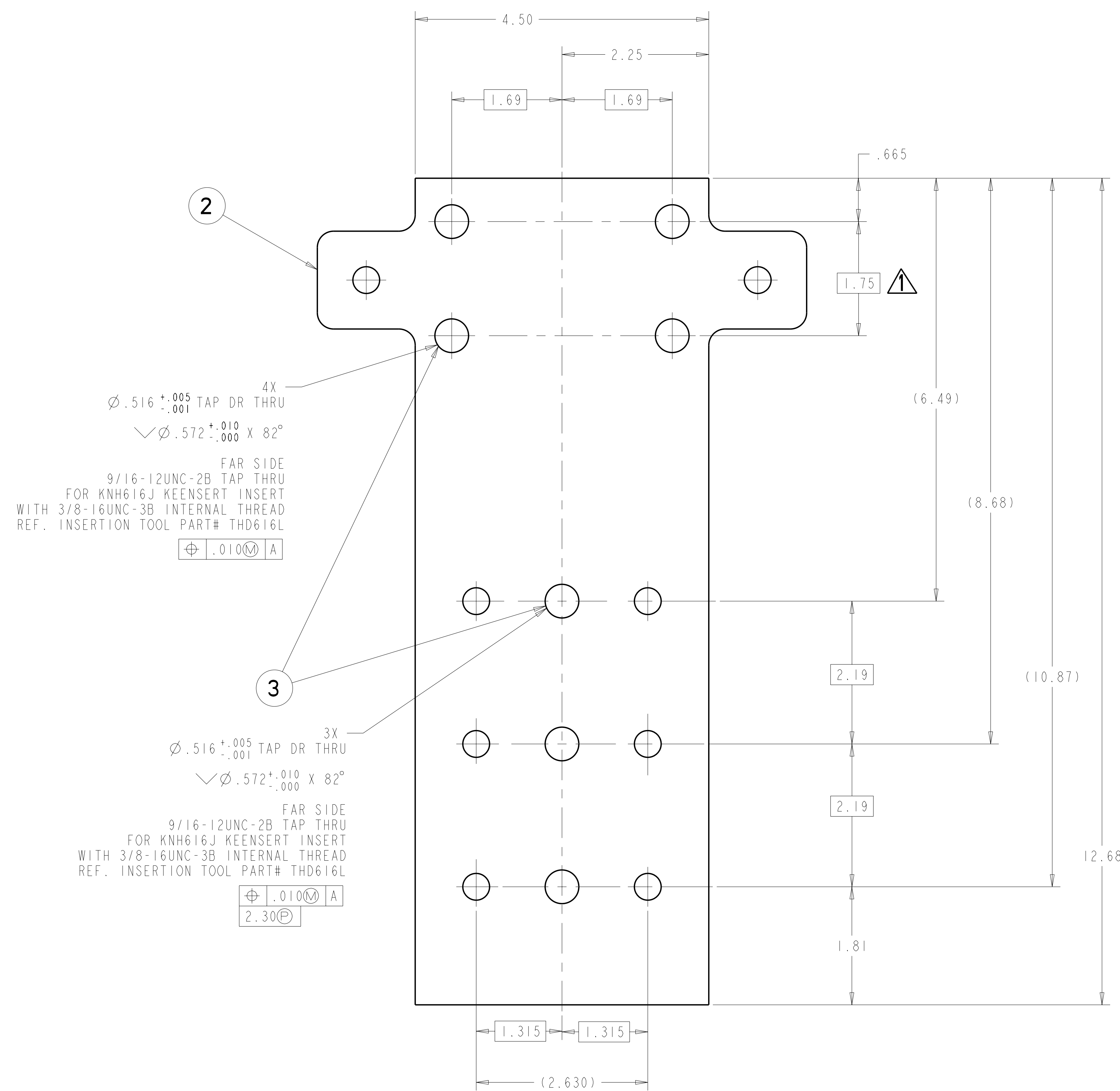
BOTTOM VIEW
