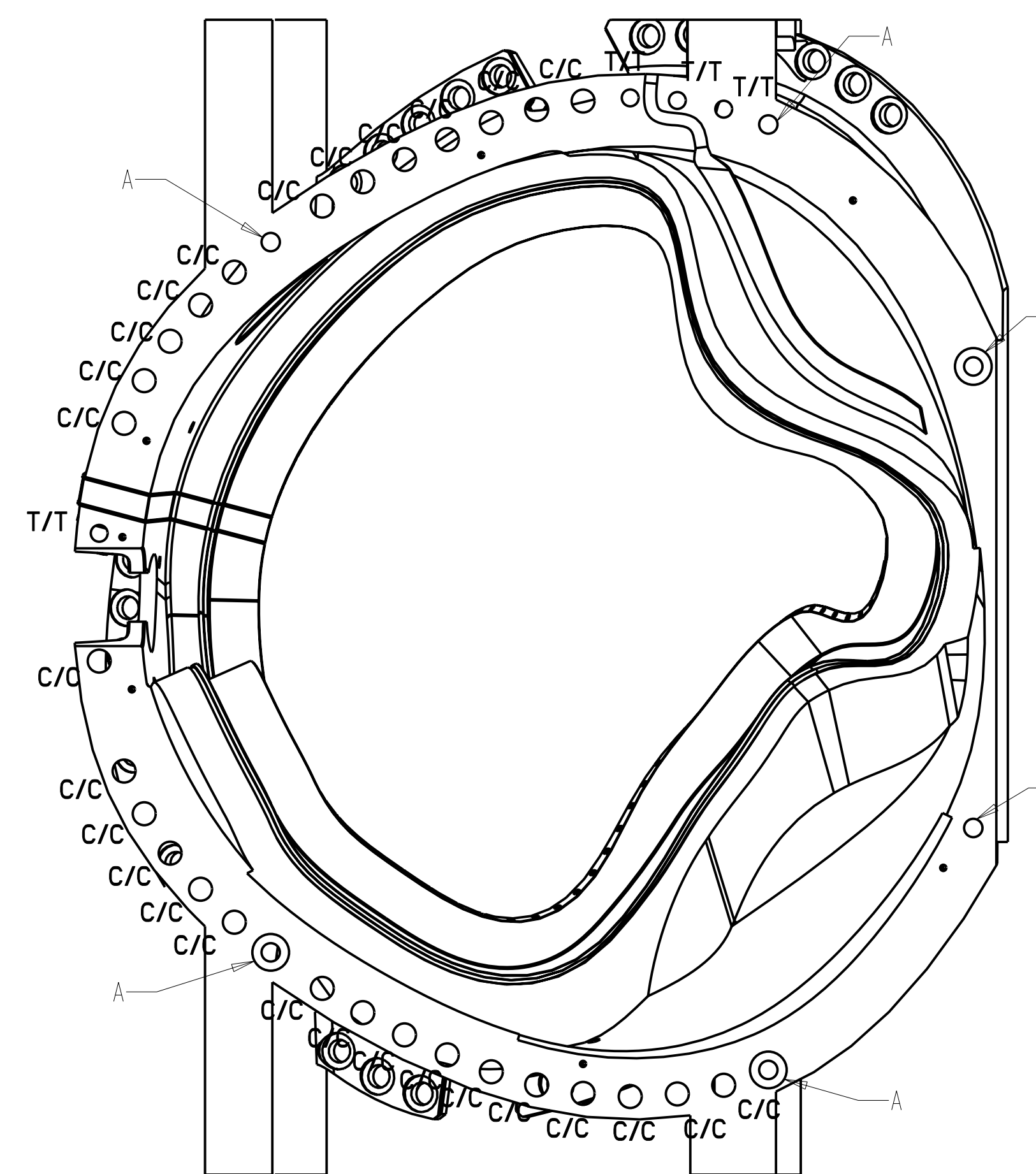
TYPE-C DATUM-E (WINDING SIDE-B)
