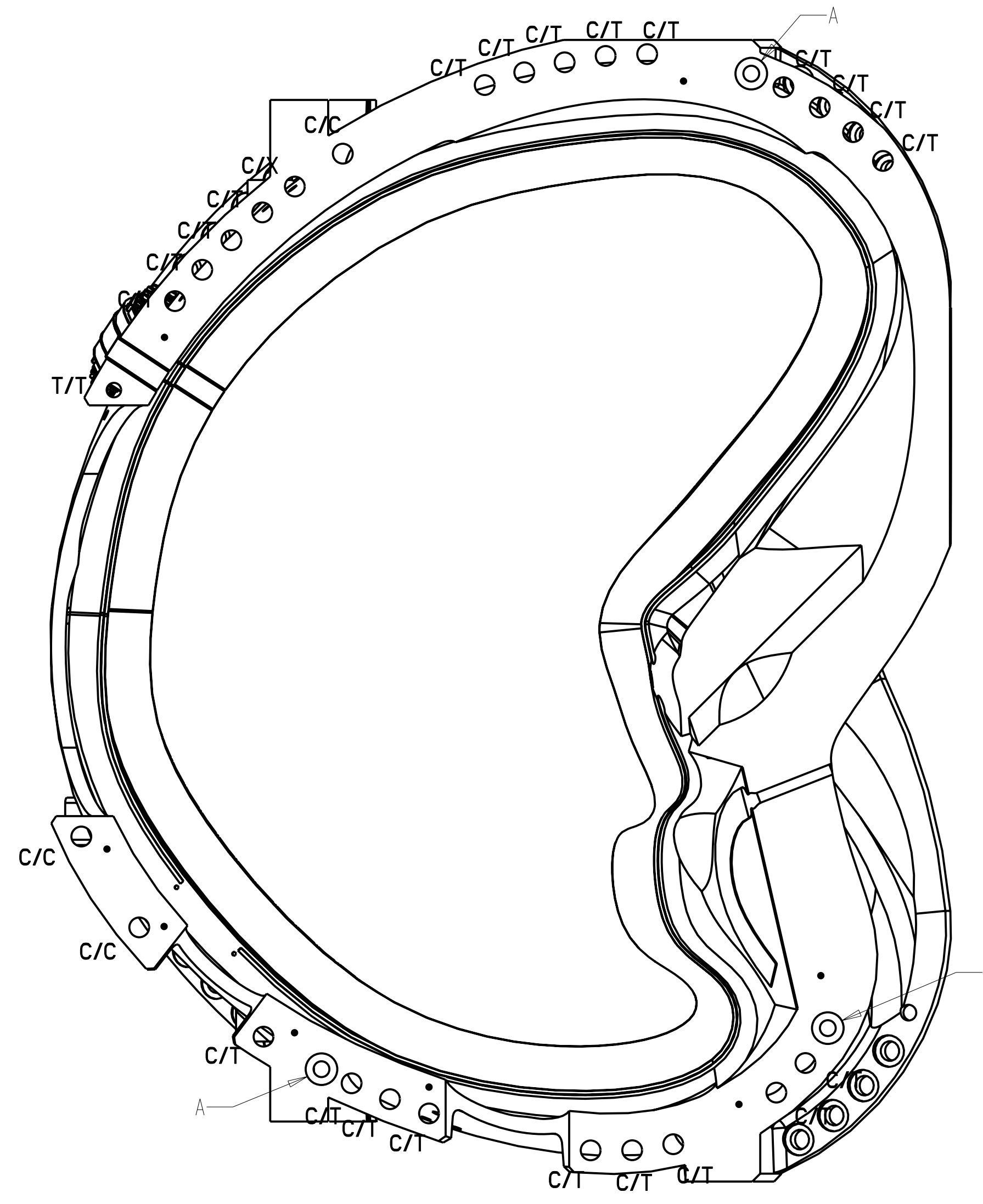
TYPE-A DATUM-E (WINDING SIDE-B)
