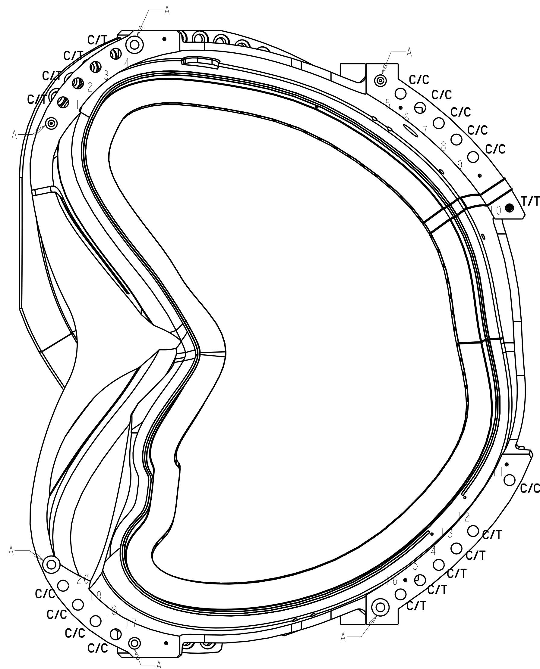
TYPE-A DATUM-D (WINDING SIDE-A)
