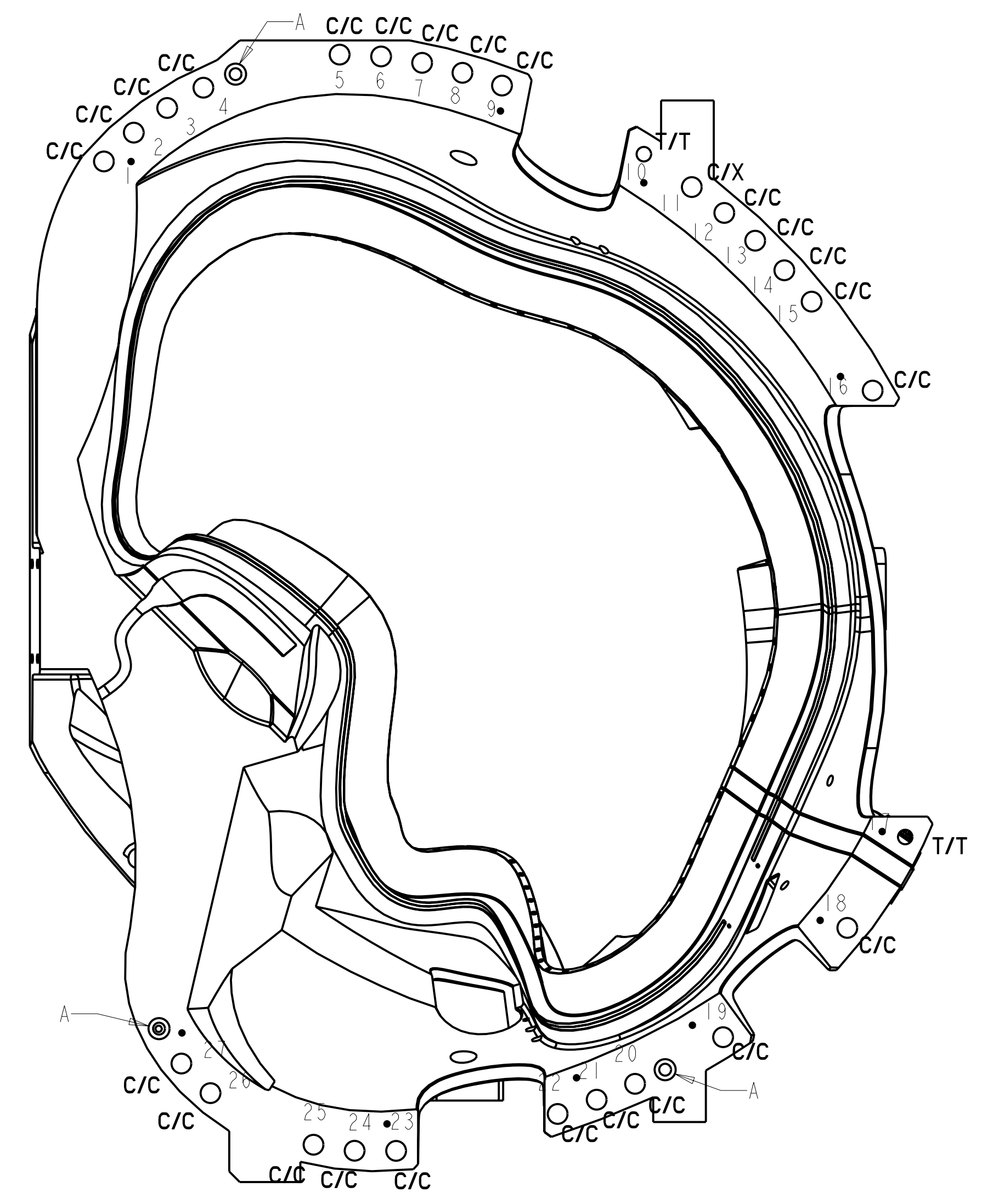
TYPE-B DATUM-D (WINDING SIDE-A)
