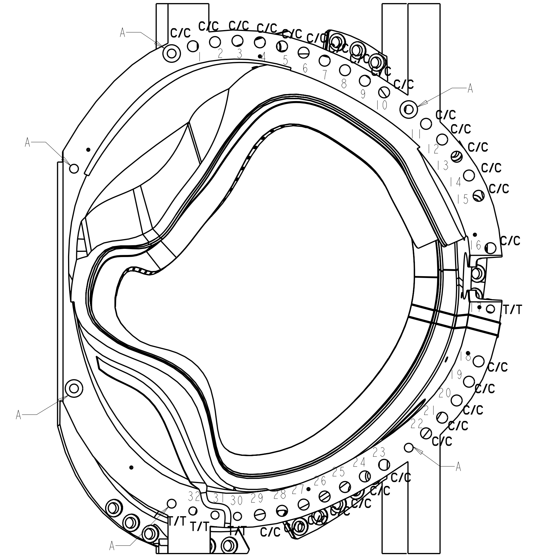
TYPE-C DATUM-E (WINDING SIDE-B)
