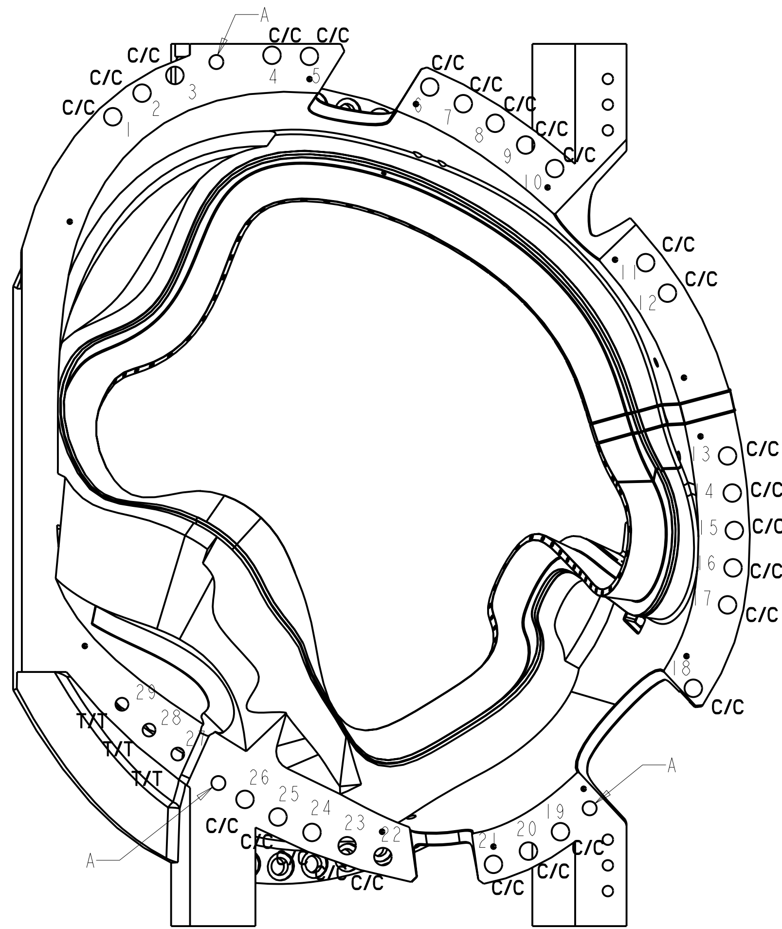
TYPE-C DATUM-D (WINDING SIDE-A)
