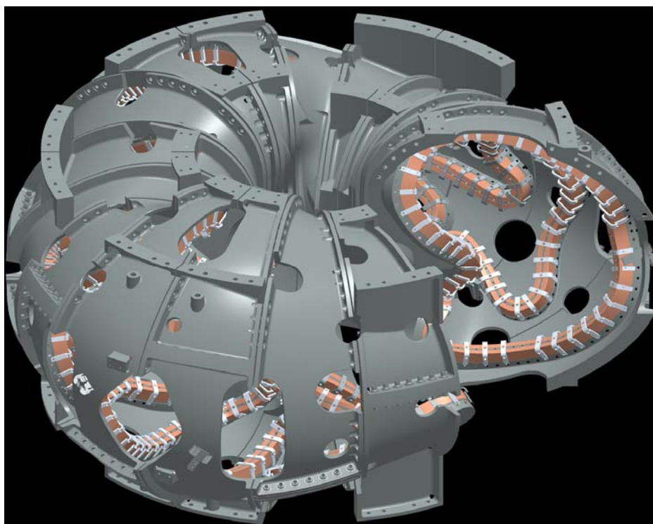
Figure 9: Modular coil assembly.
