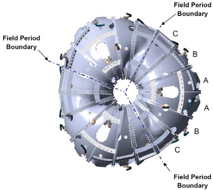
Figure 10: Top view of the modular coil form assembly
