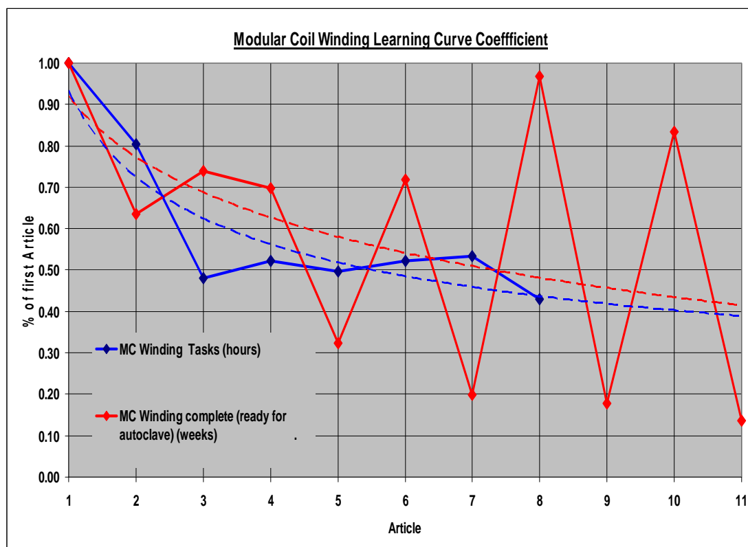
Figure 16: Learning curve for modular coil winding: time intervals between completion successive coils normalized to the time interval between the first and second articles.
