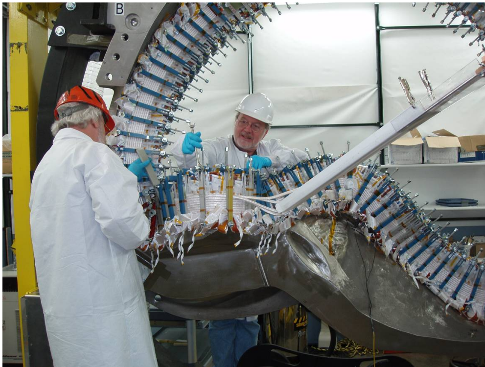
Figure 12: Modular coil winding operations at PPPL.
