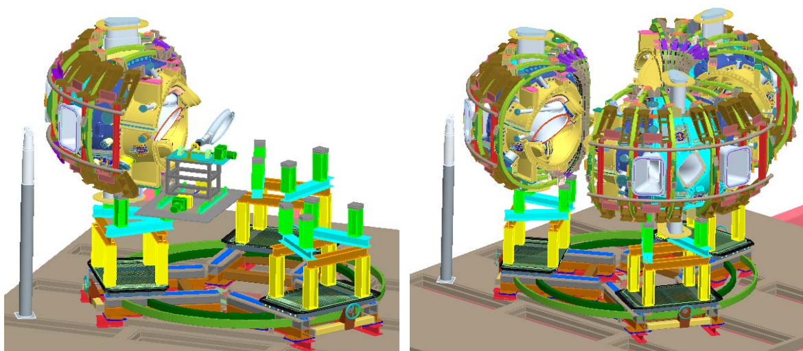
Figure 25: Schematics illustrating base structure, retractable FPA carts, and machine assembly.
