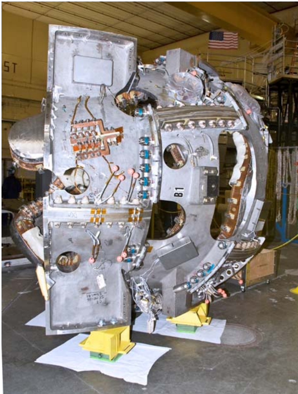
Figure 23: Assembled half field period.
