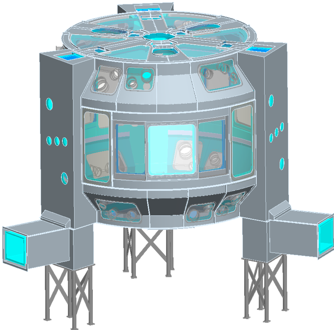
Figure 20: Conceptual schematic of the NCSX cryostat.
