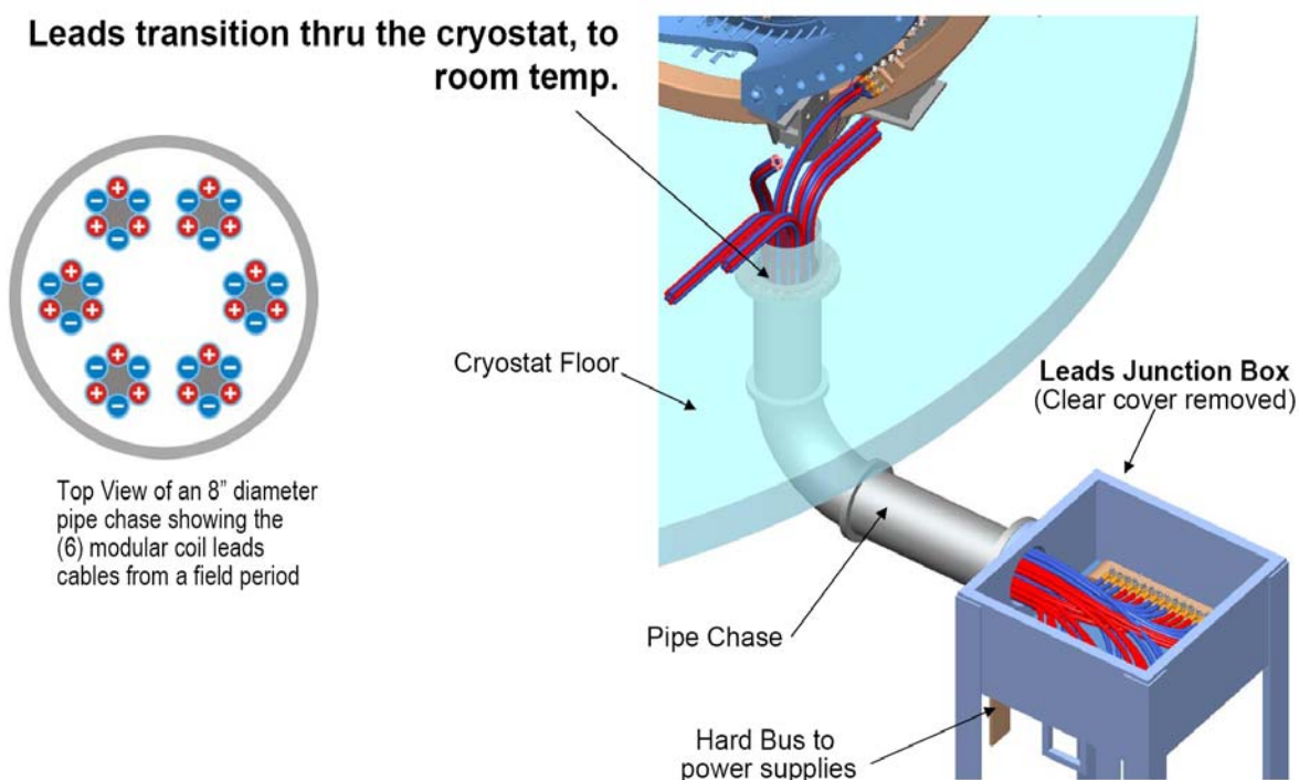
Figure 19: Schematic illustrating coil electric power distribution
