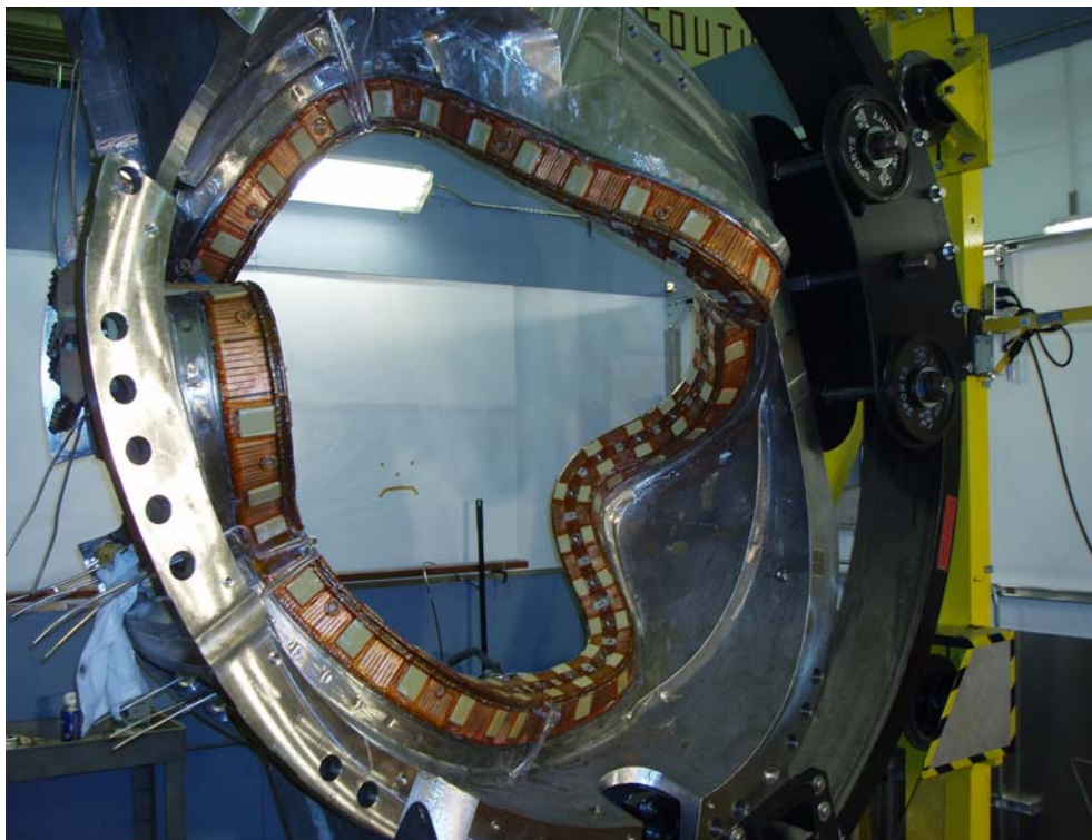
Figure 13: Modular coil after vacuum-pressure impregnation (VPI).
