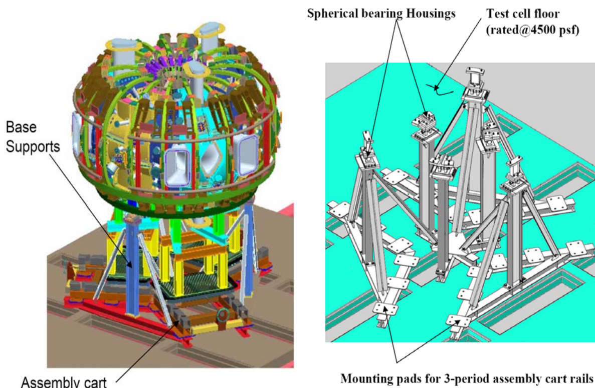
Figure 21: Base supports design; assembly cart (WBS 18) also shown in illustration on left.
