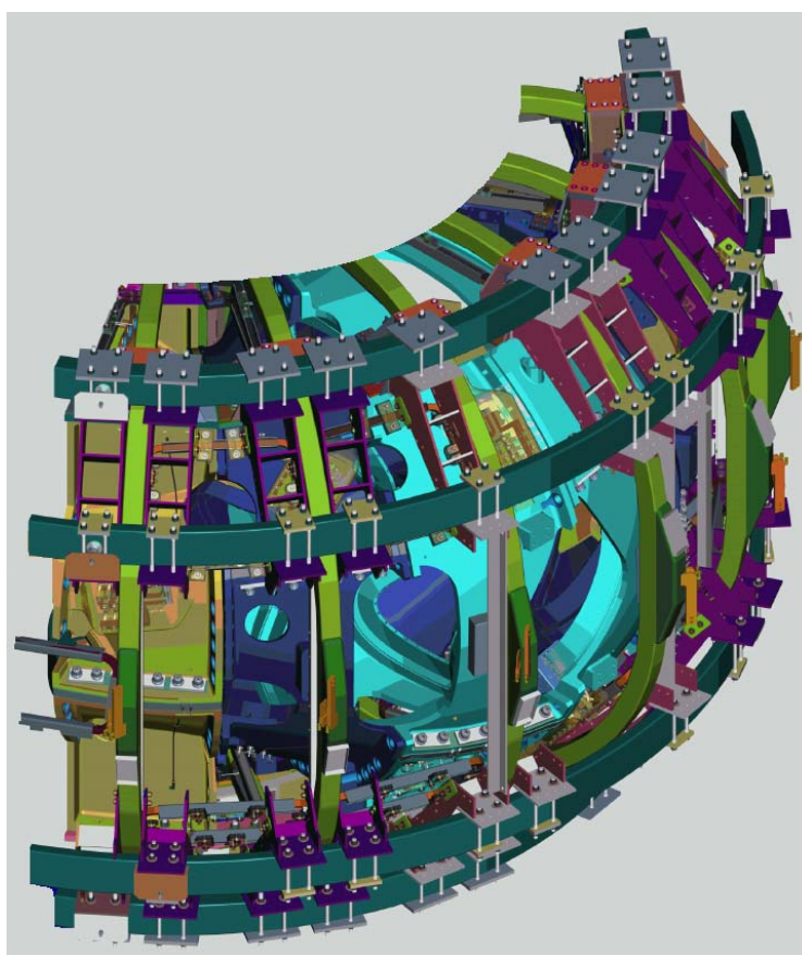
Figure 17: Outer poloidal field coil supports
