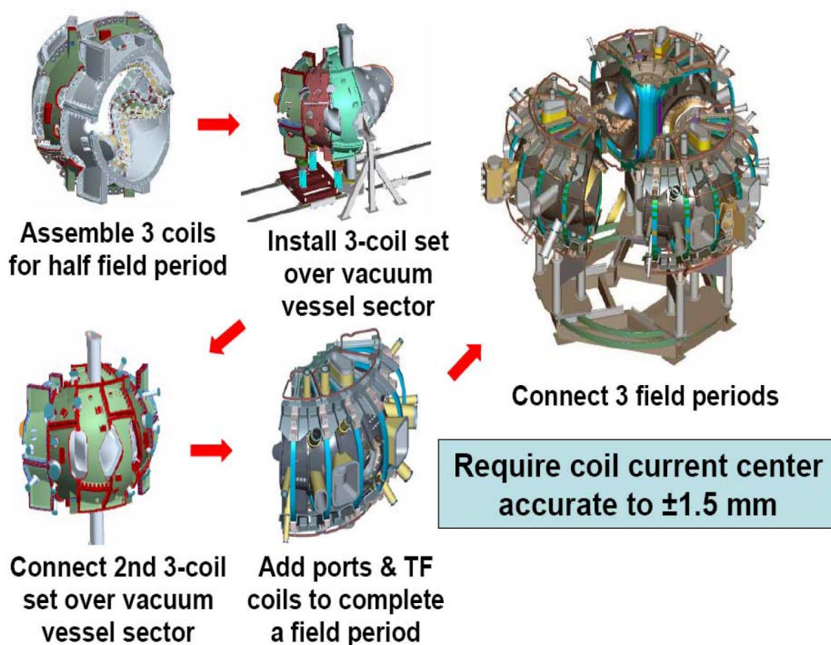
Figure 22: Field Period Assembly (WBS 18) and Final Machine Assembly (WBS 7) sequence schematic
