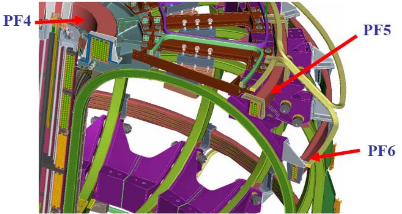
Figure 7: Poloidal field coils design
