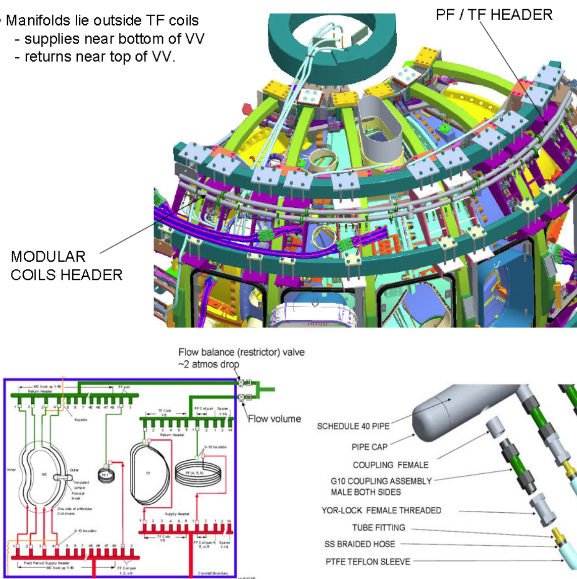
Figure 18: Schematics illustrating LN2 distribution
