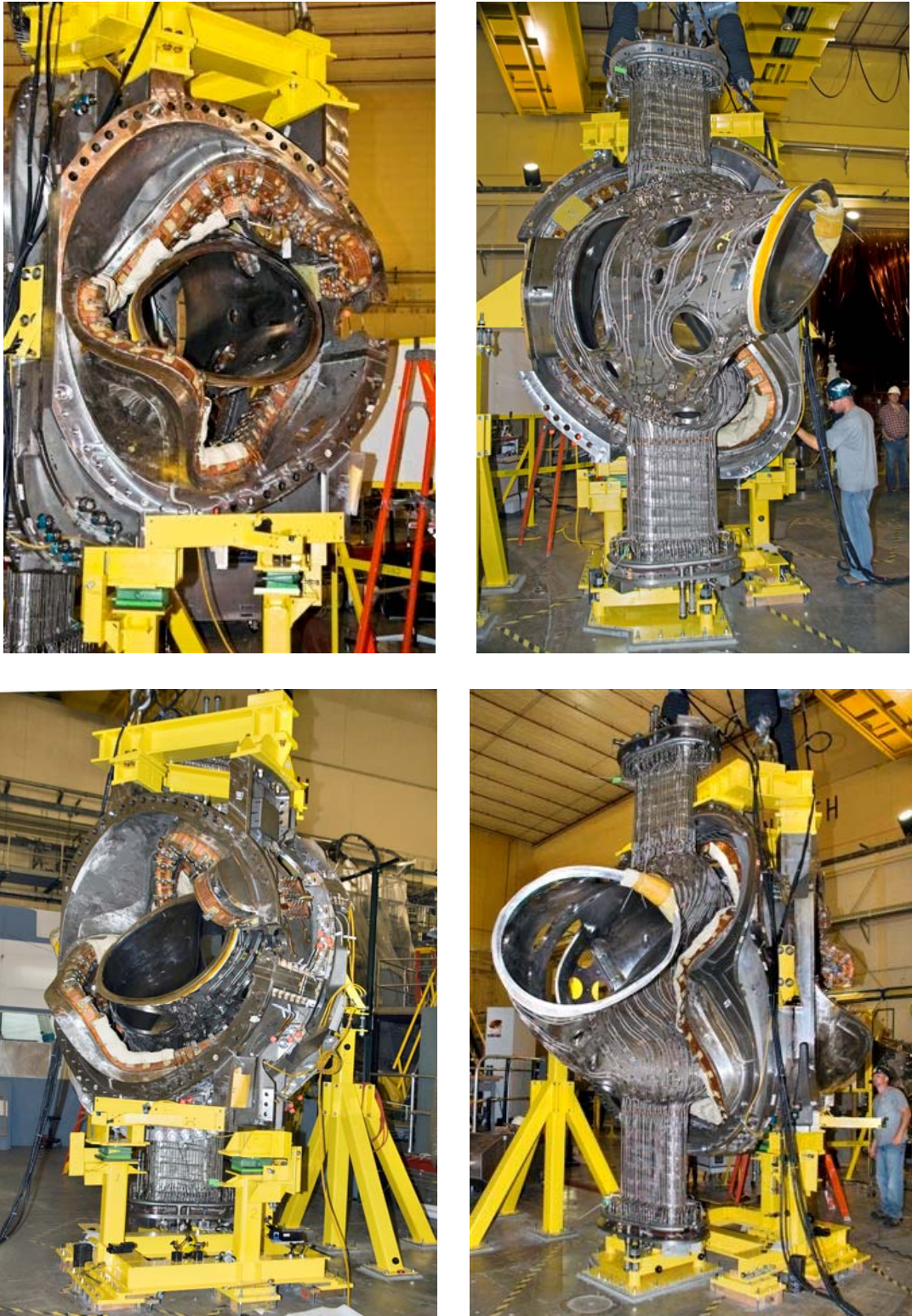
Figure 24: Half-field period assembly installed over vacuum vessel sub assembly.
