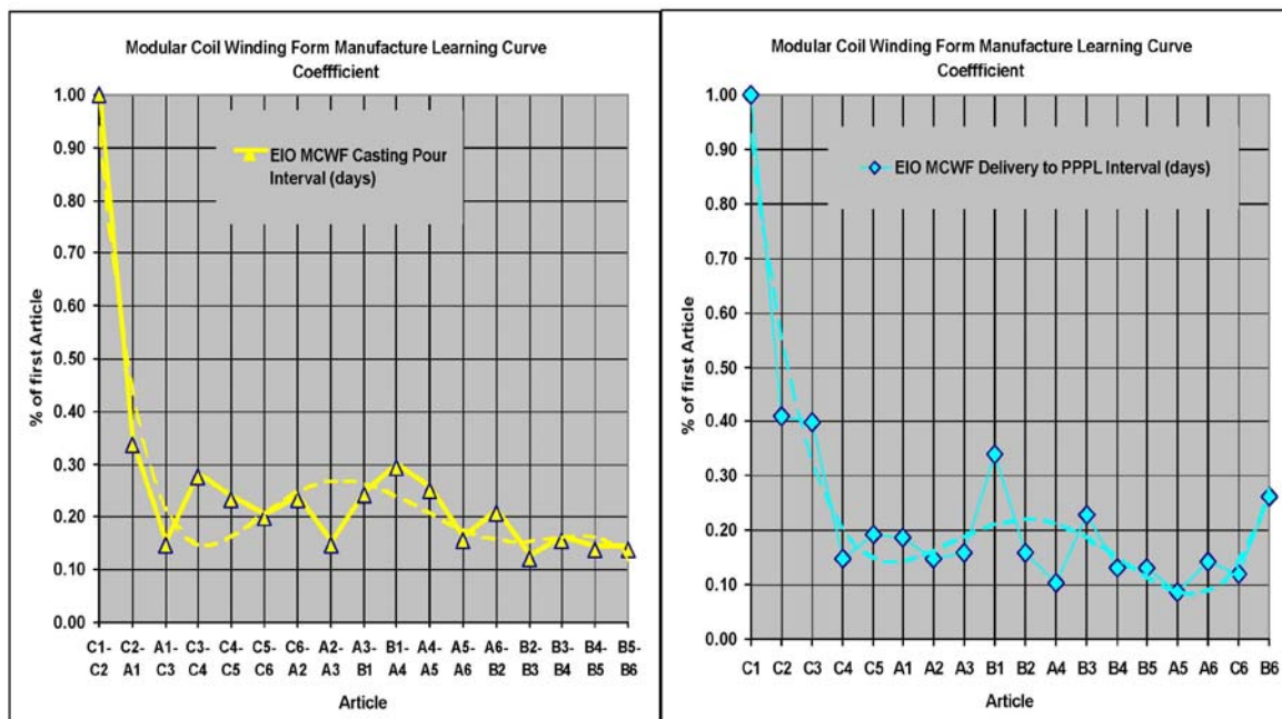
Figure 15: Learning curve for manufacture of MCWF: (1) time intervals between castings normalized to the interval between the first and second article; and (2) time intervals between MCWF deliveries normalized to the time between receipt of the first article casting and delivery of the machined first article to PPPL.
