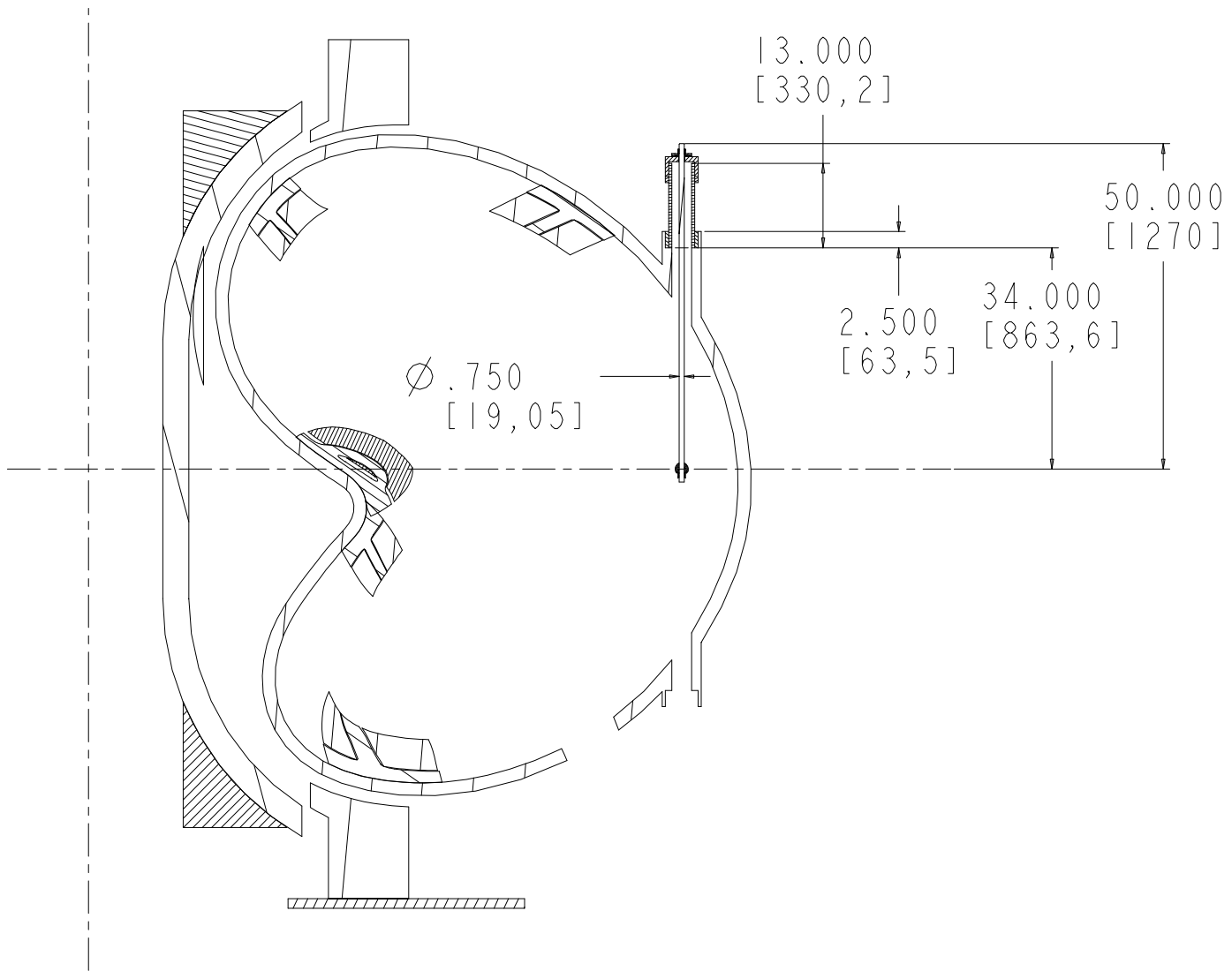
SECTION SECT-13_5-SECT-13_5
