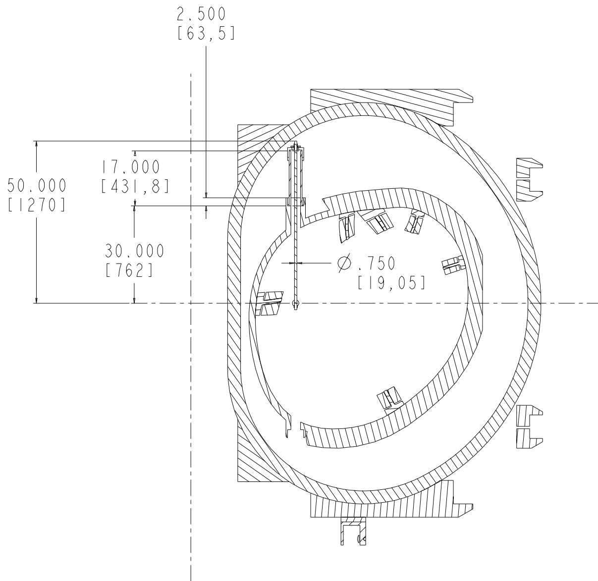
SECTION SECT50-SECT50
