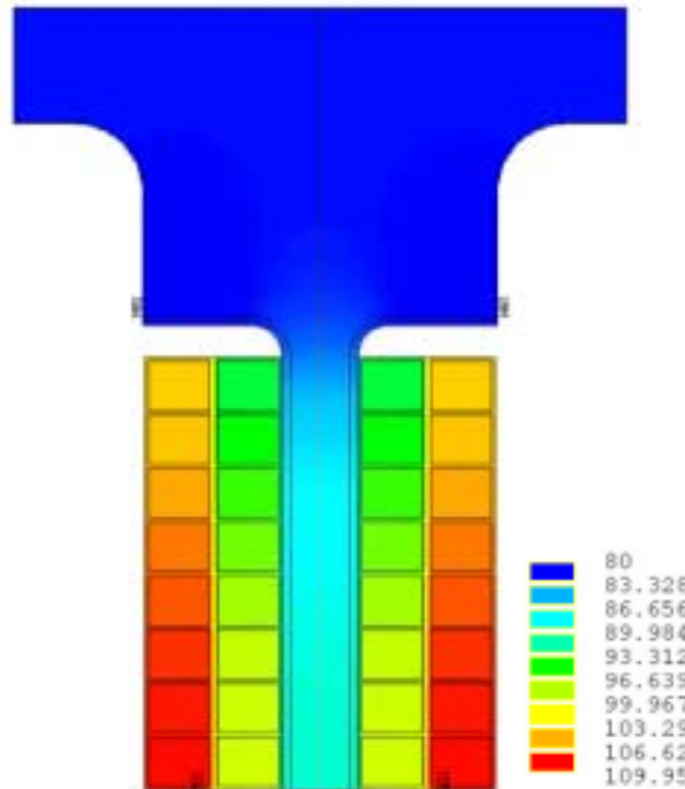
Plate on one side
