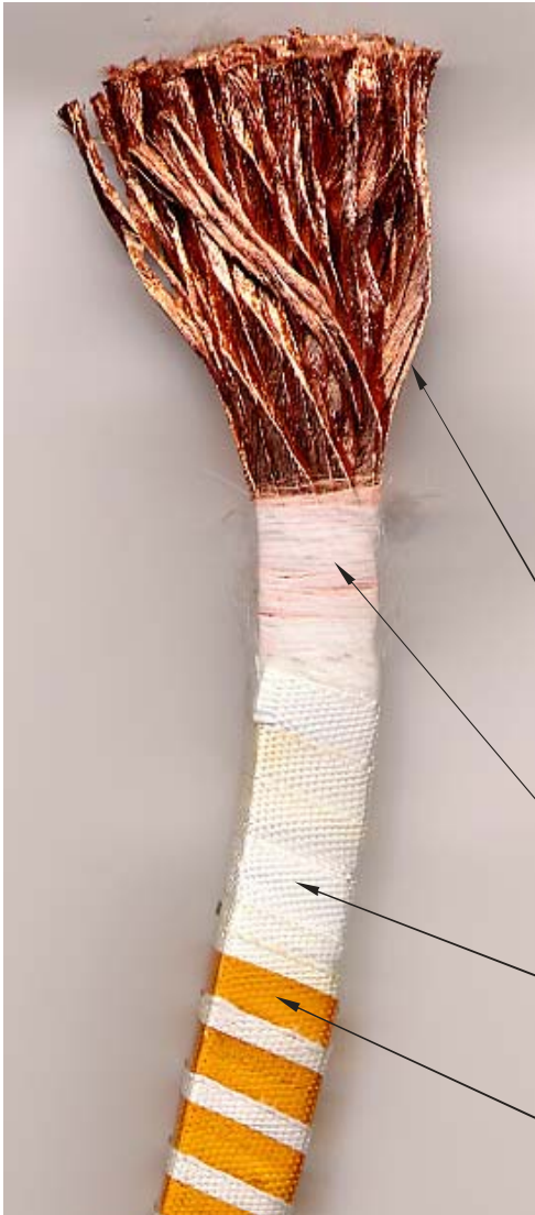
Photograph of actual conductor sample showing insulation components
