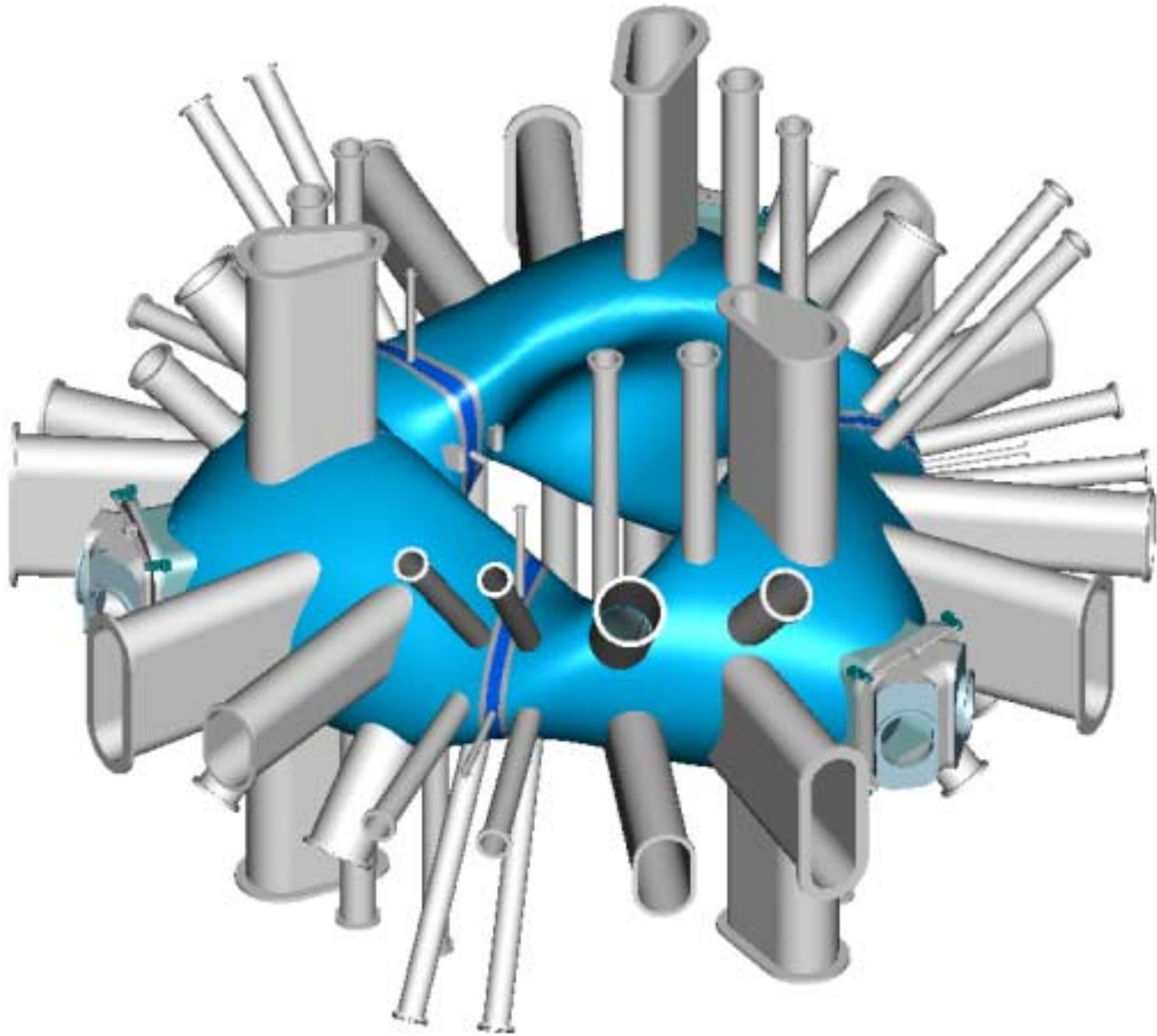
Vacuum Vessel and Ports
