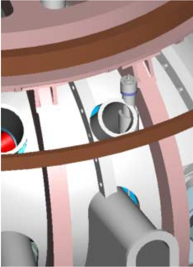
Vacuum Vessel Supports and Vacuum Vessel Port
