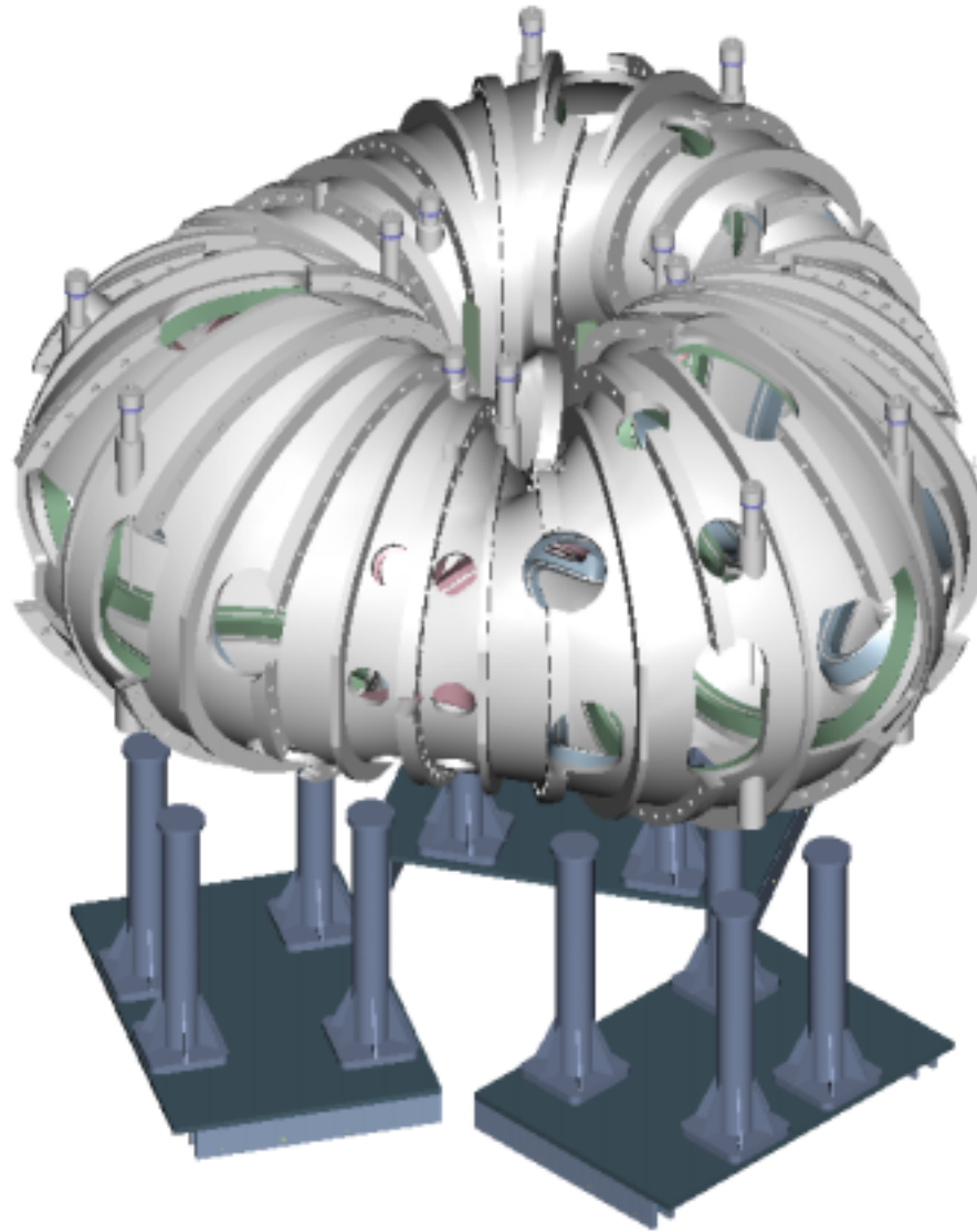
Structural Shell with Supports (TF Supports shown separately)
