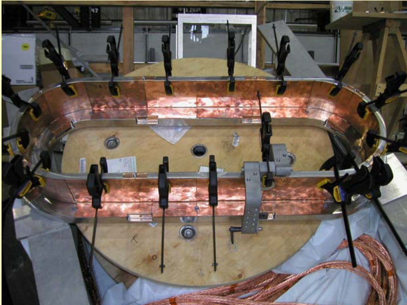
Inner wall of copper cladding
