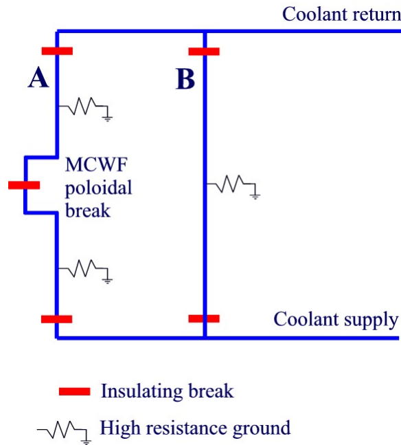
Figure 3-3 Electrical isolation and grounding of coolant loops
