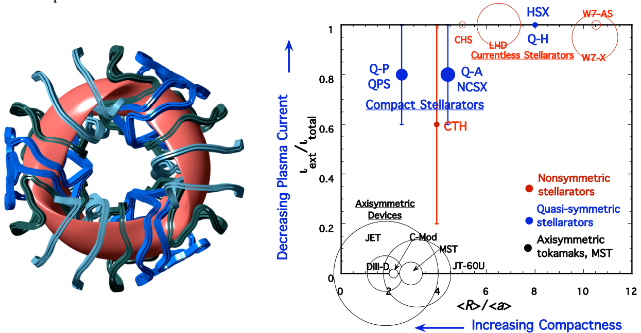
Fig. 1. NCSX plasma surface and coils.
