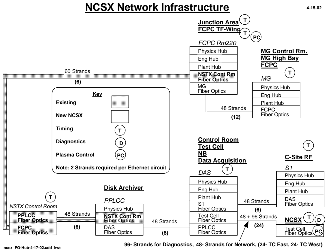
Figure 1 Schematic of Network Infrastructure
