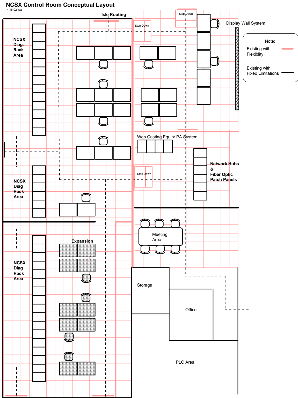
Figure 3 NCSX Control Room Conceptual Layout
