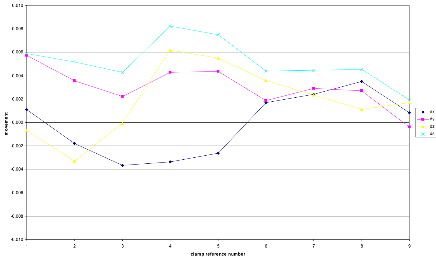
A6 Winding Surface Movement after 25% Weld
