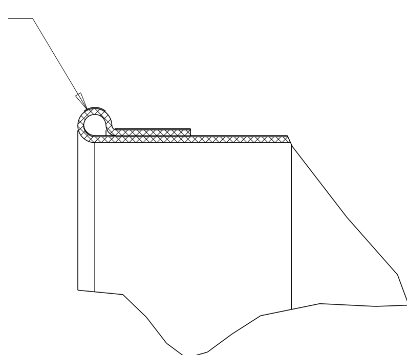
DETAIL B SCALE 2.000
