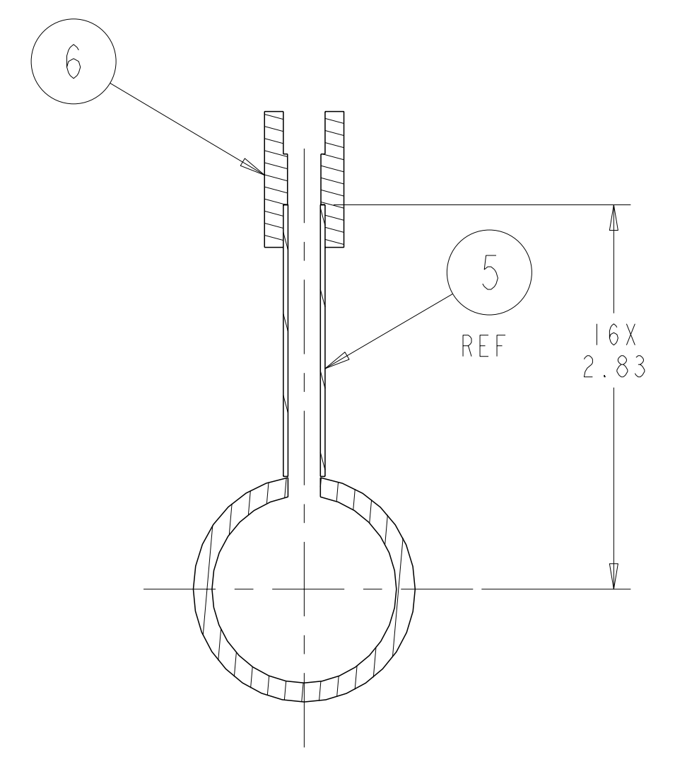
SECTION A-A SCALE 1.00
