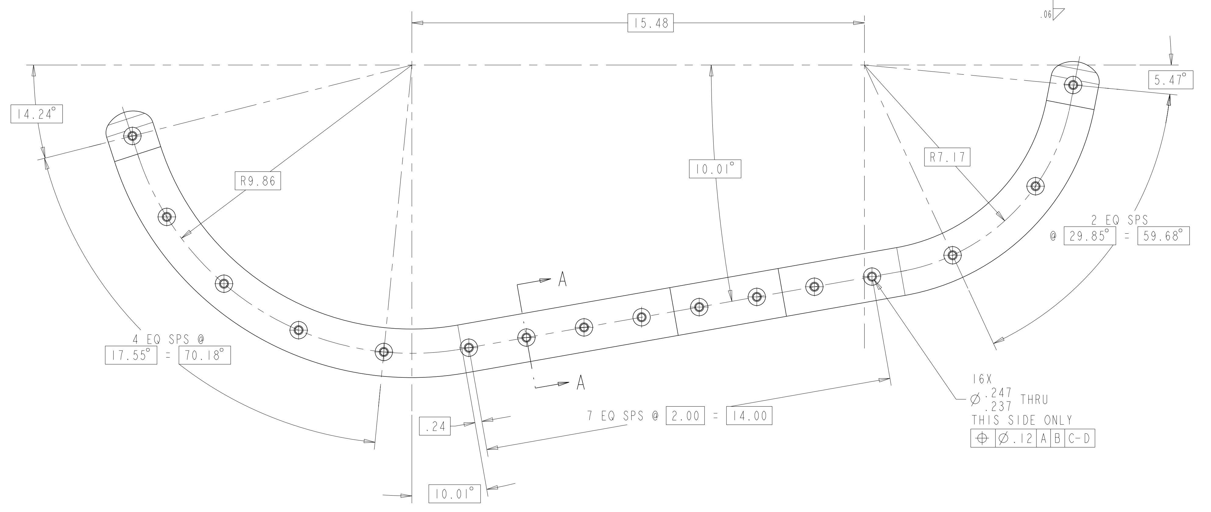
VIEW FOR HOLE LOCATION
