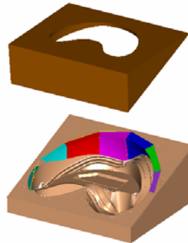
Top and bottom drag box
