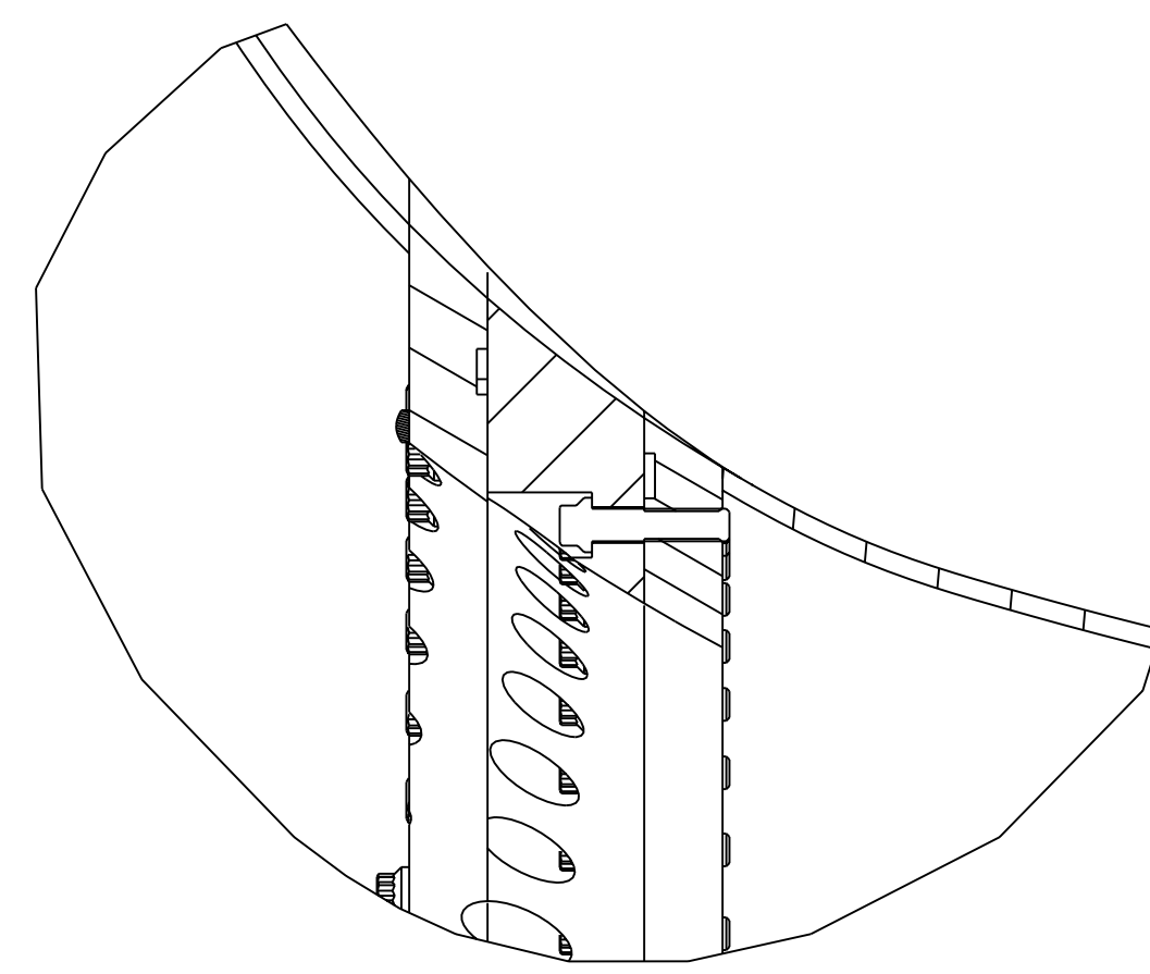
SECTION 13-13
