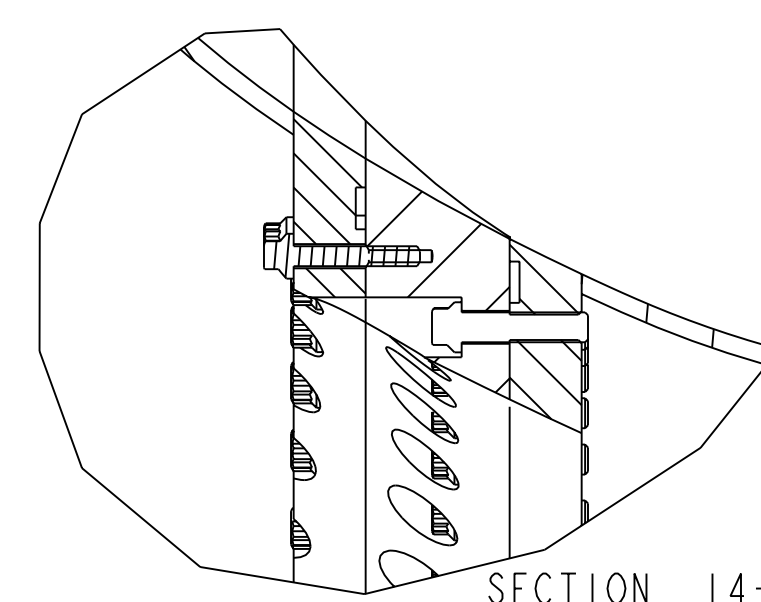
SECTION 14-14
