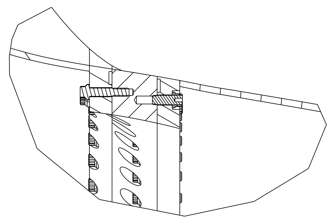
SECTION 16-16
