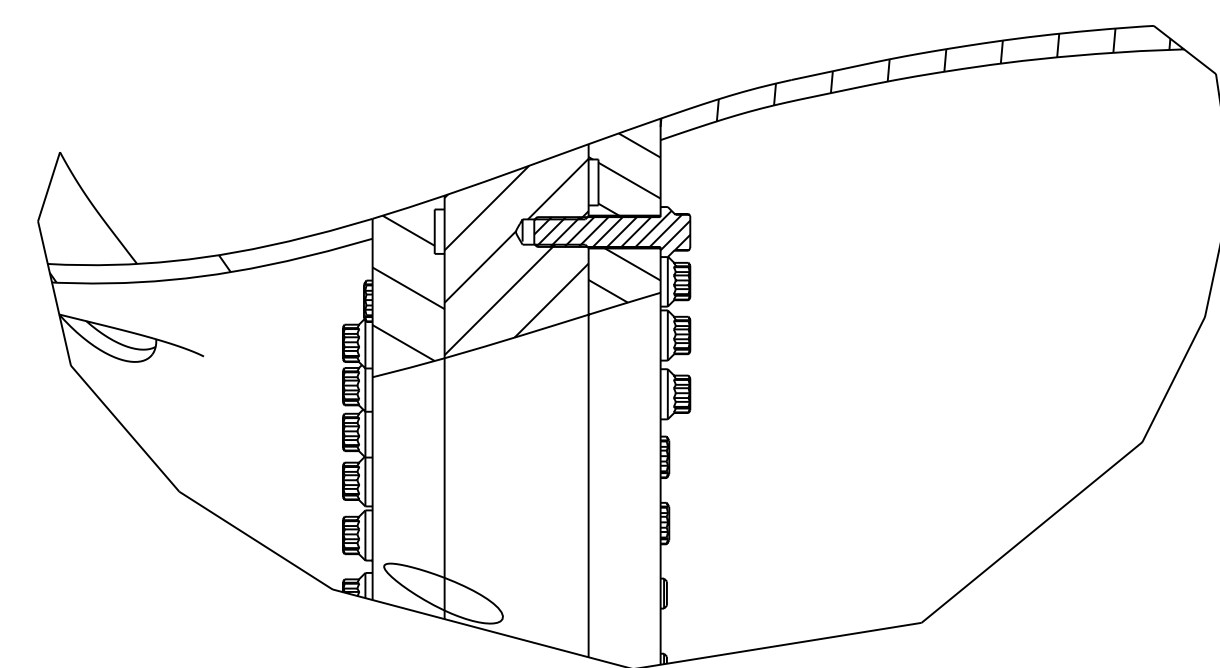
SECTION 20-20
