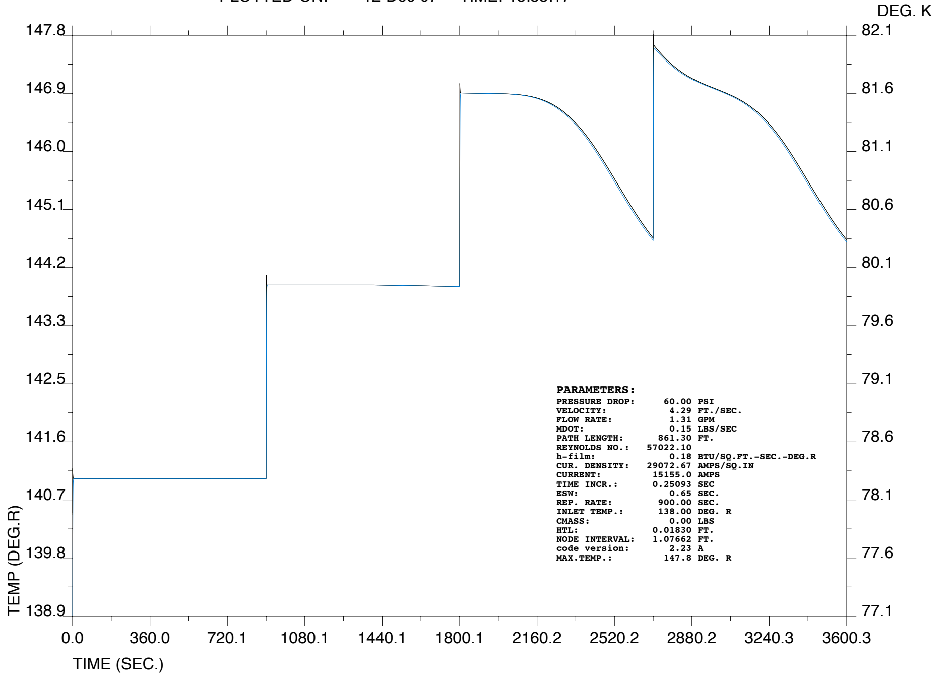
NCSX PF4 Coil LN2-cooling 15.15kA, 0.65 ESW
