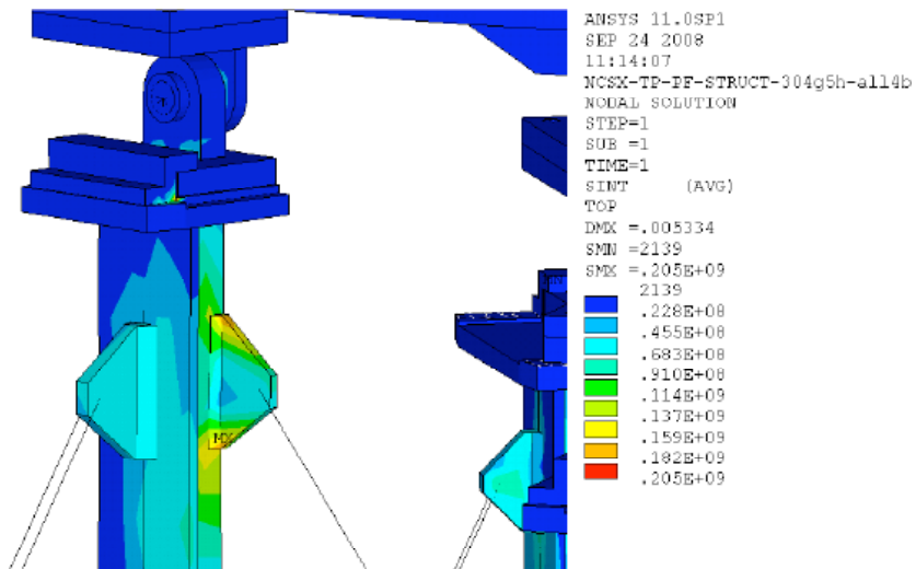
Figure 9b Peak Tresca stress contours at R.T. - 1.7T Ohmic -peak stress is 29.7 ksi
