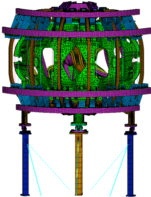
Figure 5a. Fully integrated model of NCSX single period
