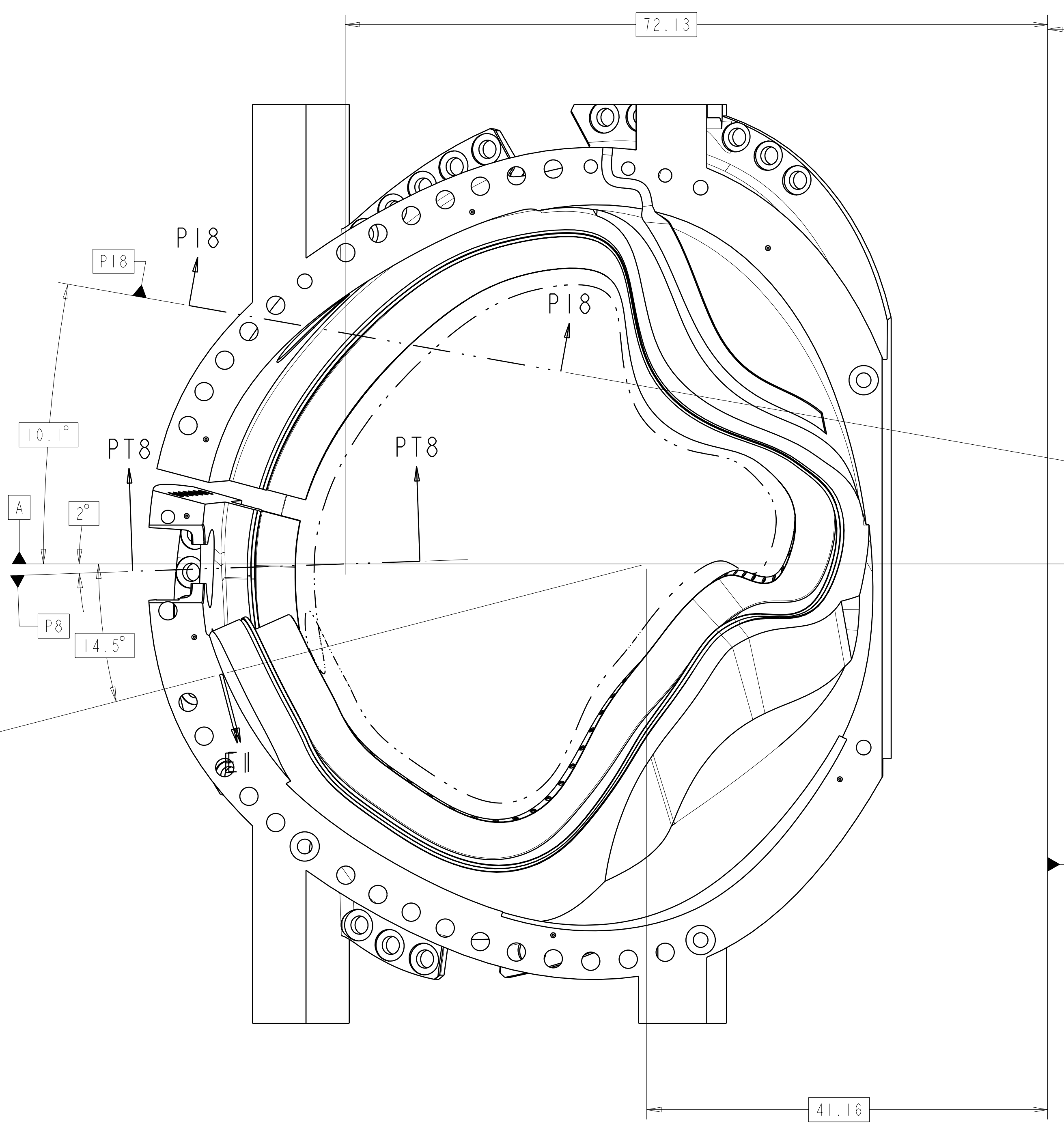
VIEW AT DATUM E SCALE 0.13
