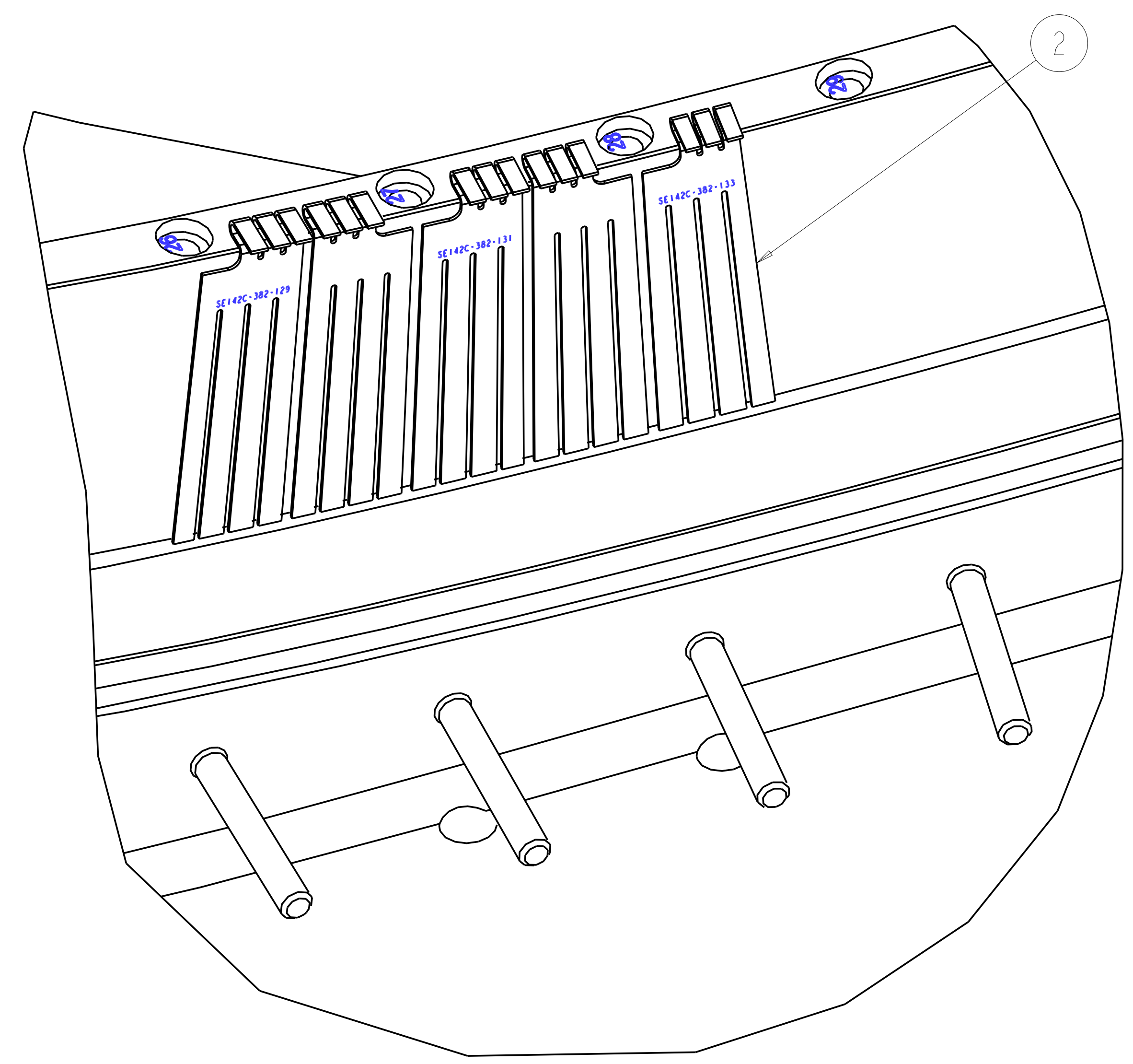
ISOMETRIC VIEW
