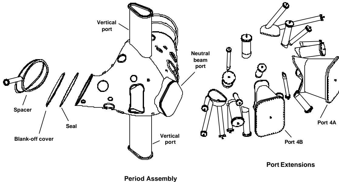
Figure 1 - VVSA Components
