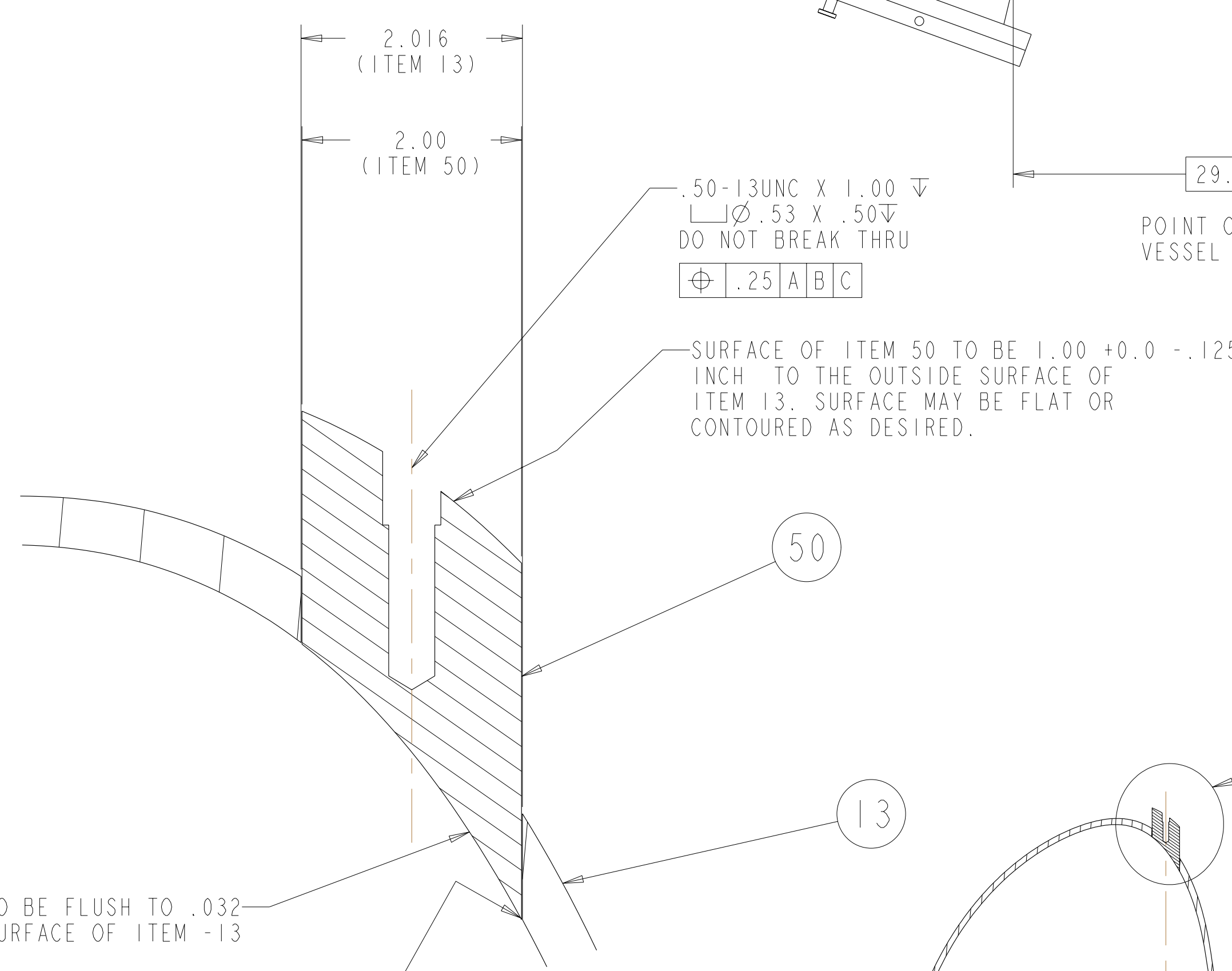
TOP VIEW
