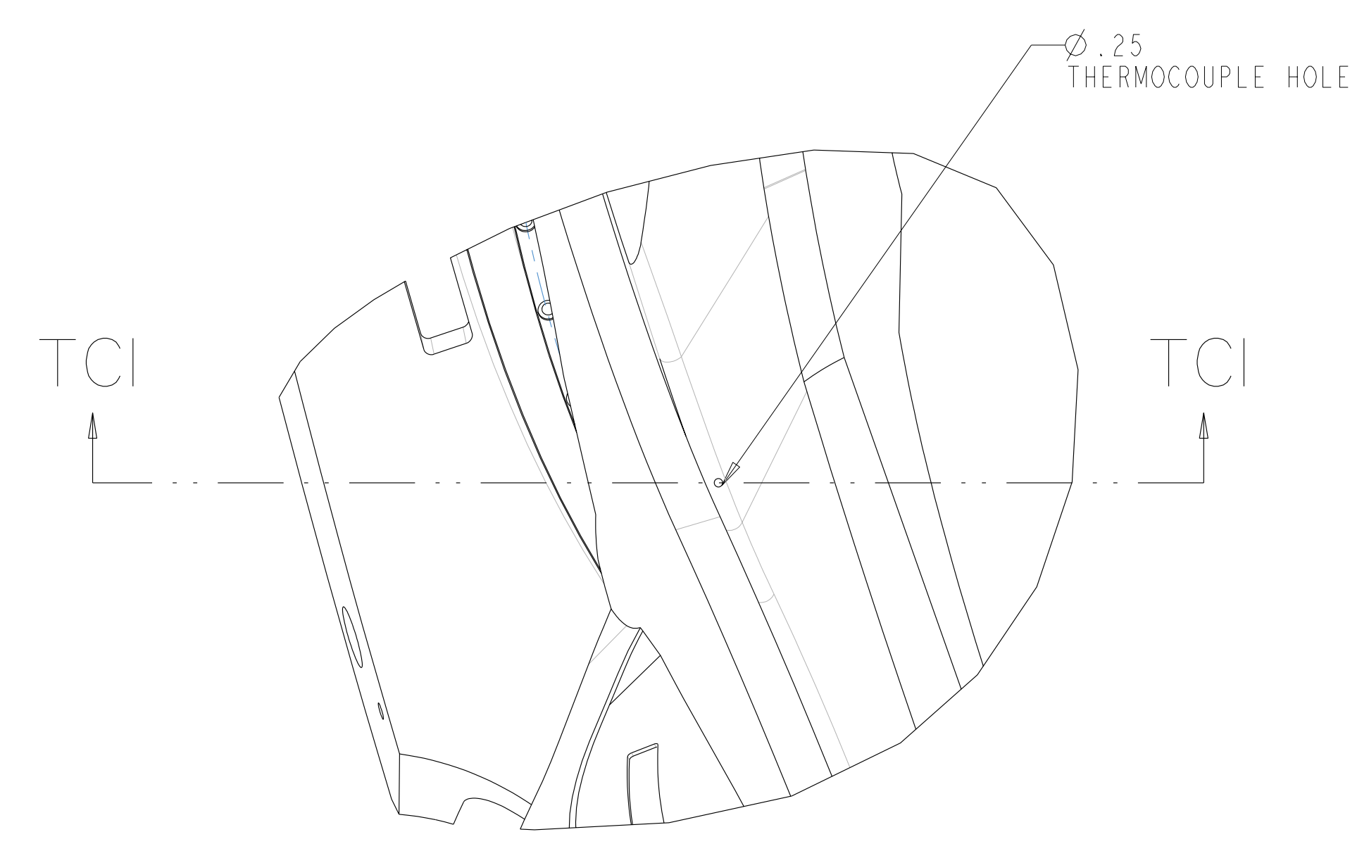
THERMOCOUPLE HOLE SCALE 0.250 USE PRO/E MODEL GEOMETRY TO DETERMINE SECTION ORIENTATION
