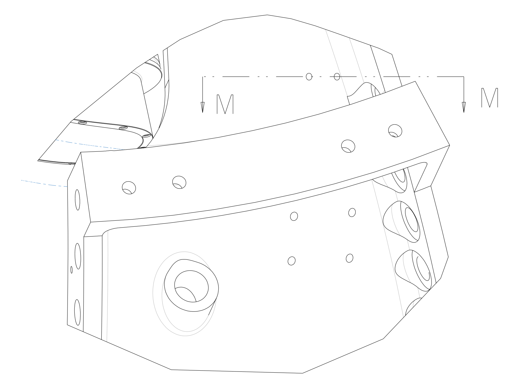
VPI BLEED HOLES SCALE 0.250 USE PRO/E MODEL GEOMETRY TO DETERMINE SECTION ORIENTATION
