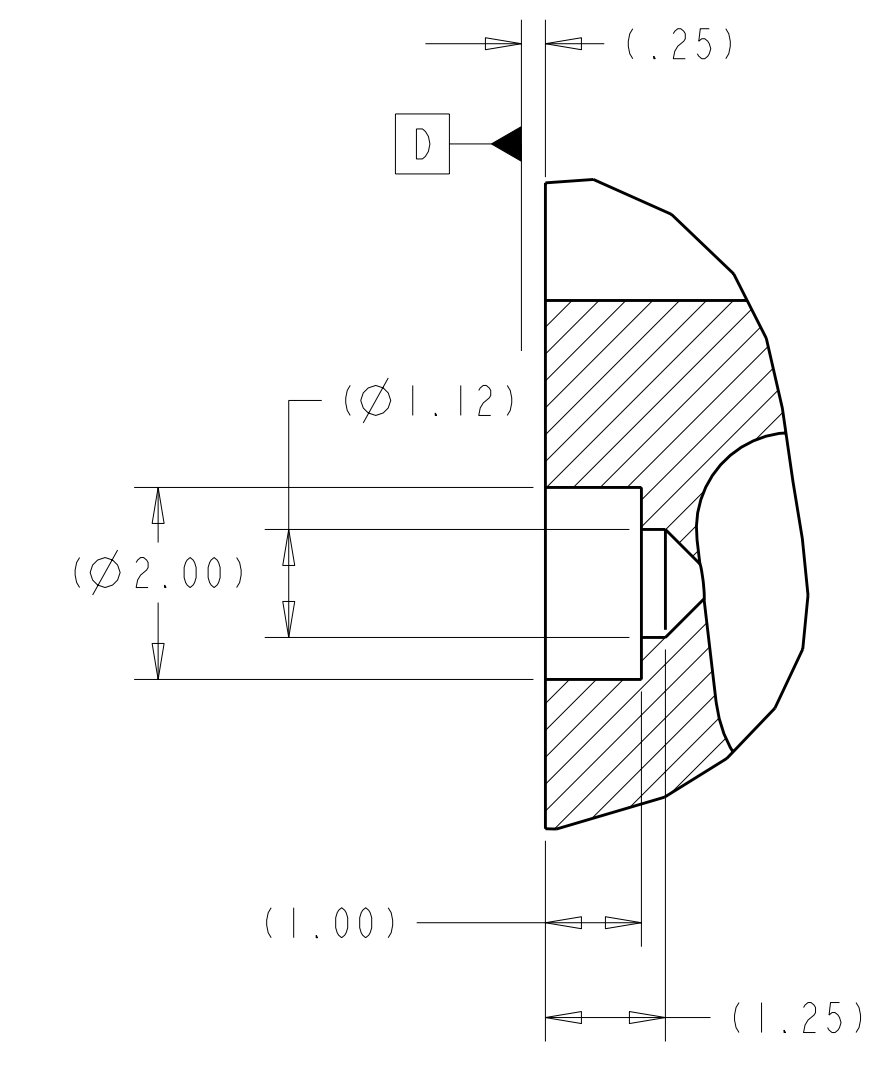
DETAIL X SCALE 0.50
