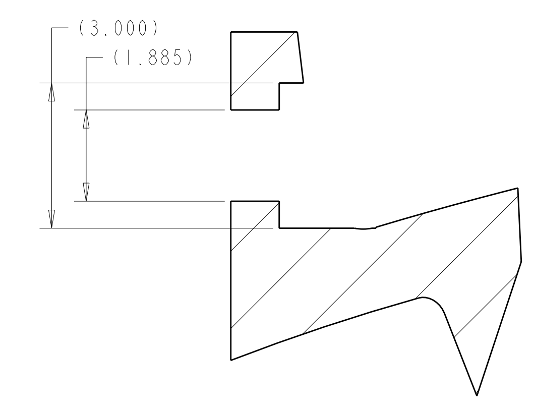
SECTION E-E SCALE 0.500
