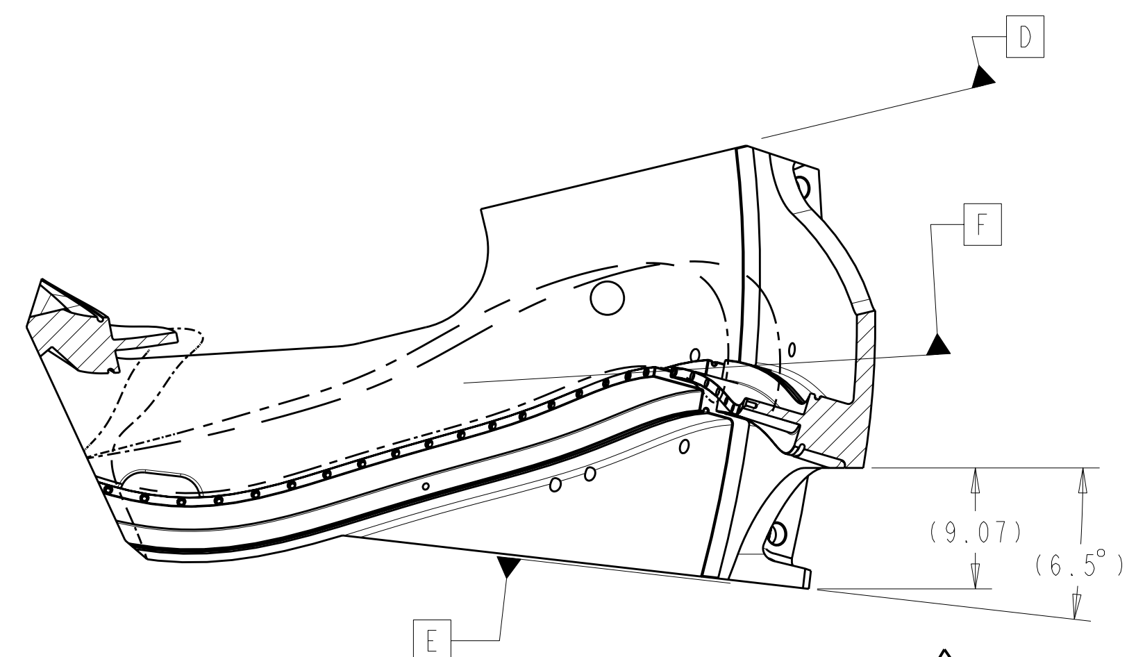
SECTION P4-P4 SCALE 0.1
