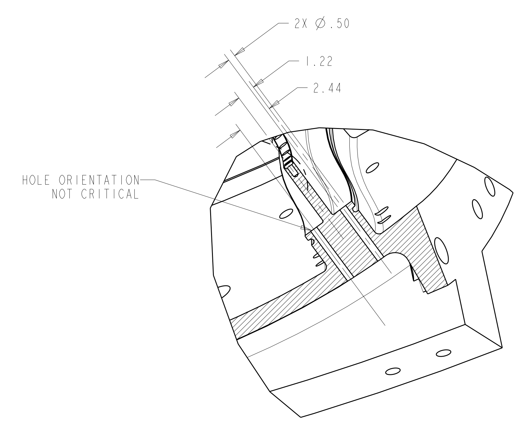
SECTION M-M
