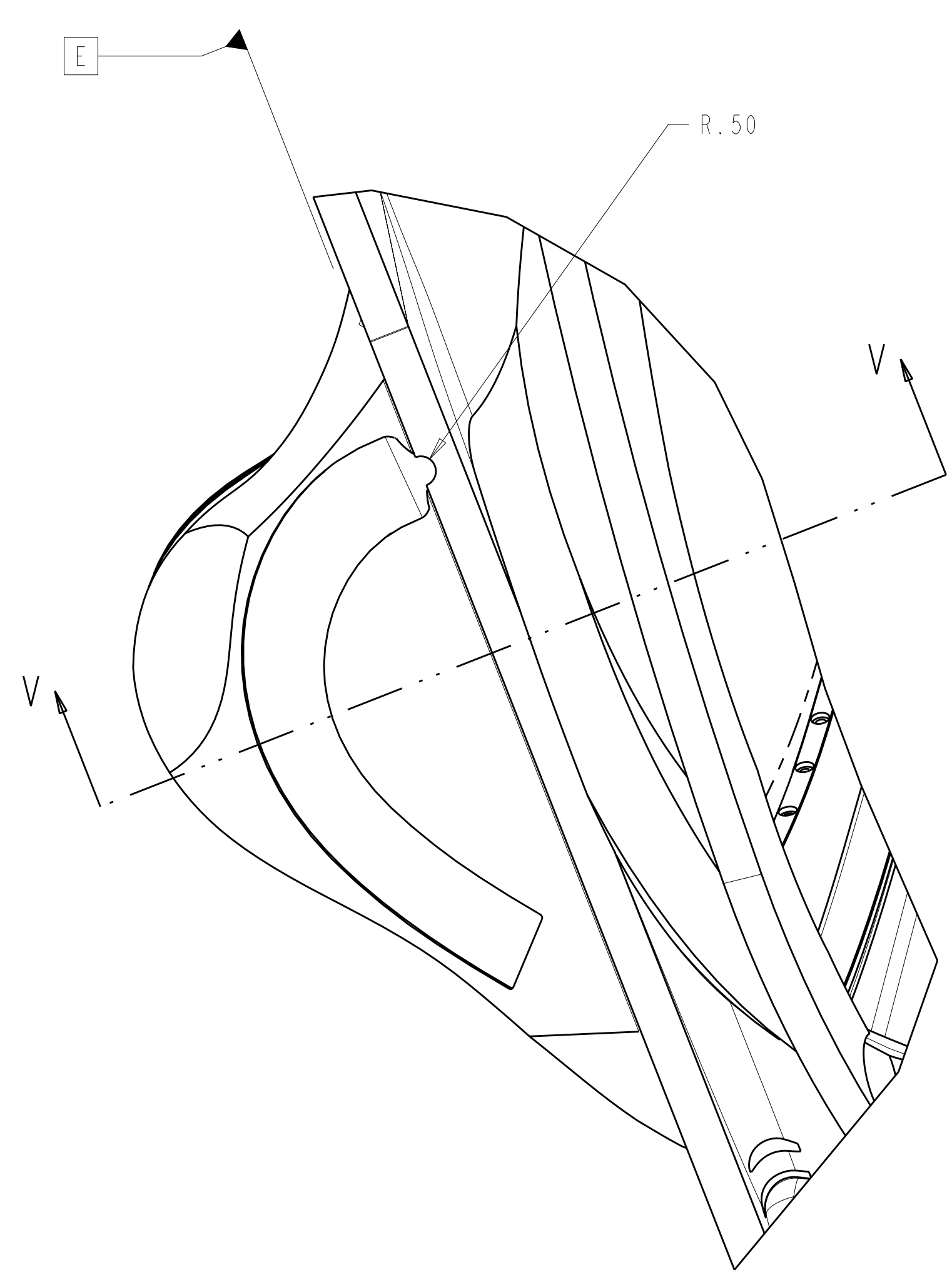
DETAIL E WING SHIM POCKET SCALE 0.25
