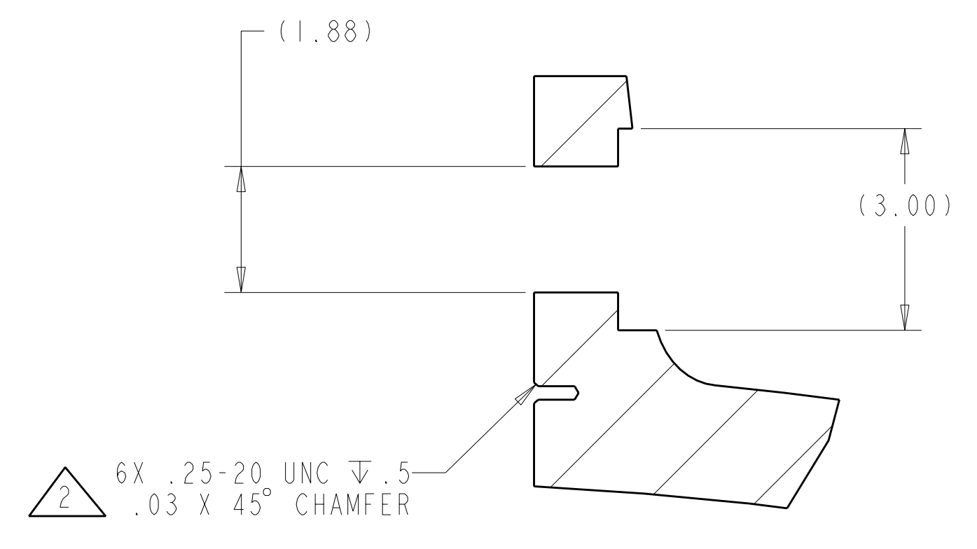
SECTION S-S SCALE 0.50
