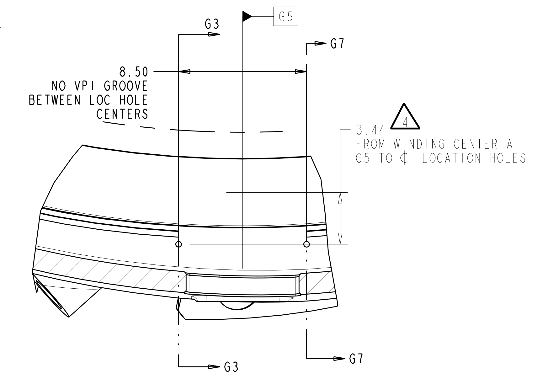
SECTION G2-G2 SCALE 0.250
