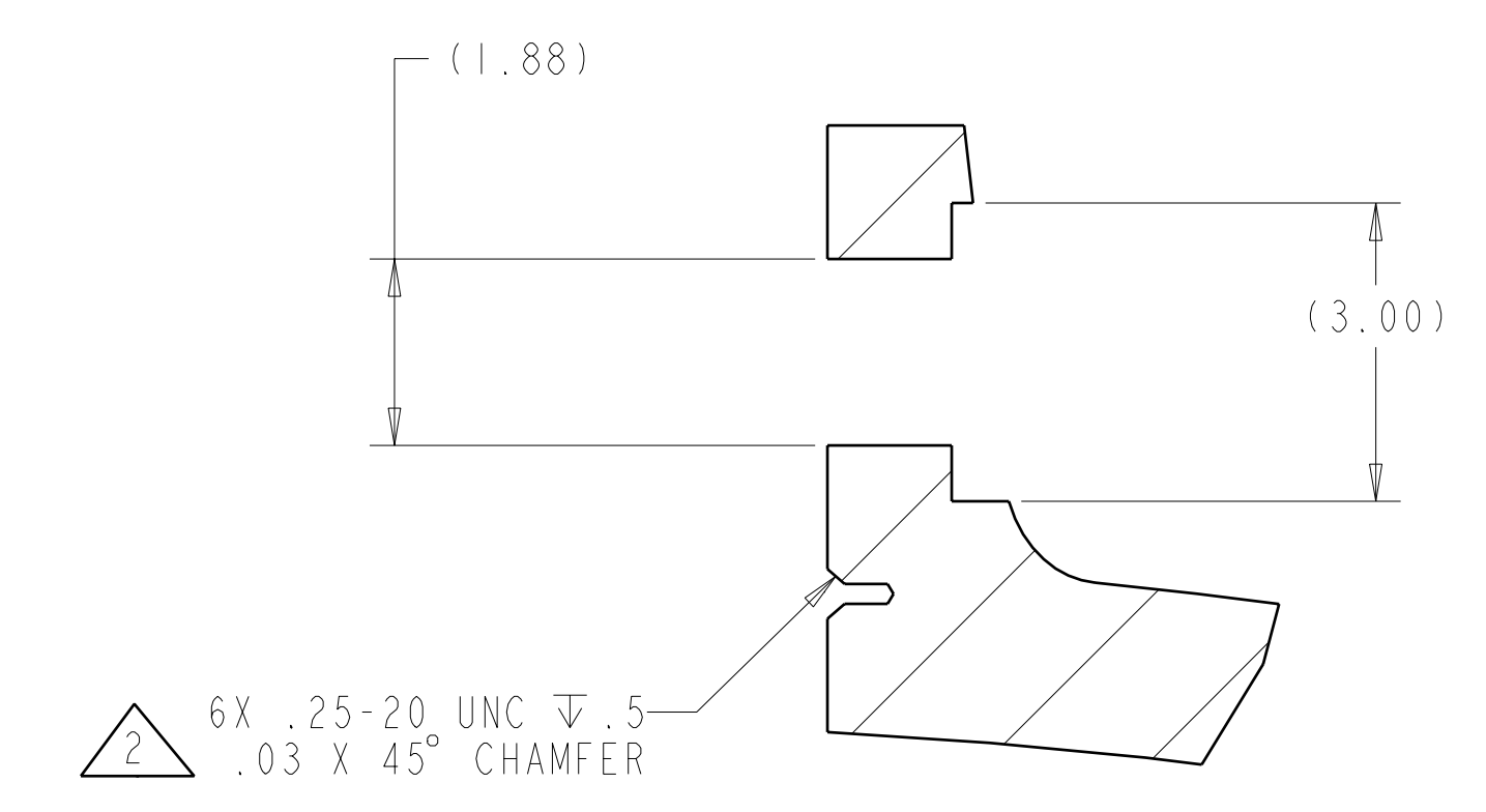
SECTION S-S SCALE 0.50
