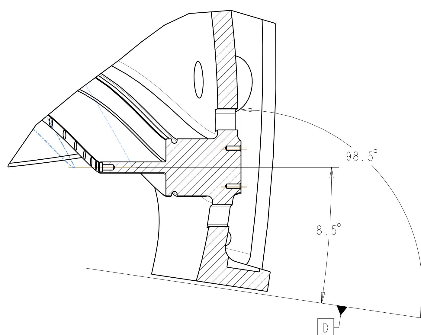
SECTION G-G LEAD BLOCK DETAIL SCALE 0.25
