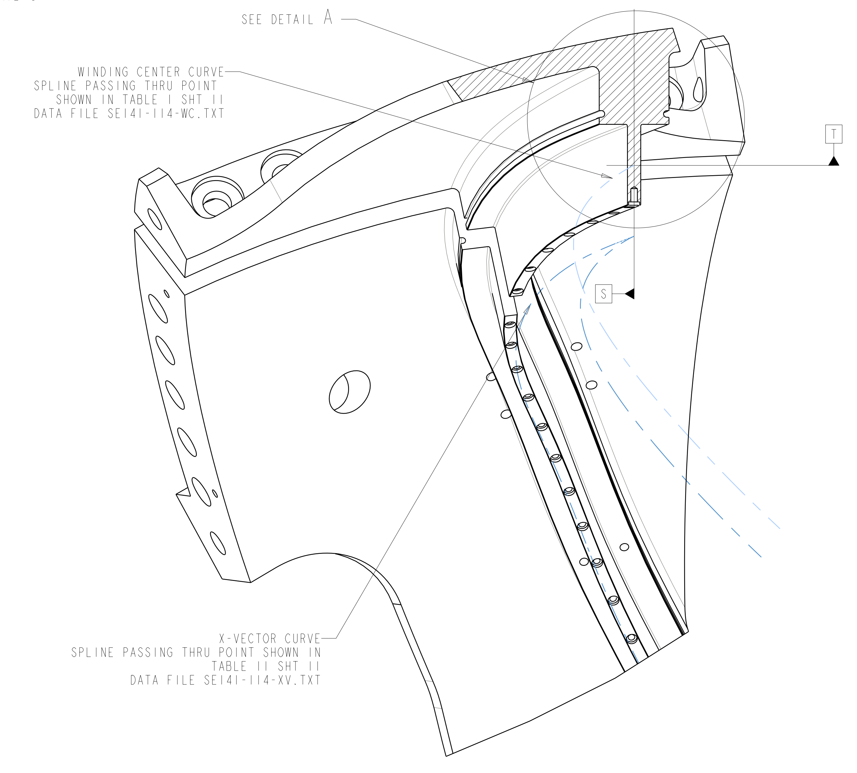
SECTION R-R SCALE 0.30
