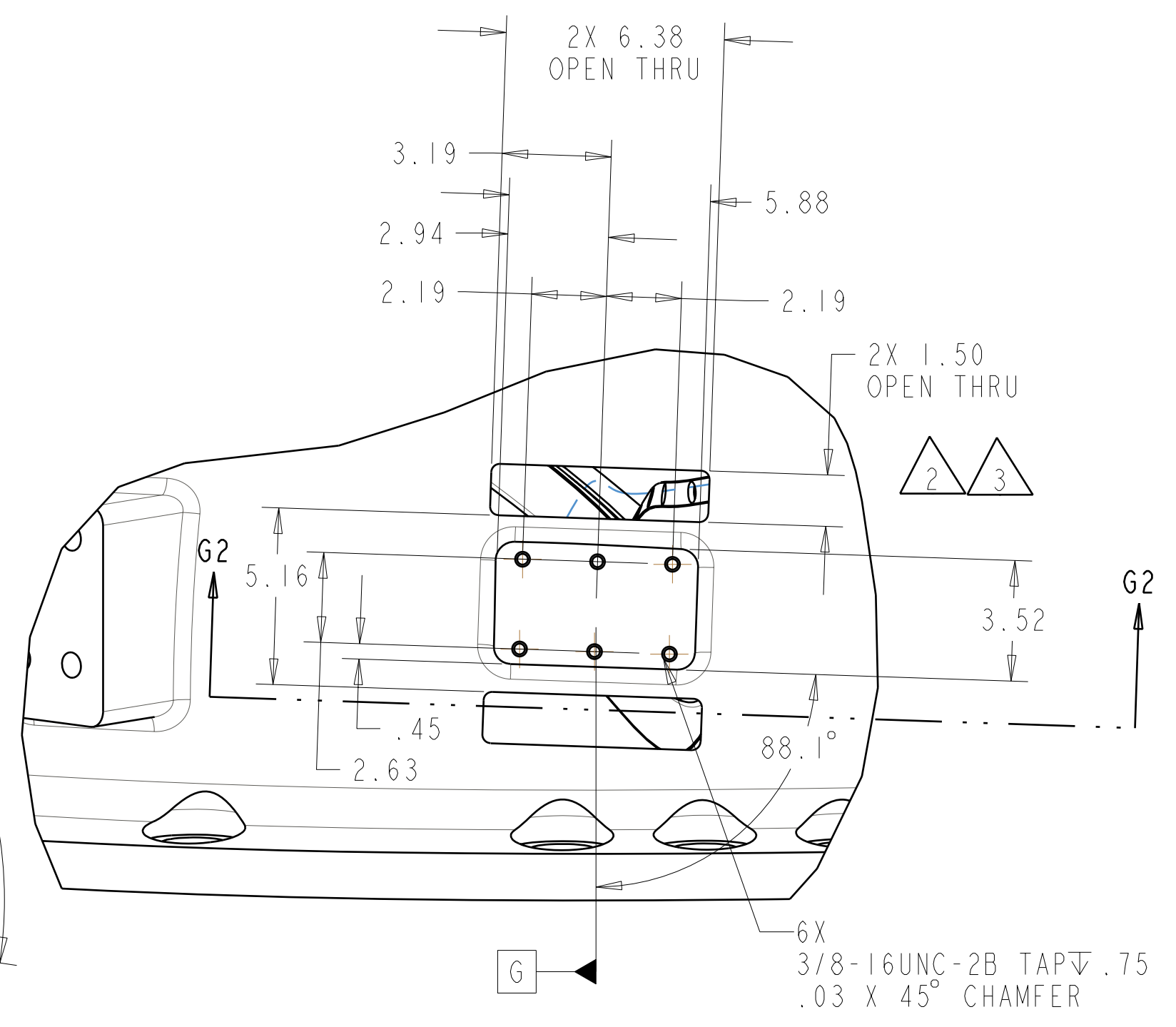
DETAIL J ASSEMBLY FIXTURE MOUNT SCALE 0.25
