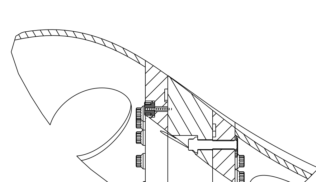
SECTION 7-7
