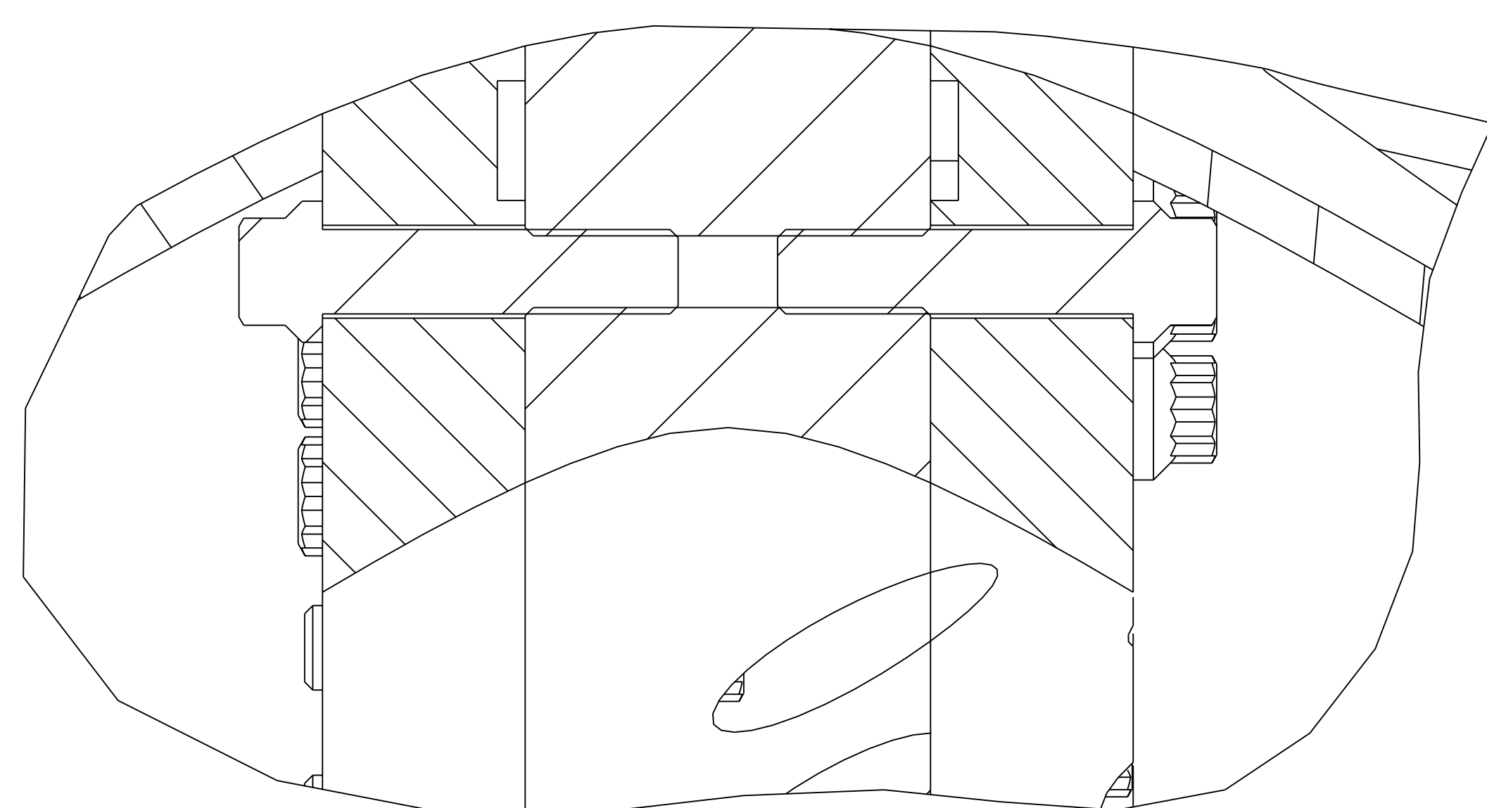
SECTION 1-1 SCALE 1.000
