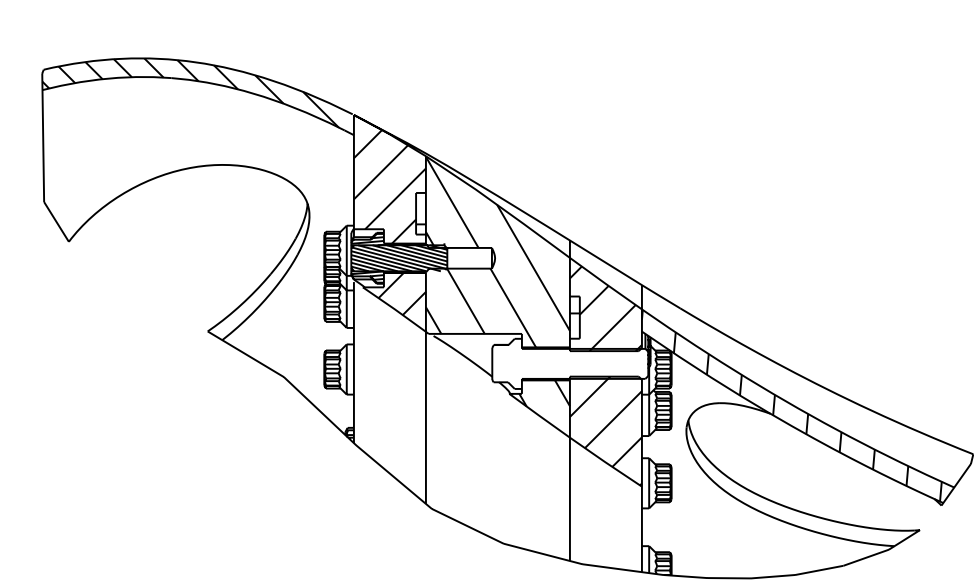
SECTION 6-6
