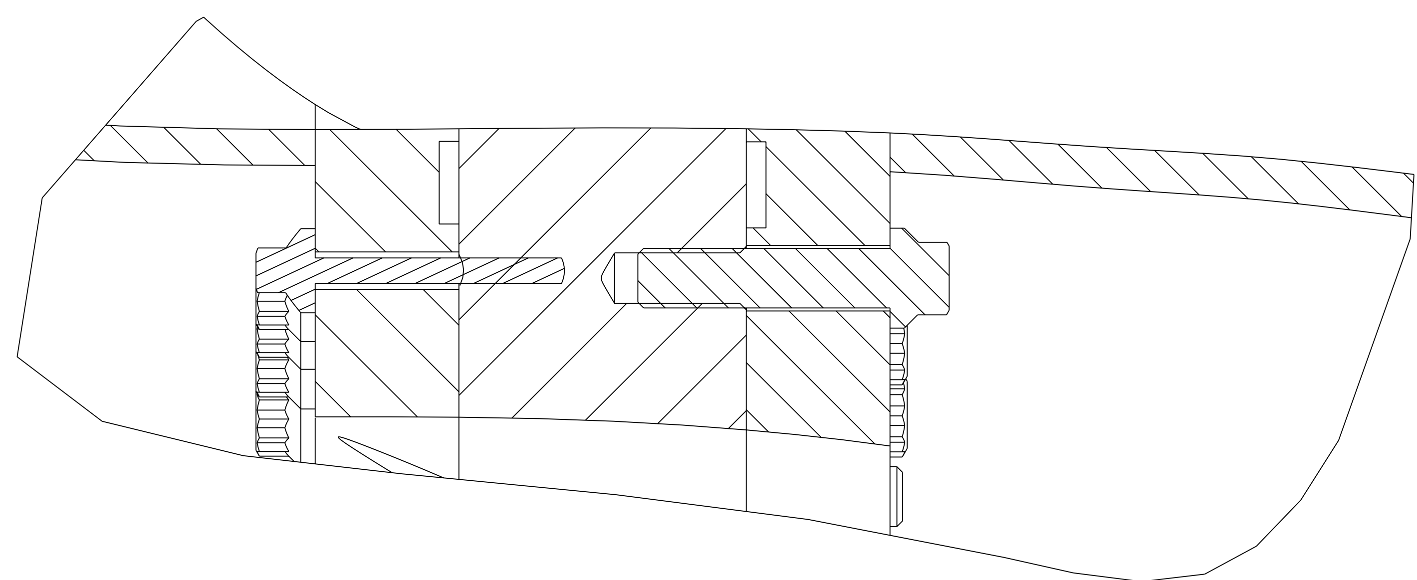
SECTION 17-17 SCALE 1.000
