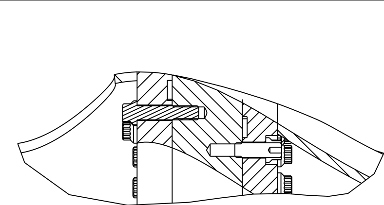
SECTION 3-3
