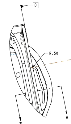
AUX VIEW TO SHOW WING SHIM POCKET
