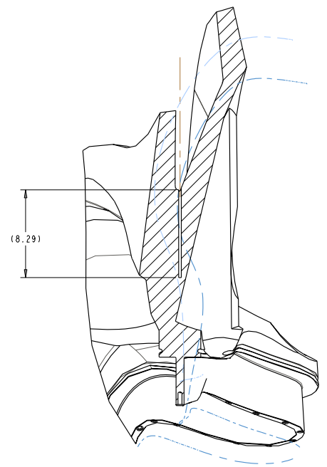
SECTION TCI-TCI
