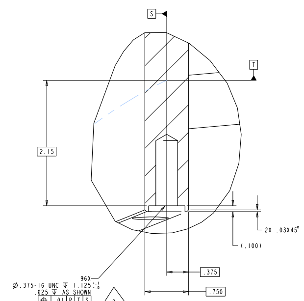
DETAIL C SCALE 2.00
