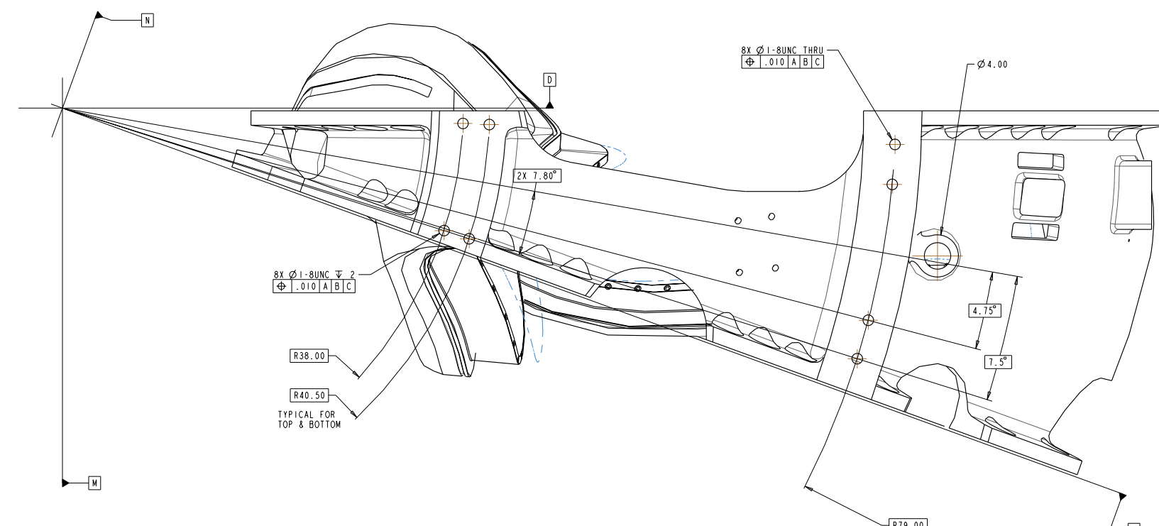
BOTTOM VIEW SCALE 0.25
