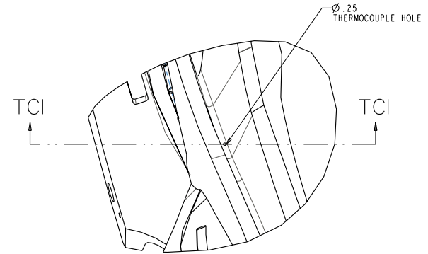
THERMOCOUPLE HOLE SCALE 0.250 USE PRO/E MODEL GEOMETRY TO DETERMINE SECTION ORIENTATION
