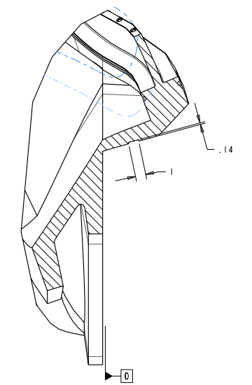
SECTION W-W WING SHIM POCKET SCALE 0.25
