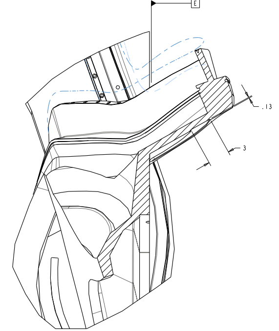
SECTION V-V SCALE 0.25
