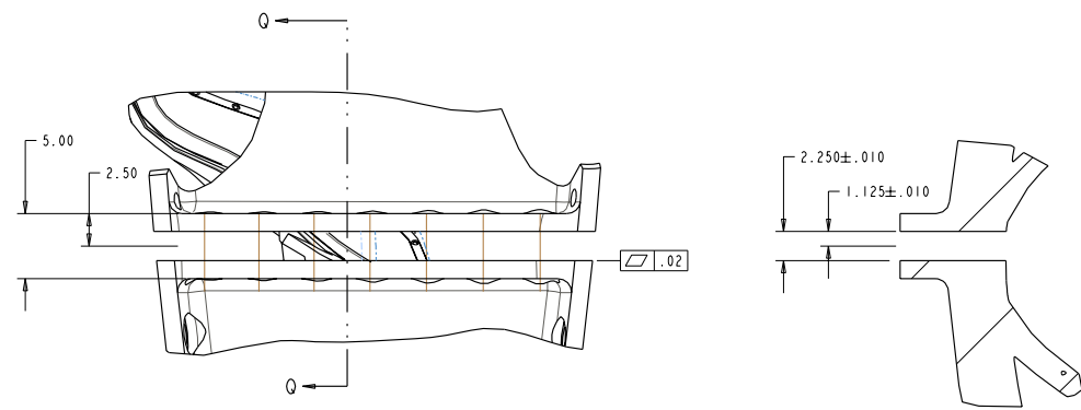
SECTION Q-Q
