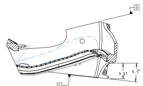
SECTION P4-P4 SCALE 0.1
