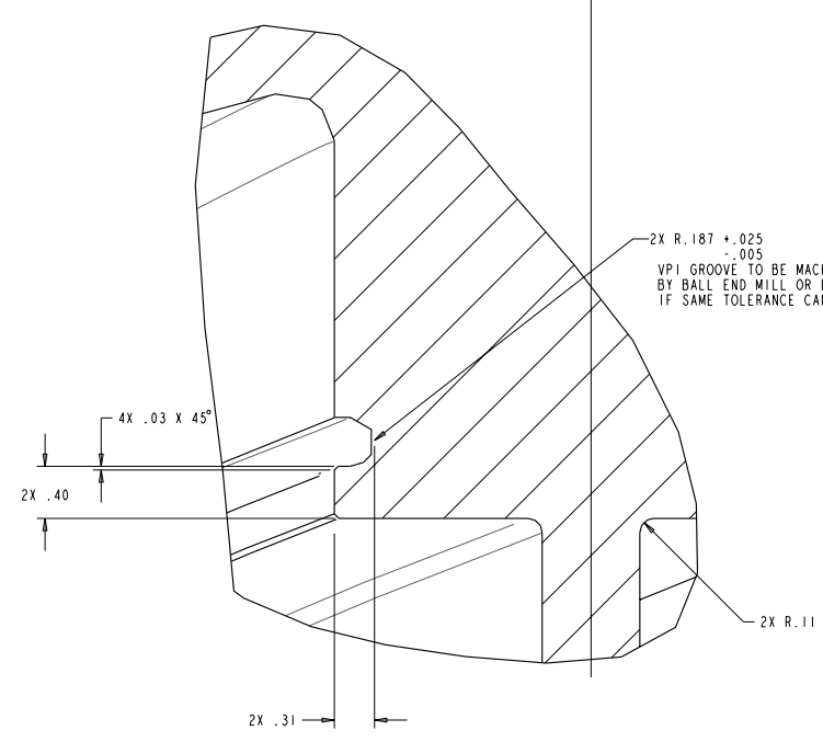
DETAIL B SCALE 2.00
