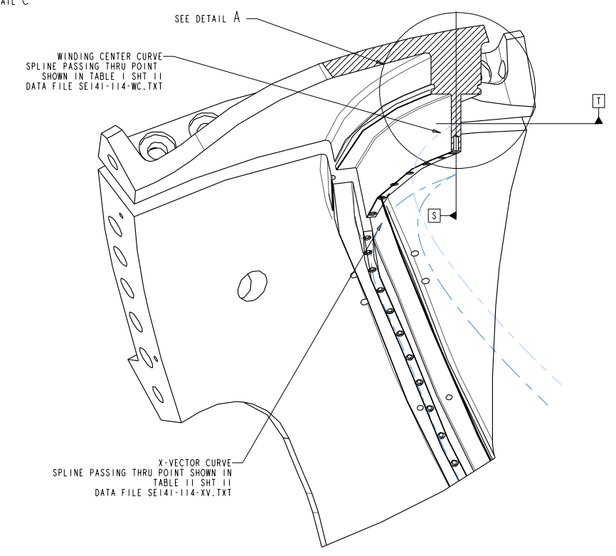
SECTION R-R SCALE 0.30
