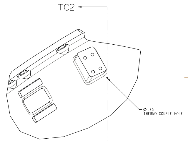
THERMOCOUPLE HOLE SCALE 0.250 USE PRO/E MODEL GEOMETRY TO DETERMINE SECTION ORIENTATION
