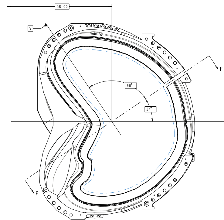
POLOIDAL BREAK DETAIL SCALE 0.10
