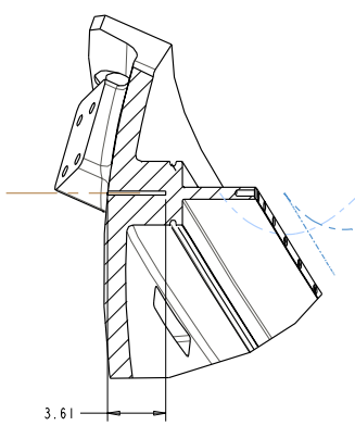
SECTION TC2-TC2
