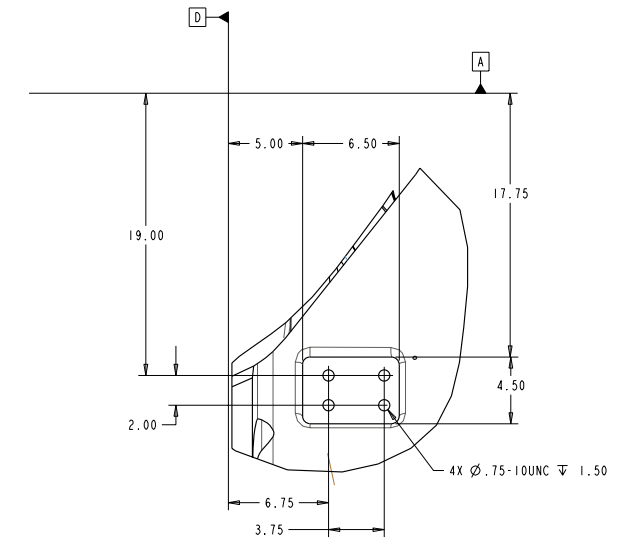
DETAIL J ASSEMBLY FIXTURE MOUNT SCALE 0.25
