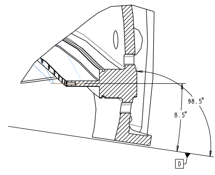
SECTION G-G LEAD BLOCK DETAIL SCALE 0.25
