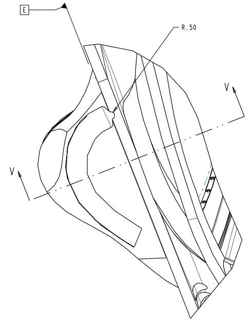
DETAIL E WING SHIM POCKET SCALE 0.25
