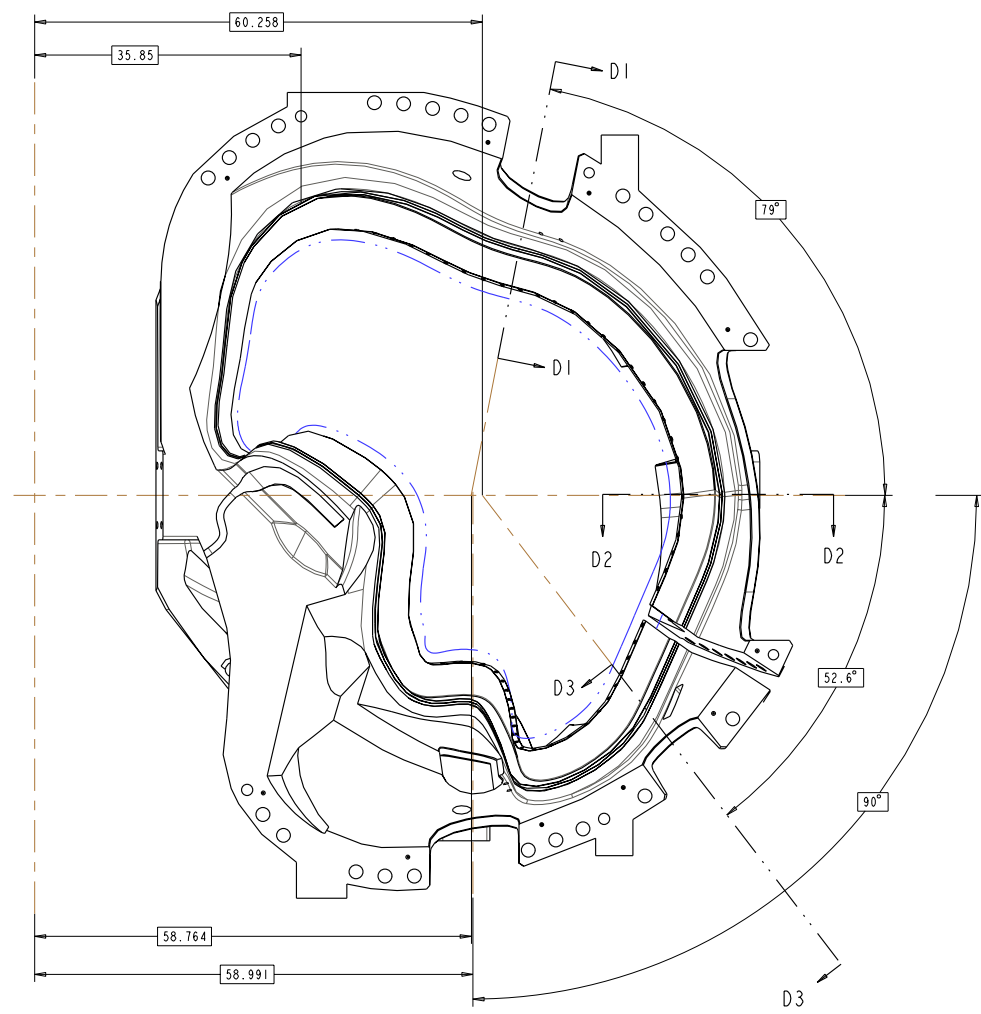
VIEW AT DATUM D SCALE 0.13
