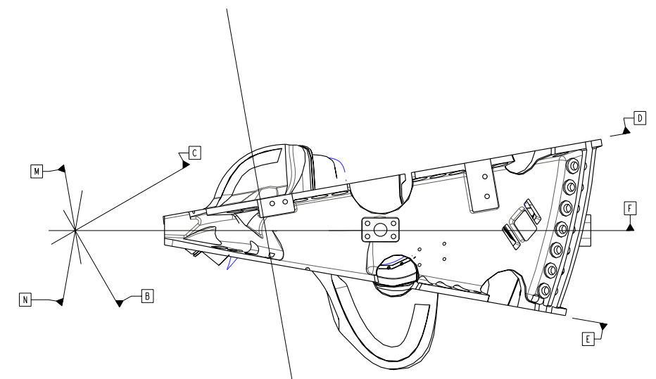
POLOIDAL BREAK DETAIL SCALE 0.13
