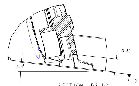
SECTION D3-D3 SCALE 0.19
