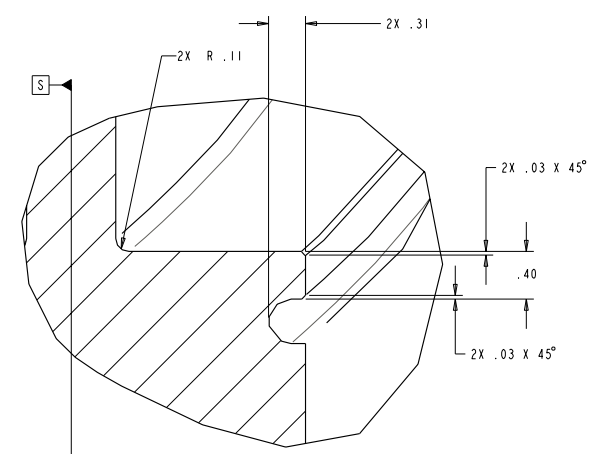
DETAIL B SCALE 2.00
