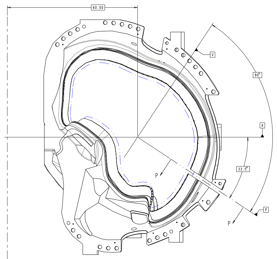
POLOIDAL BREAK DETAIL SCALE 0.13
