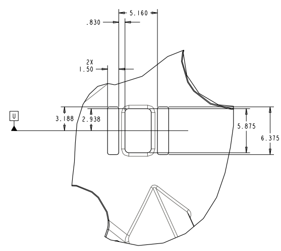
VIEW D4 - D4 SCALE 0.250
