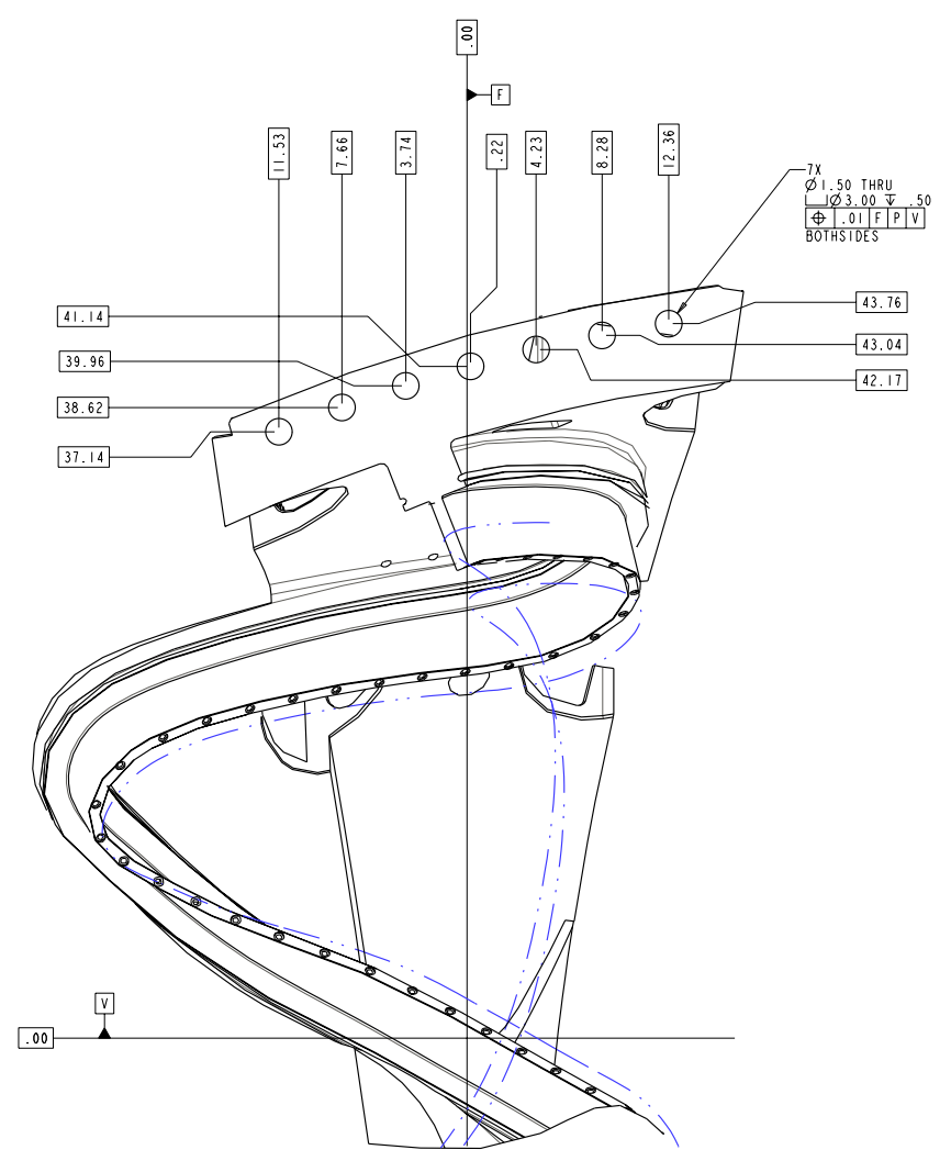
SECTION P-P SCALE 0.25
