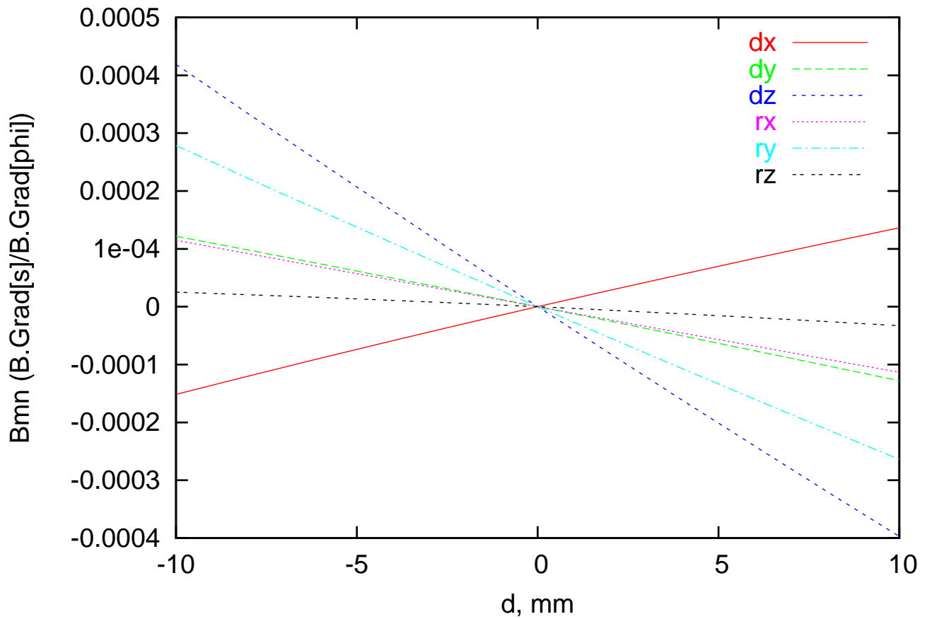
C2 m2n1 cos Resonant Field Error vs Displacement
