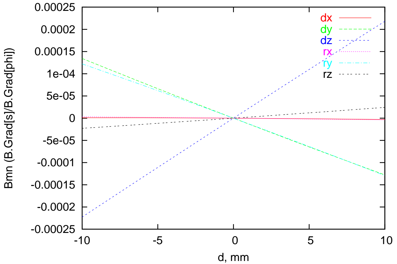
C4 m5n3 cos Resonant Field Error vs Displacement
