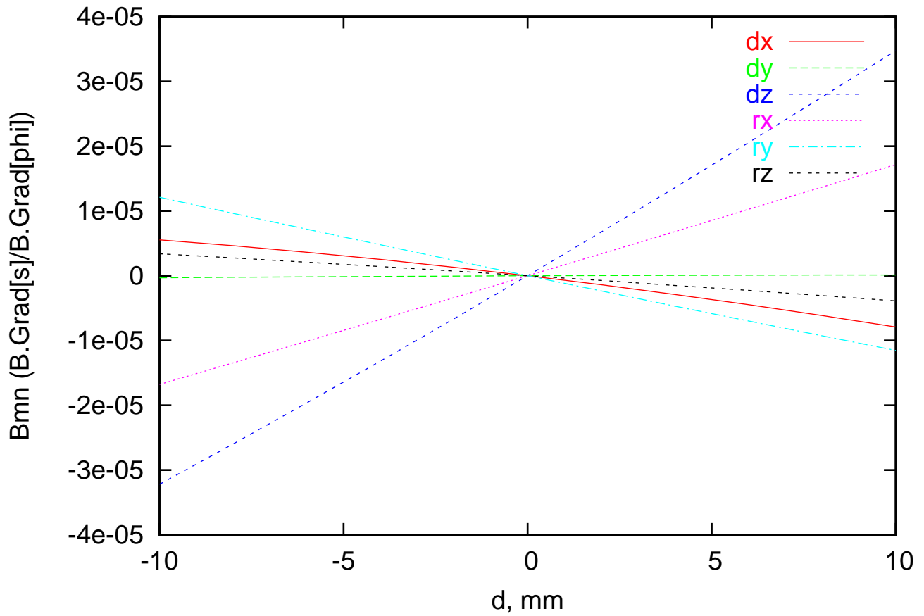
C4 m6n3 cos Resonant Field Error vs Displacement
