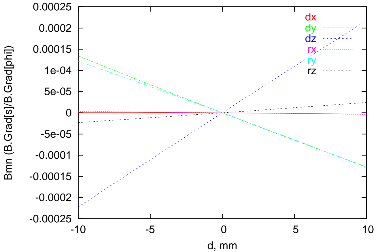
C2 m5n3 cos Resonant Field Error vs Displacement
