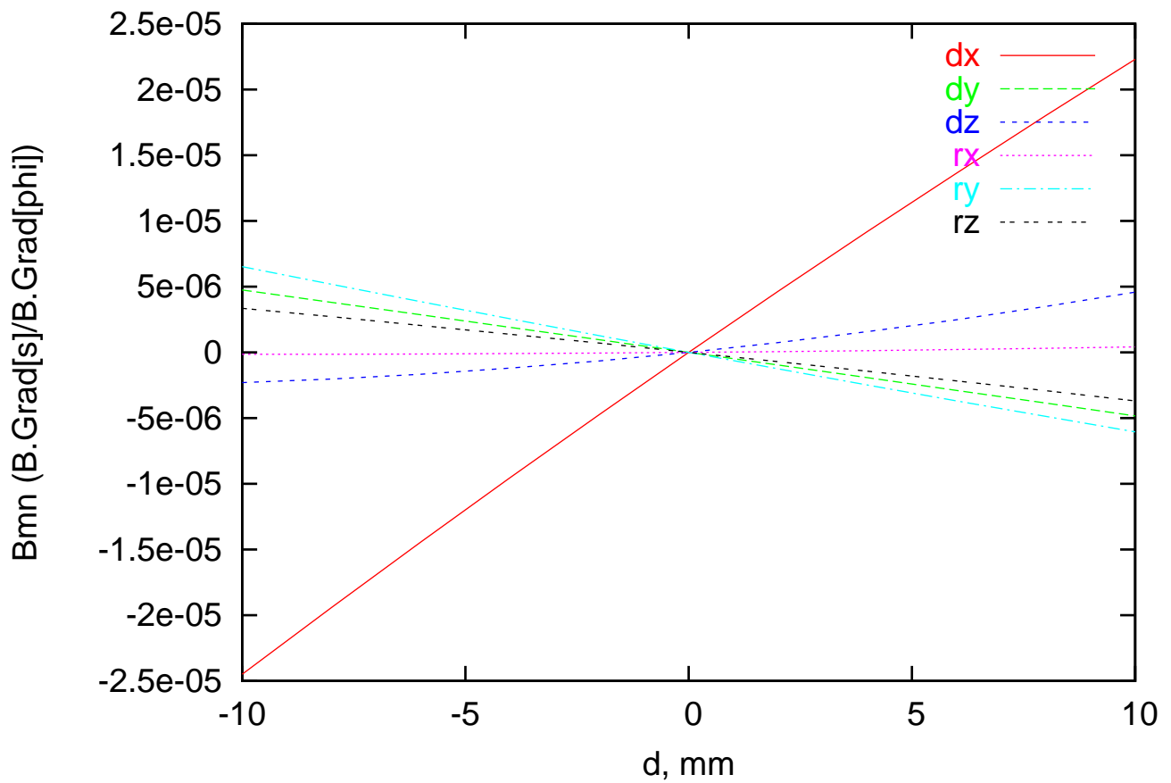
C3 m6n3 cos Resonant Field Error vs Displacement
