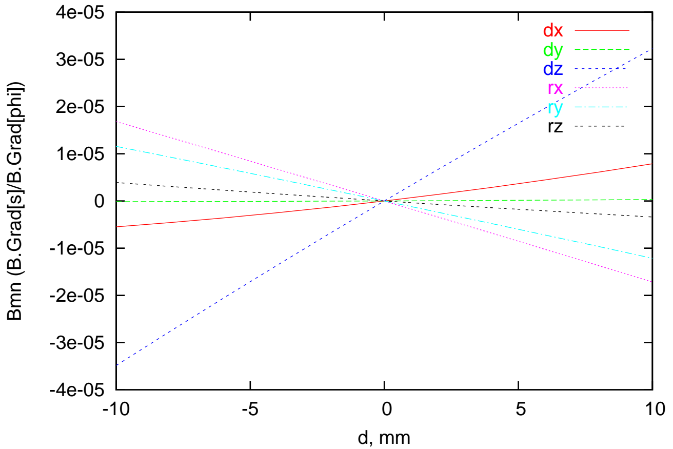
C1 m6n3 cos Resonant Field Error vs Displacement
