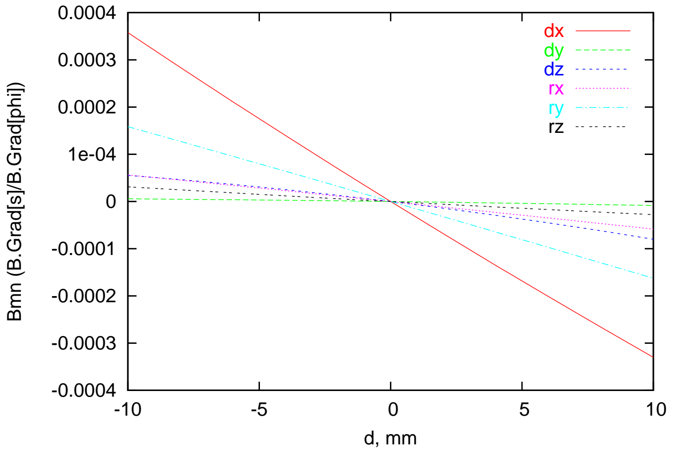
C1 m5n3 cos Resonant Field Error vs Displacement
