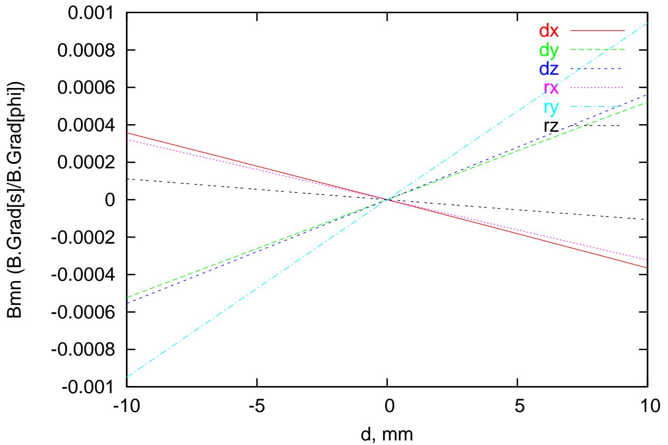
C4 m2n1 cos Resonant Field Error vs Displacement
