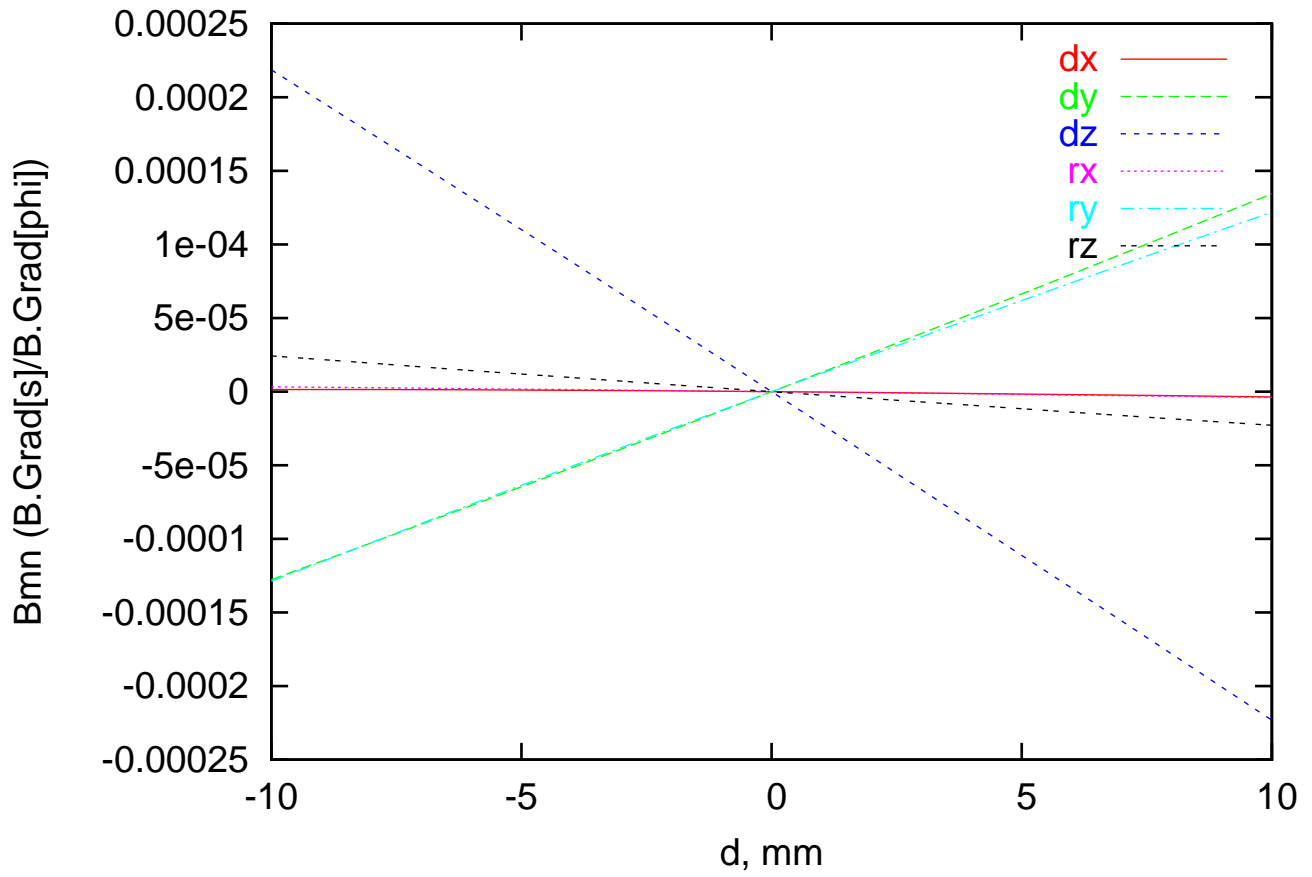
C3 m5n3 cos Resonant Field Error vs Displacement
