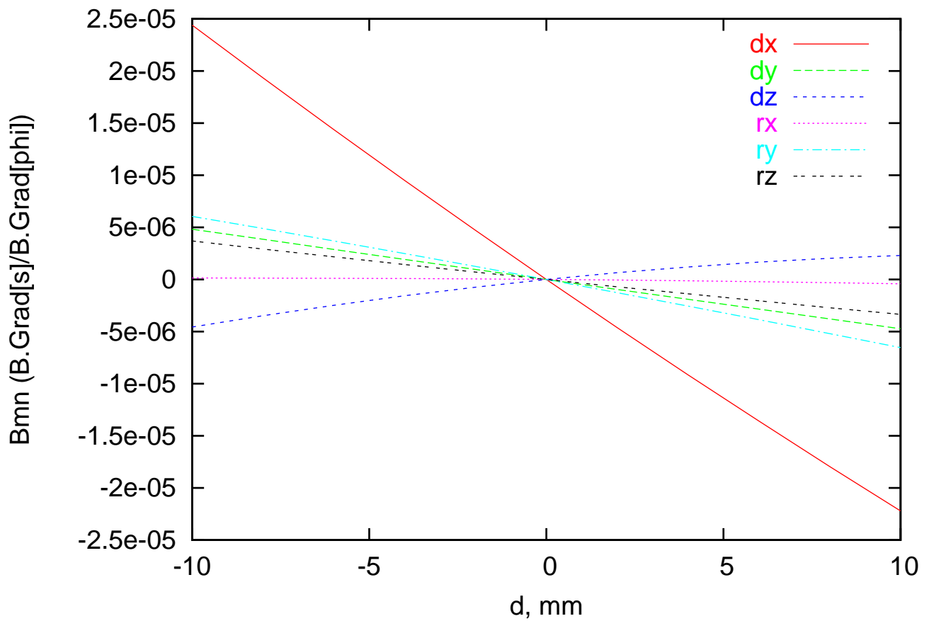
C2 m6n3 cos Resonant Field Error vs Displacement
