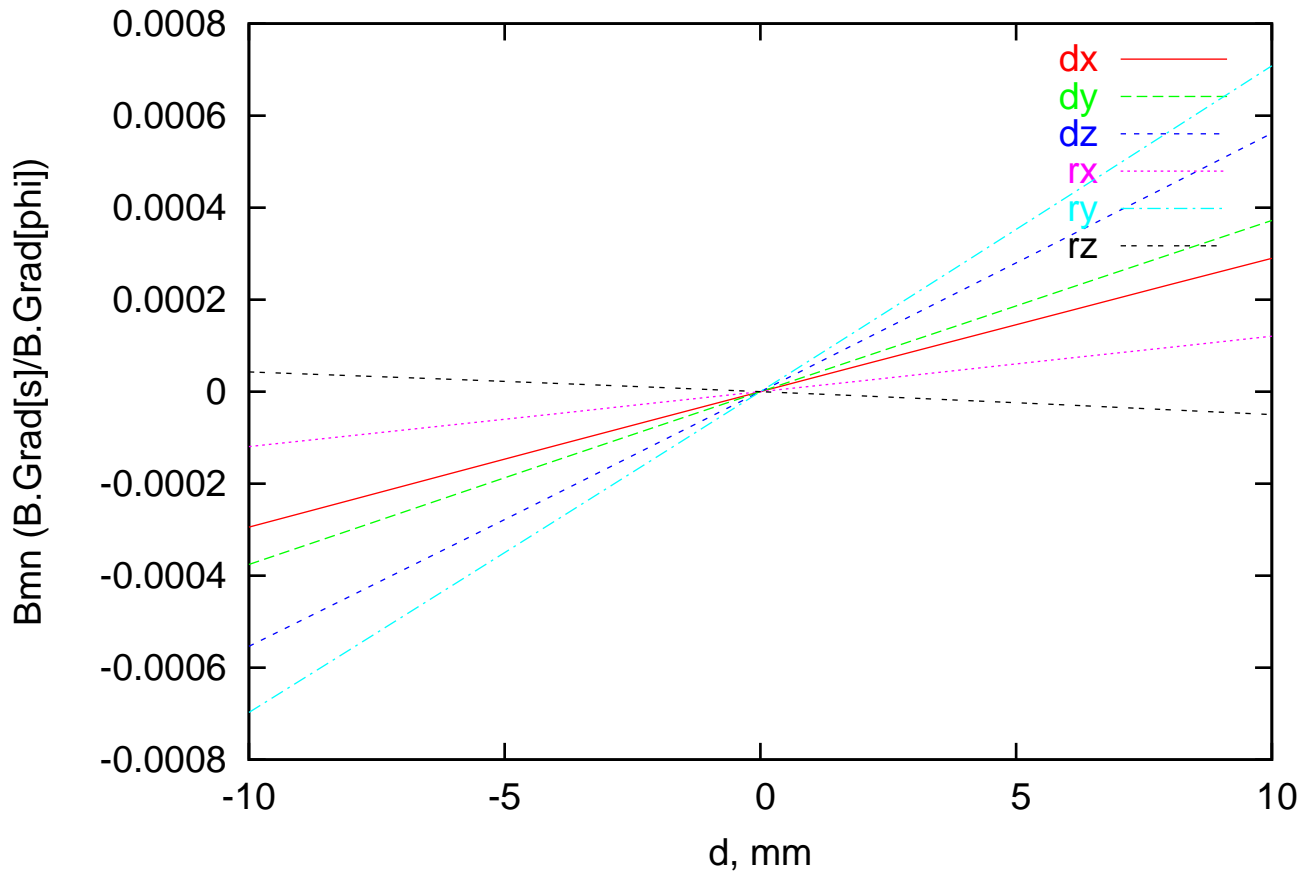
C3 m2n1 cos Resonant Field Error vs Displacement
