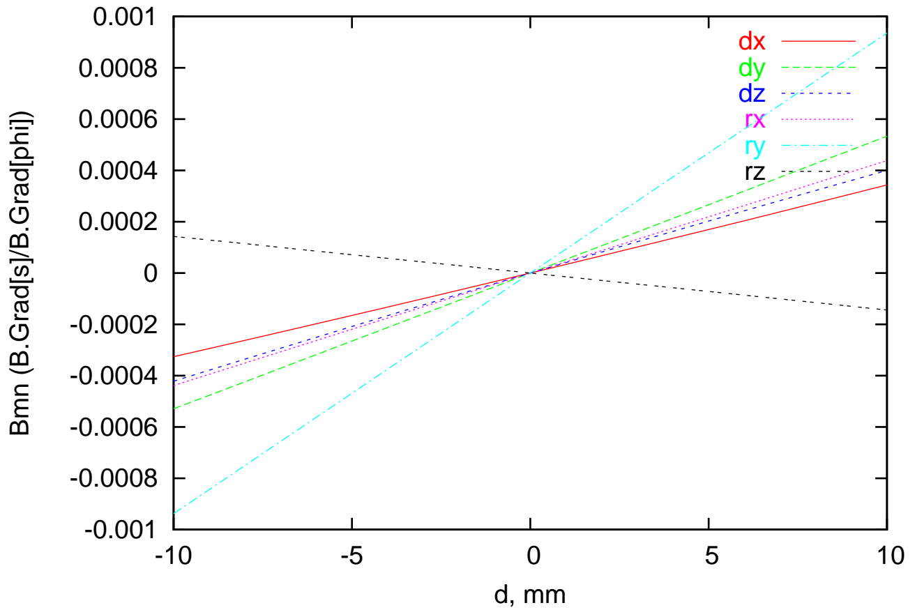
C1 m2n1 cos Resonant Field Error vs Displacement
