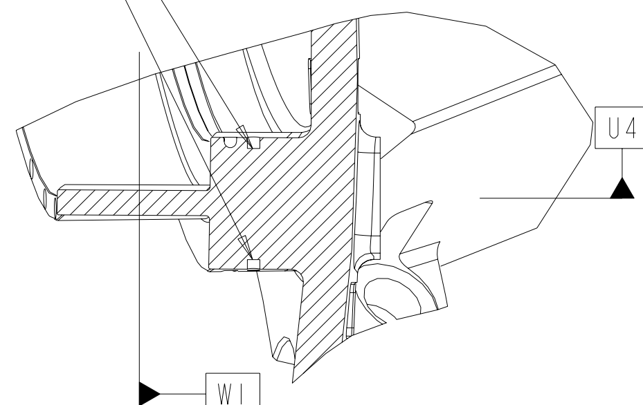
SECTION U2-U2 3 5
