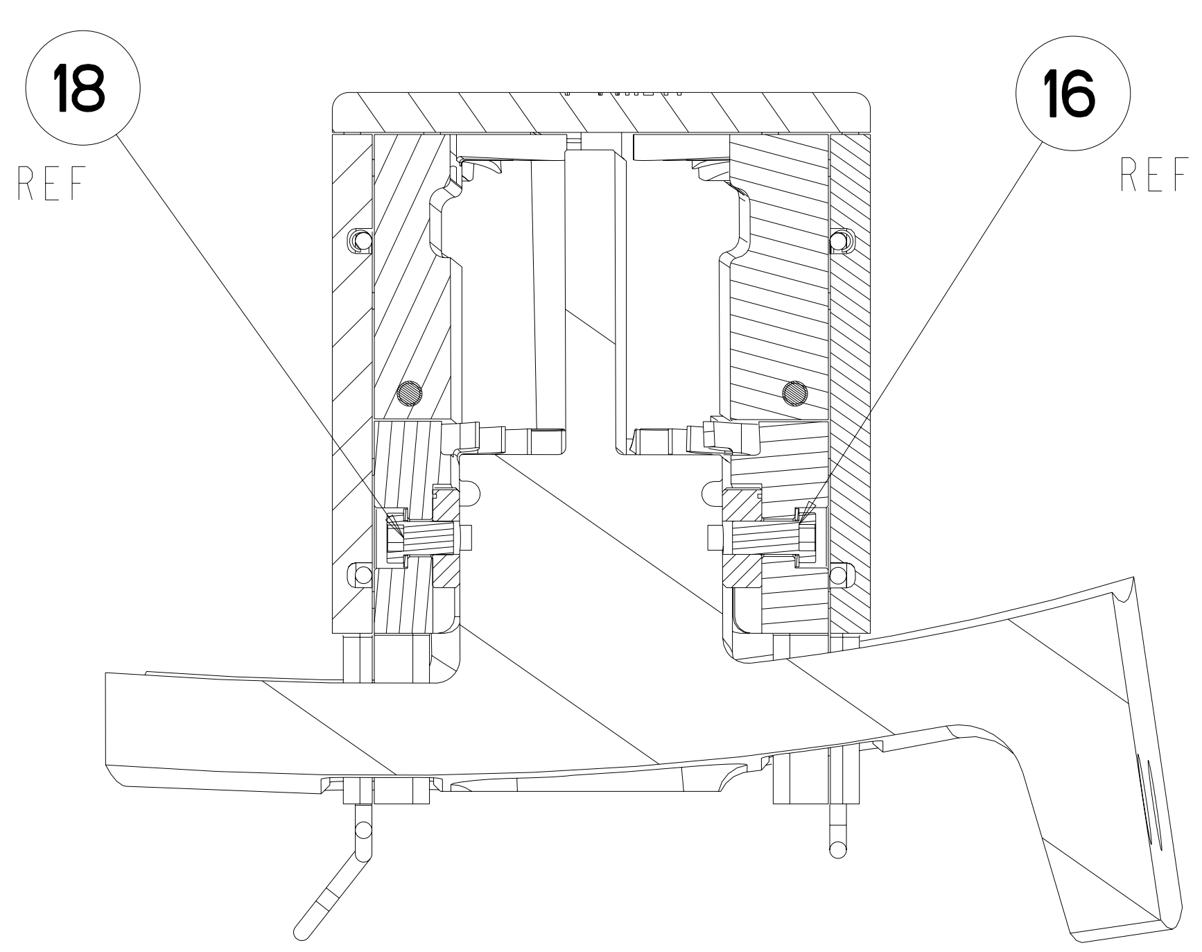
SECTION C-C
