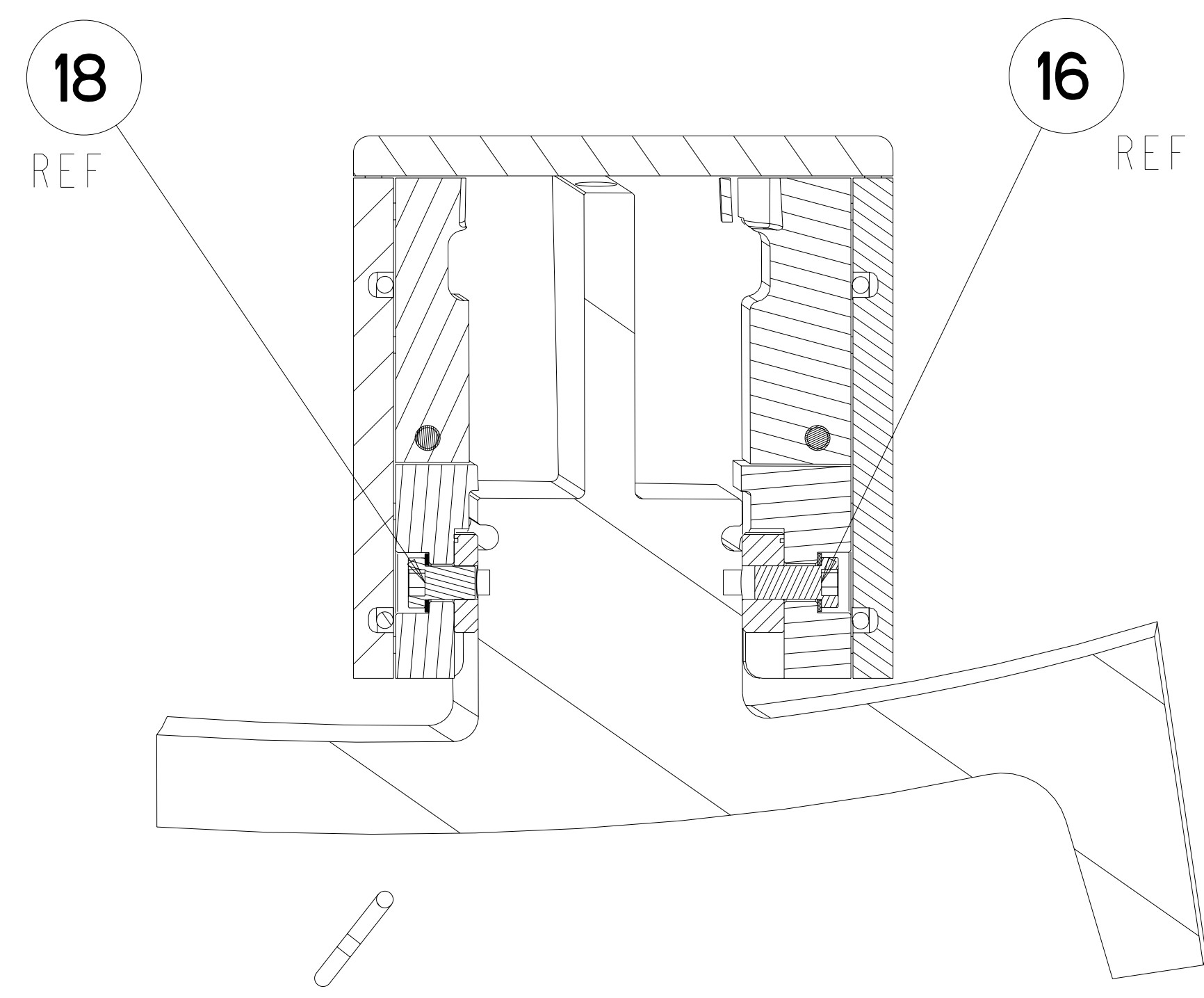
SECTION B-B
