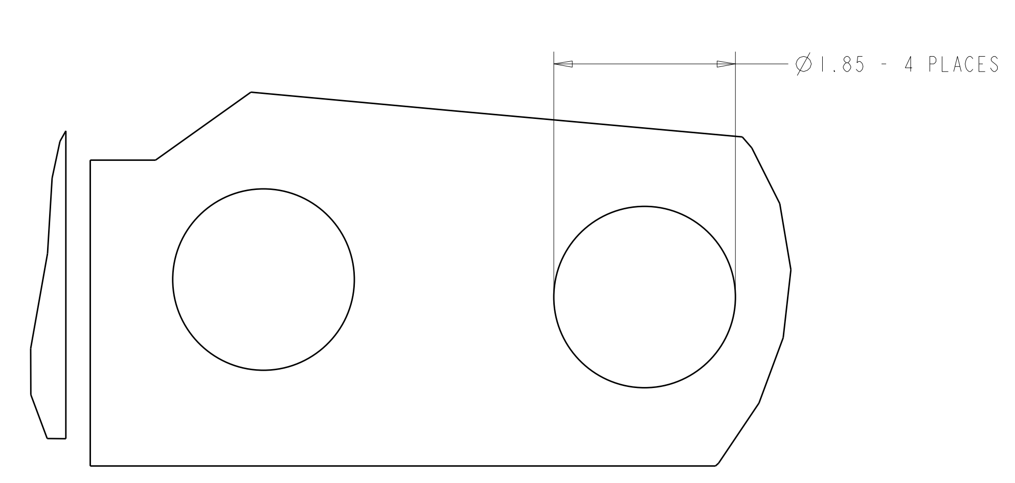
DETAIL A SCALE 1.000
