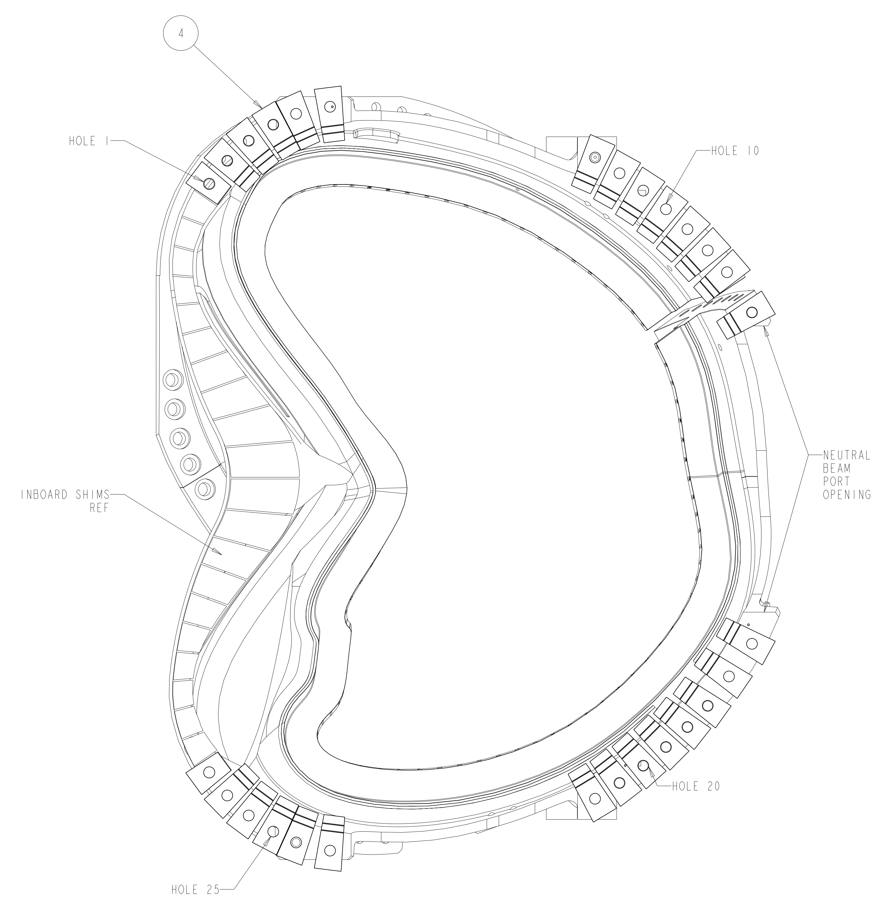
A-A FLANGE SHIMS SEE SE140-046 FOR WELDING SCALE 0.125
