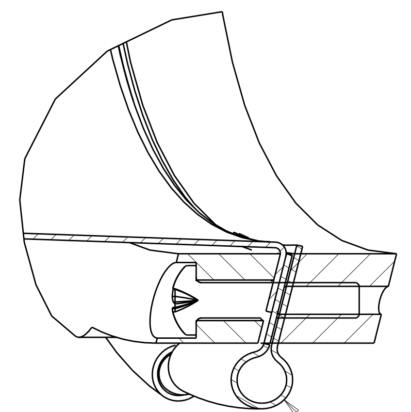
TYPICAL CLOTH HEM DETAIL FOR DRAWSTRING SCALE 2.00
