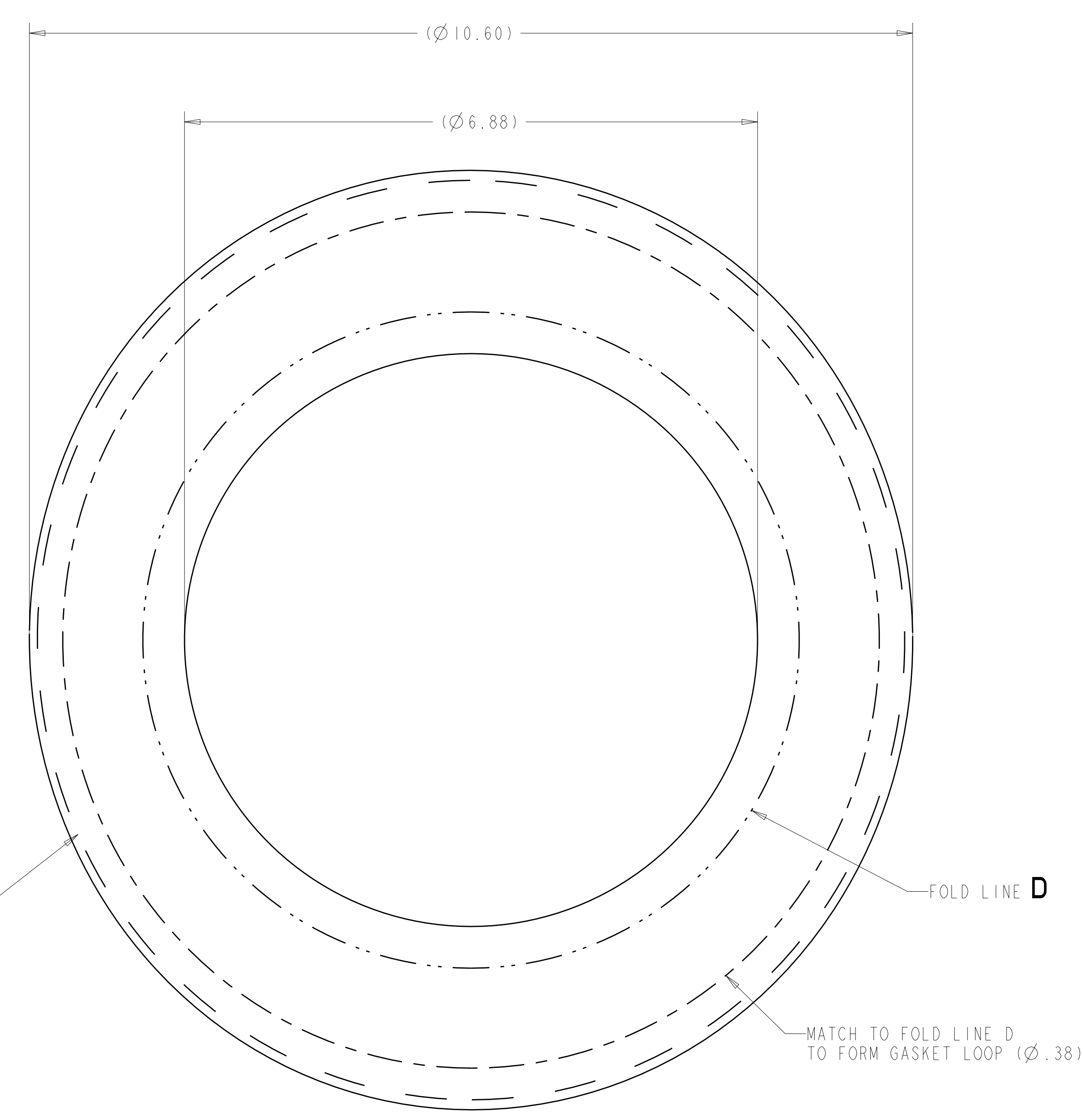
-3 FLAT PATTERN [4] SCALE 1.000
