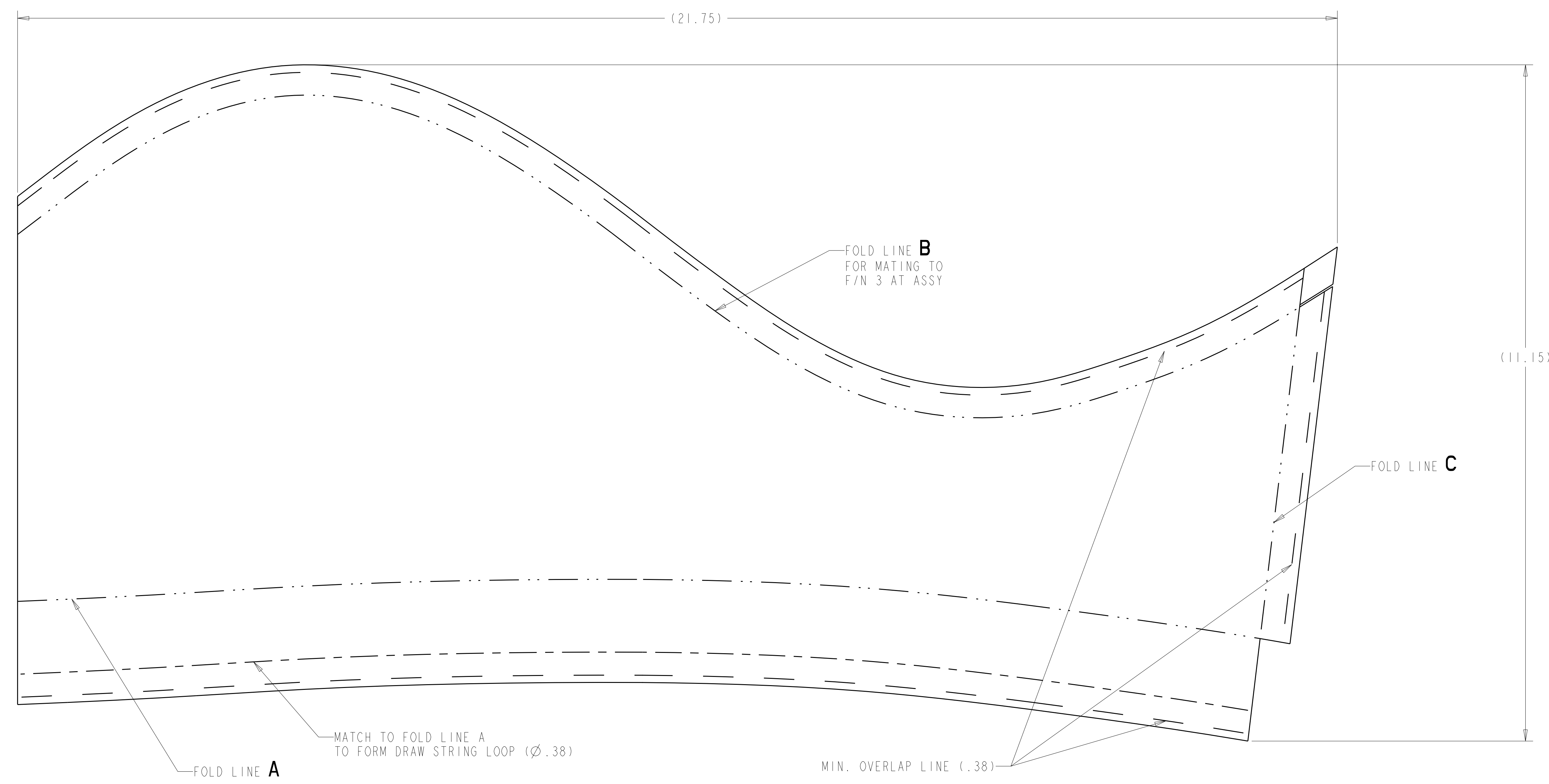
-2 FLAT PATTERN [4] SCALE 1.000
