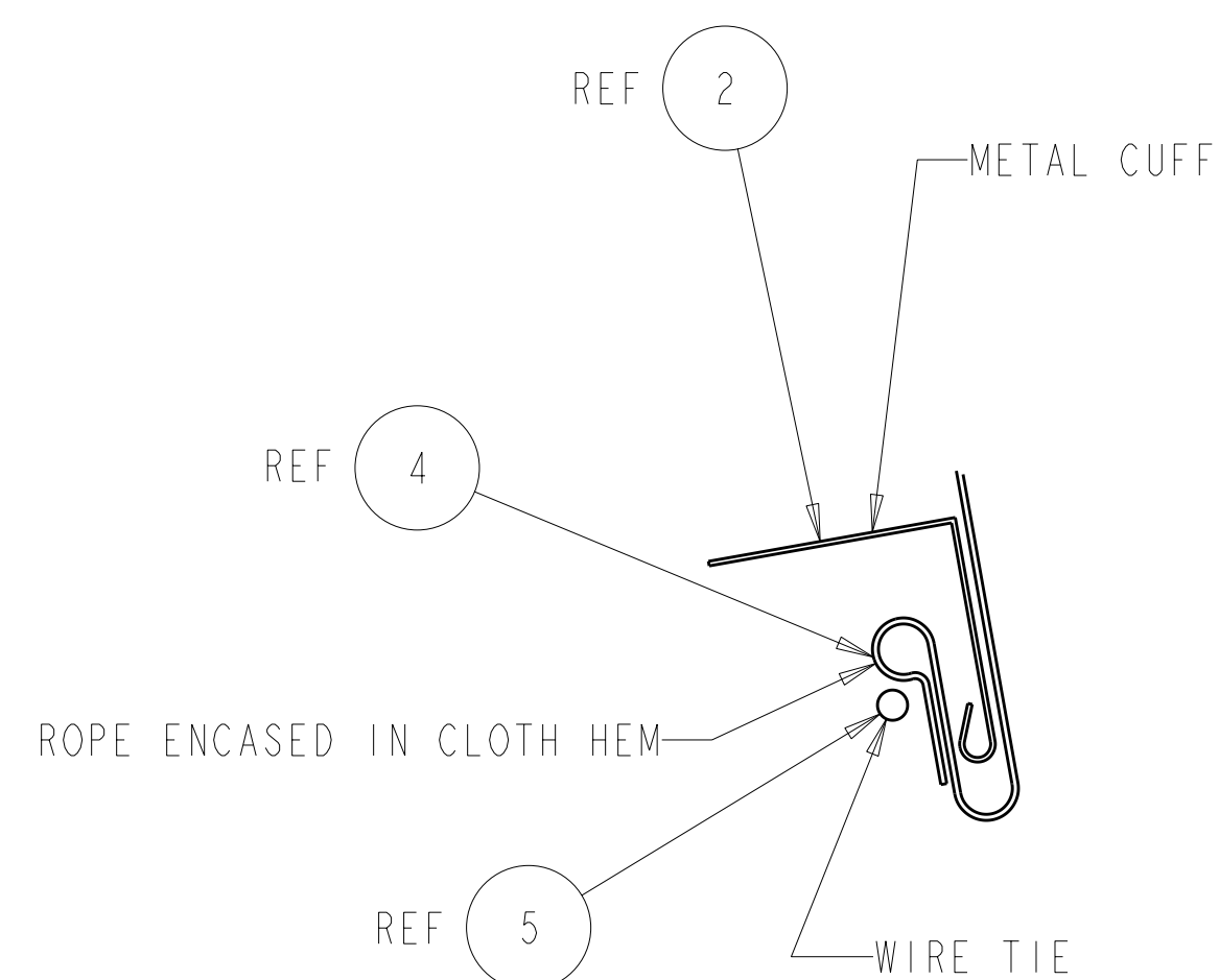
SECTION A-A SCALE 1.00
