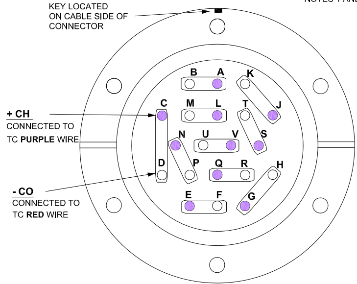
THERMOCOUPLE FEEDTHRU ( REAR VIEW - WIRE SIDE ) NOTES 1 AND 2
