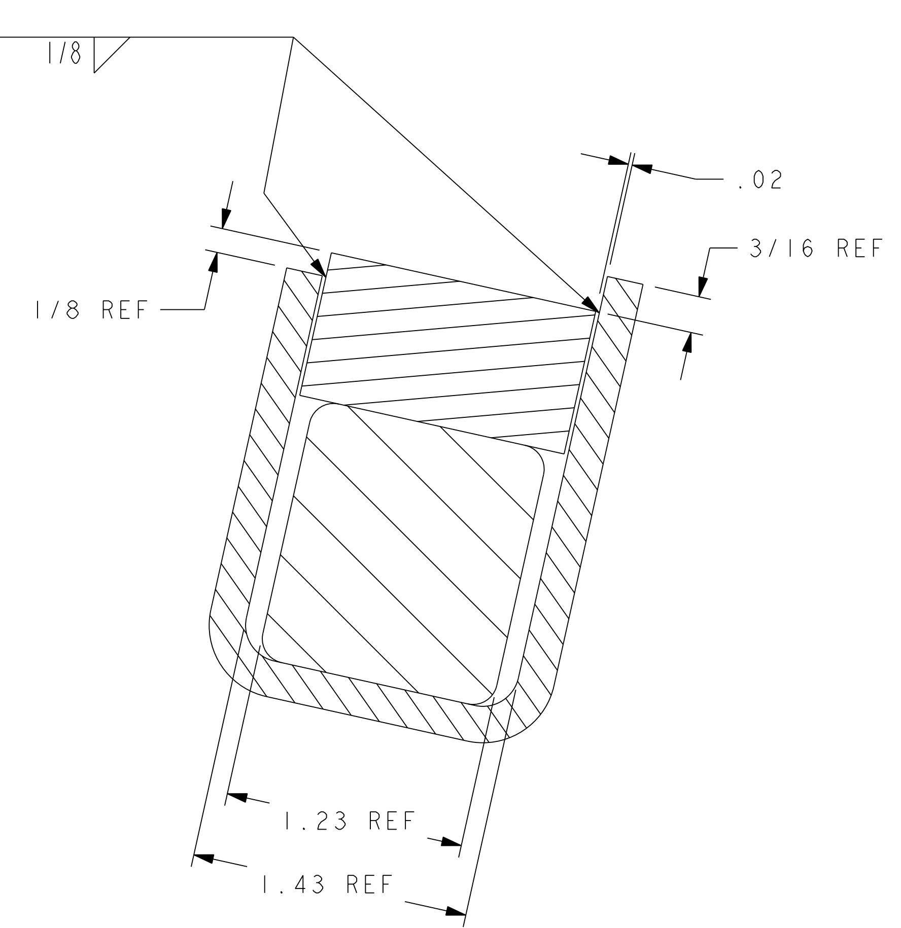
SECTION A - A SCALE 2
