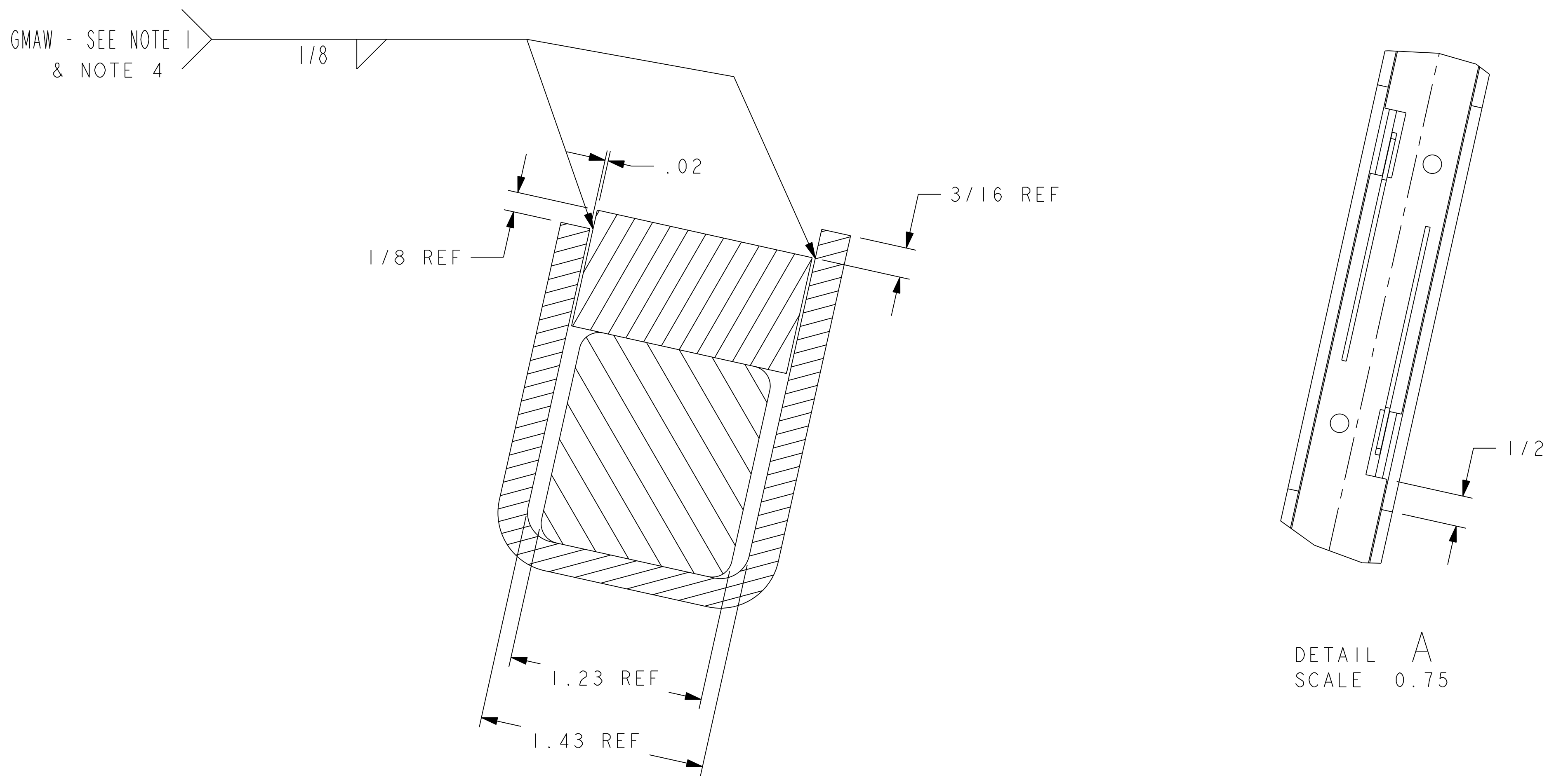
SECTION A - A SCALE 2
