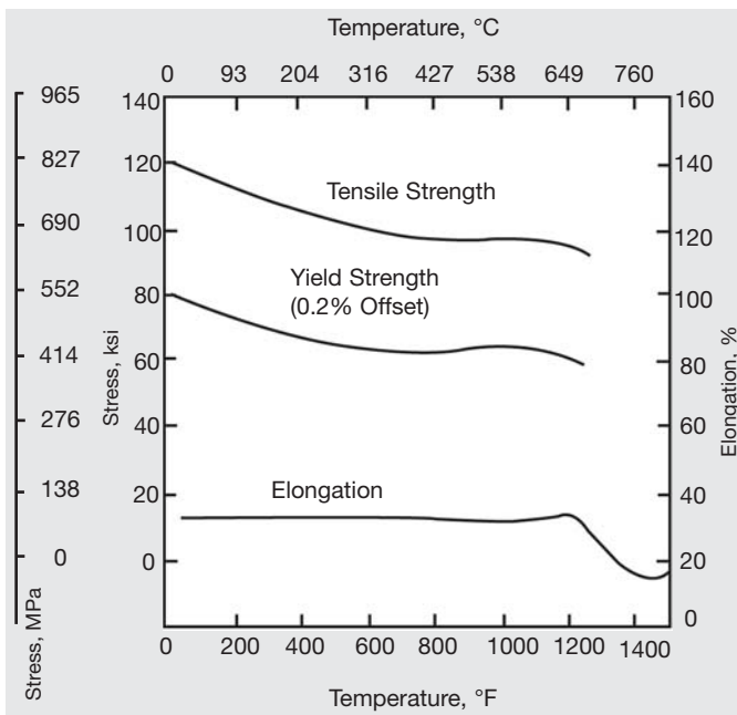
Figure 20. High-temperature tensile properties of of INCONEL alloy 625 all-weld metal (½-in. solution-treated plate; gas-tungsten-arc process with INCONEL Filler Metal 625).
