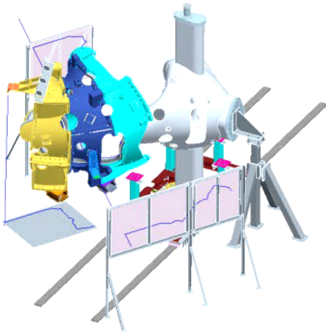
Station 3 assembly
