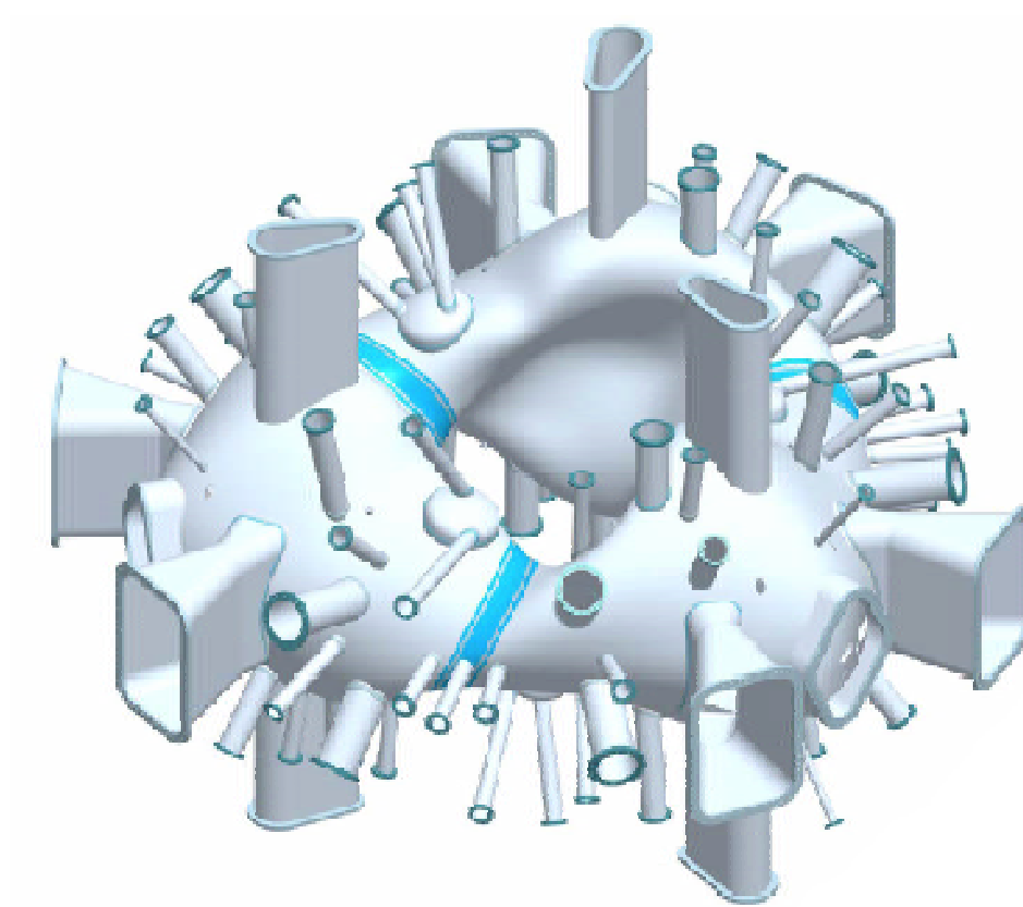
Figure 3: NCSX vacuum vessel design.
