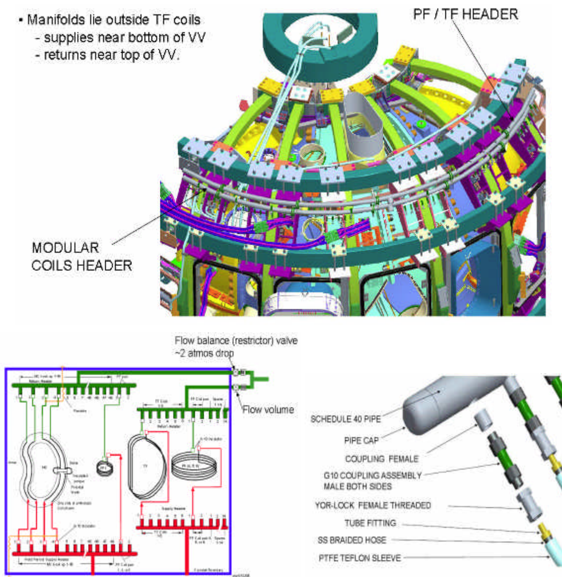
Figure 22: Schematics illustrating LN2 distribution.
