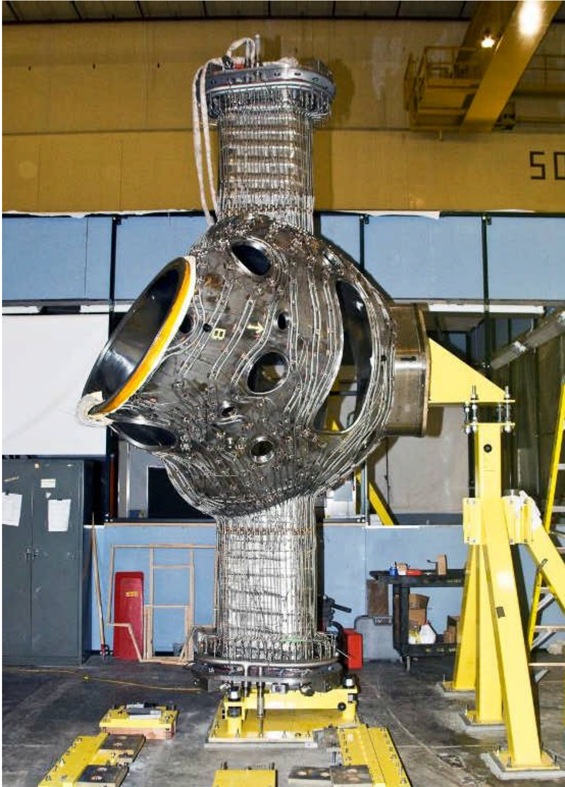
Figure 5: Vacuum vessel sub-assembly with cooling hoses and diagnostic instrumentation installed.
