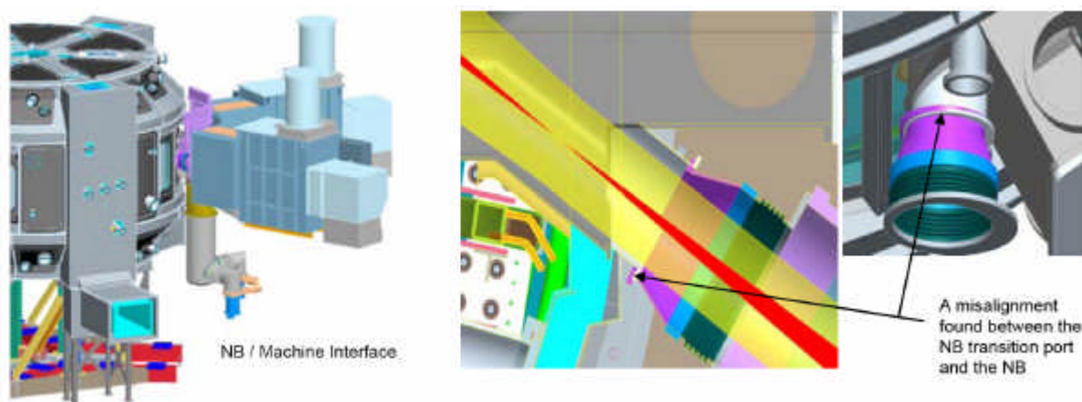
Figure 30: Neutral beam interface schematic.
