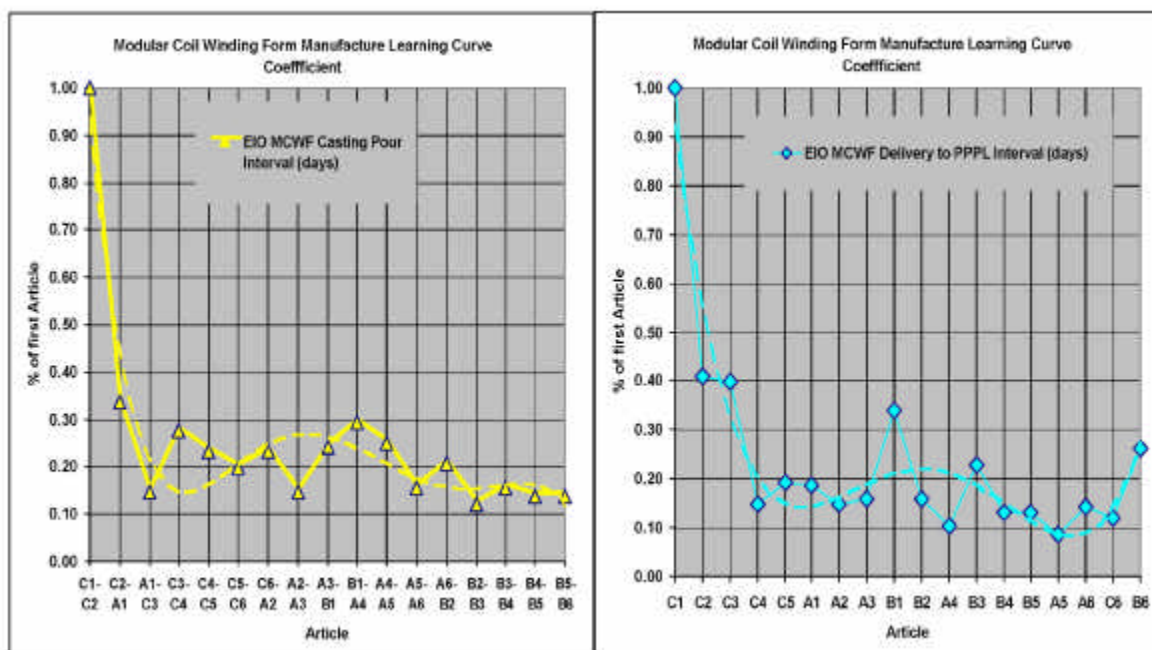
Figure 18: Learning curve for manufacture of MCWF: (1) time intervals between castings normalized to the interval between the first and second article; and (2) time intervals between MCWF deliveries normalized to the time between receipt of the first article casting and delivery of the machined first article to PPPL.
