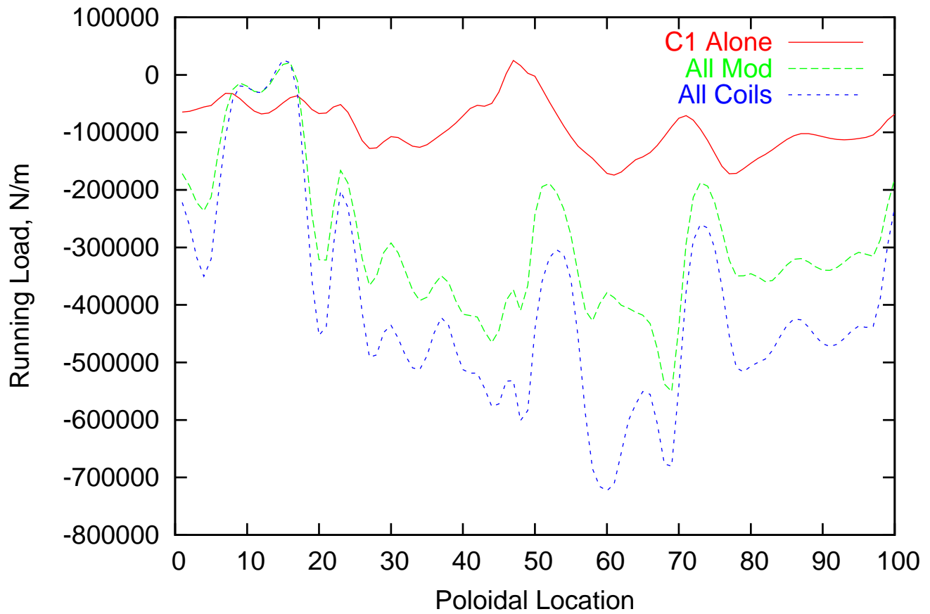
C1 Side B Radial EM Loads at 2T Currents
