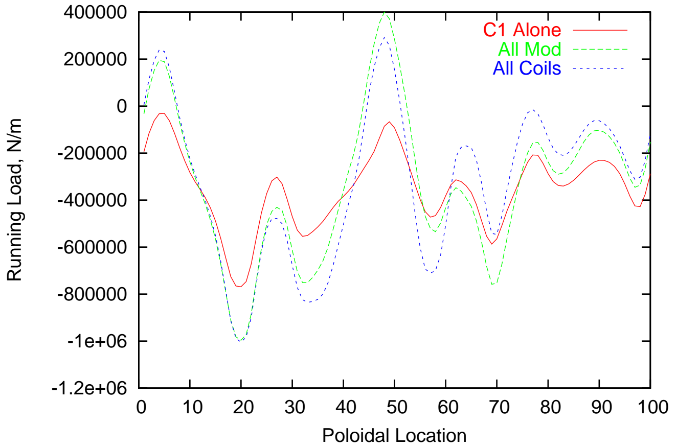
C1 Side B Lateral EM Loads at 2T Currents
