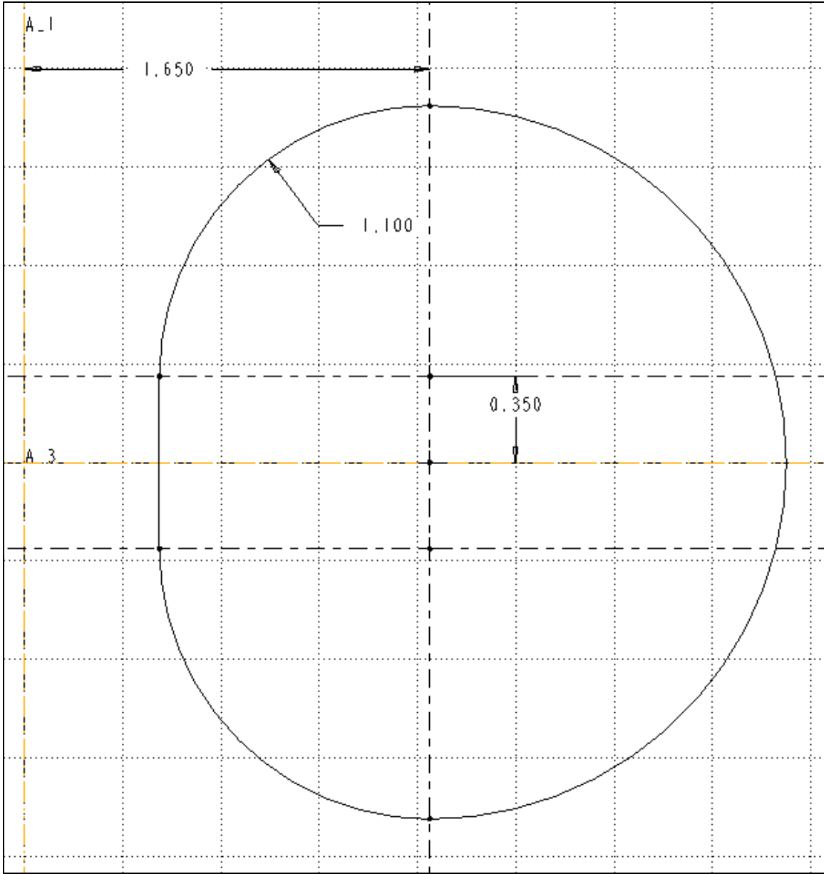
Fig. 1 – TF Coil Dimensions (m) for Case 1017
