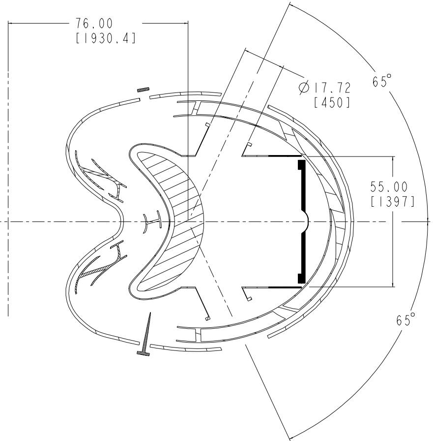
SECTION M-M
