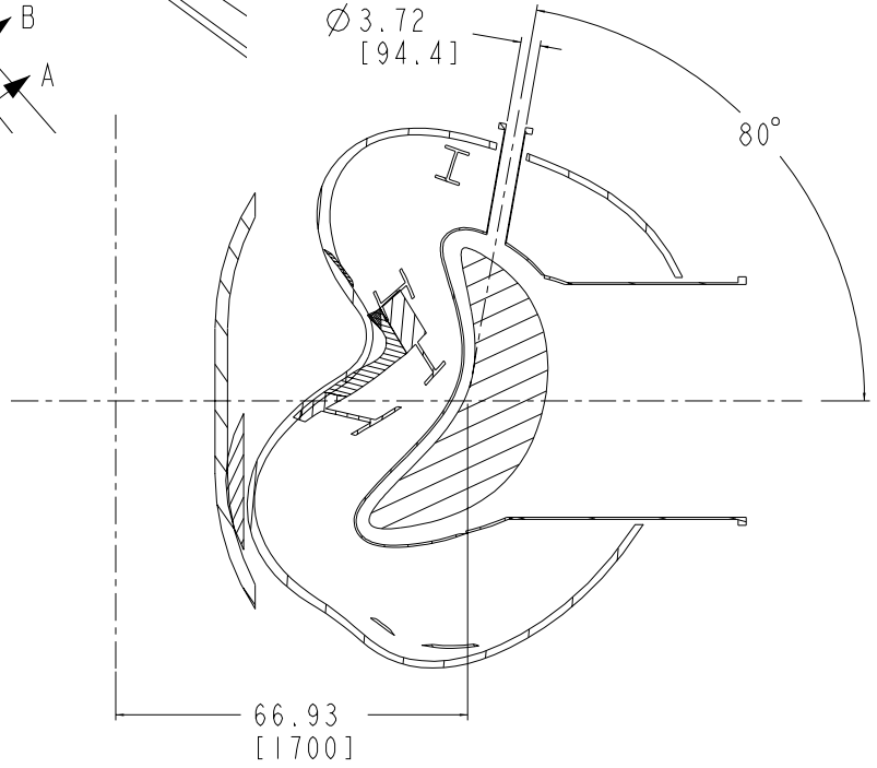
SECTION H-H
