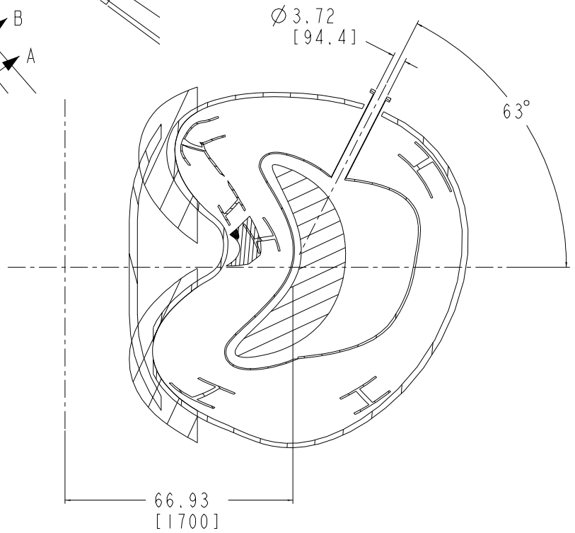
SECTION K-K
