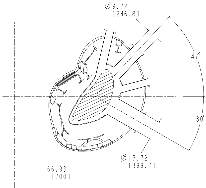
SECTION E-E
