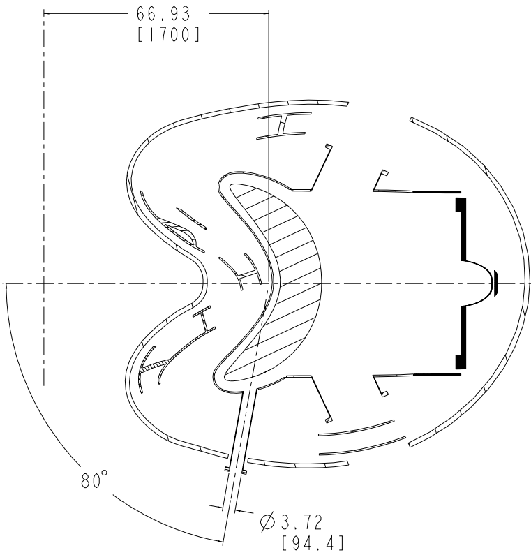
SECTION L-L
