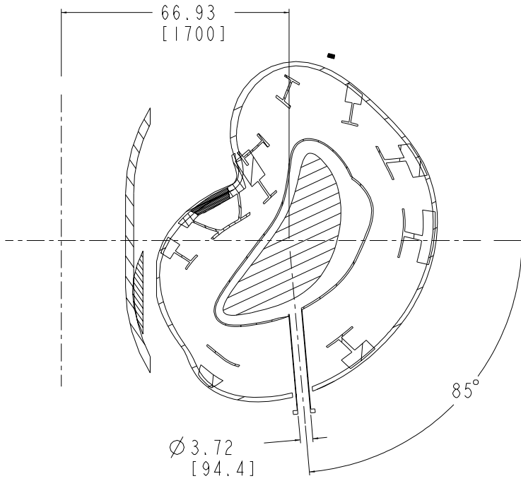
SECTION G-G
