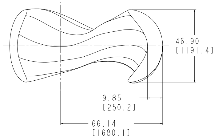
NCSX 1.36 m radius
