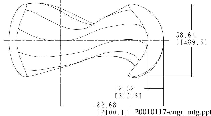
NCSX 1.7 m radius
