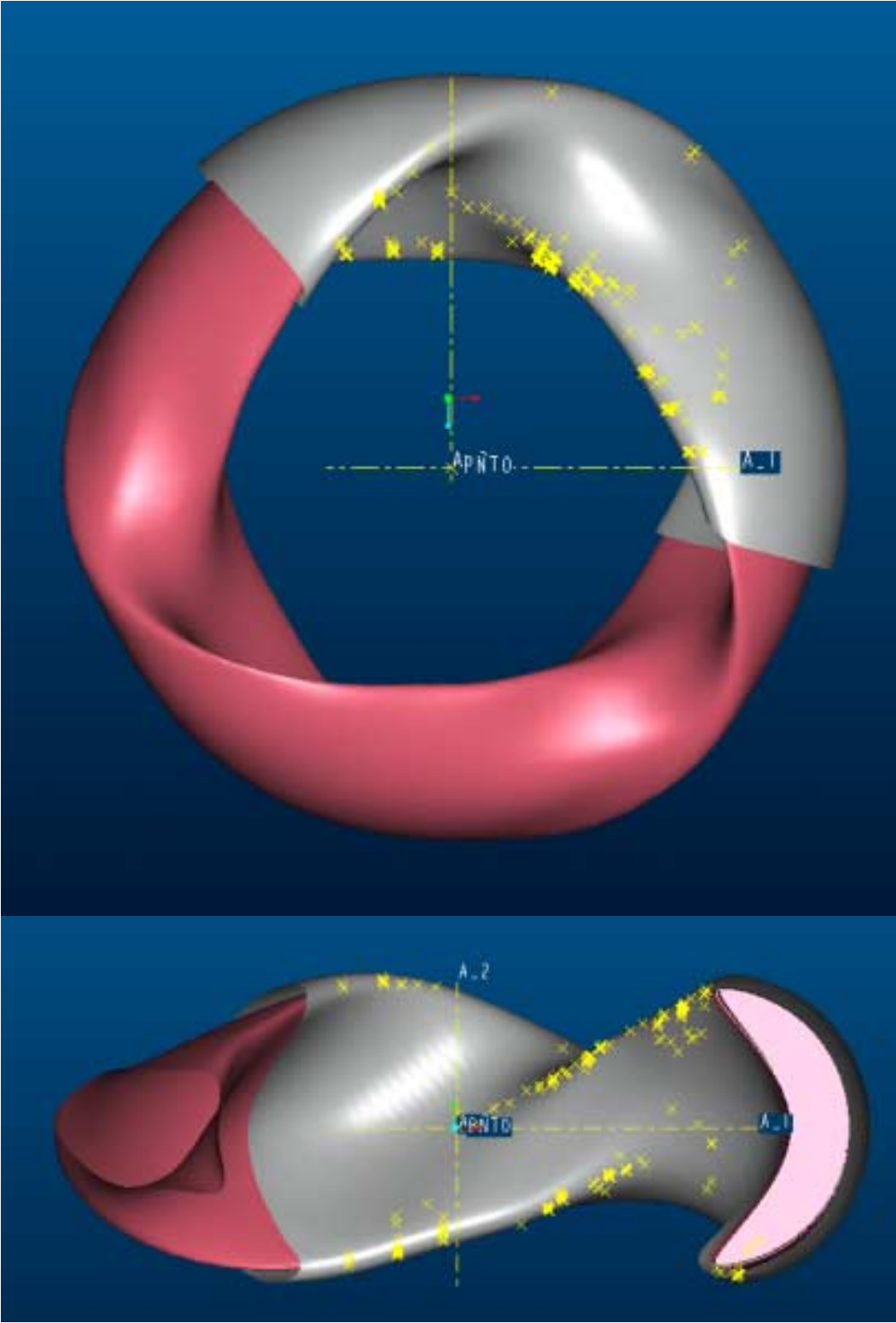
~300 strike points, shown on baseline NCSX first wall surface Sep 4, 2001 data from Maxim Umansky, scaled from 1.7 m by 0.82 factor
