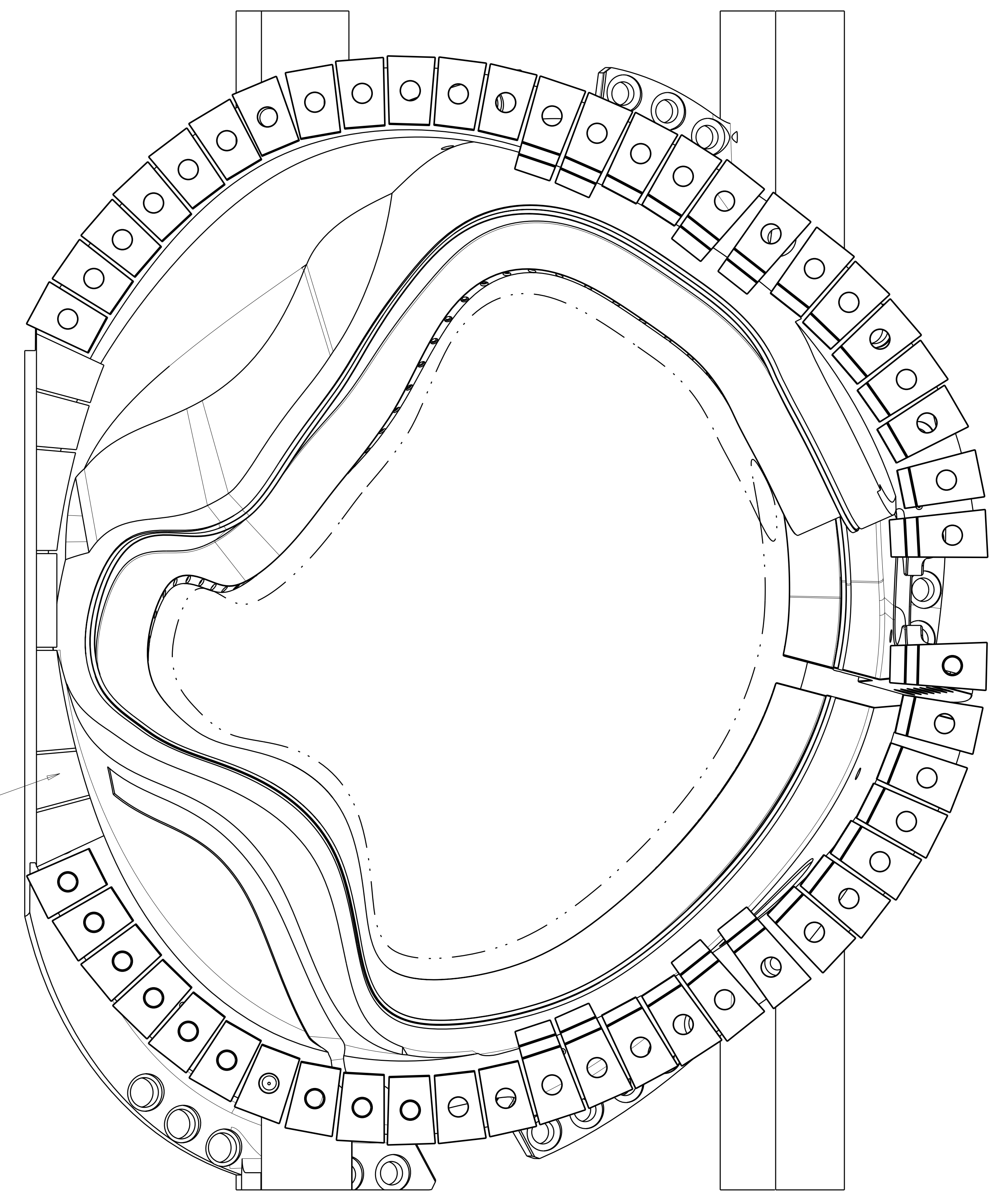
C-C SHIMS LOOKING AT THE C COIL FLANGE
