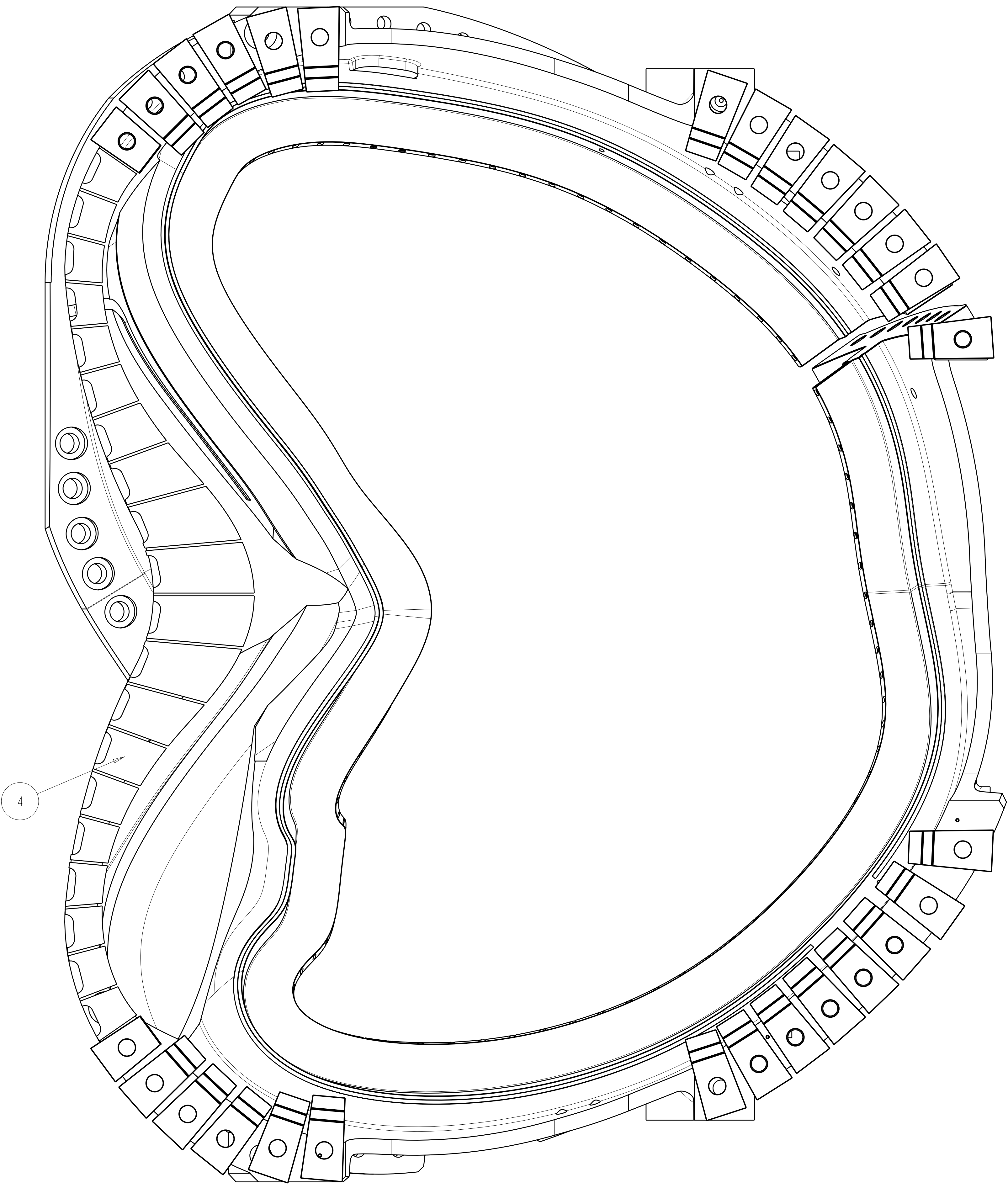
A-A SHIMS LOOKING AT THE A COIL FLANGE
